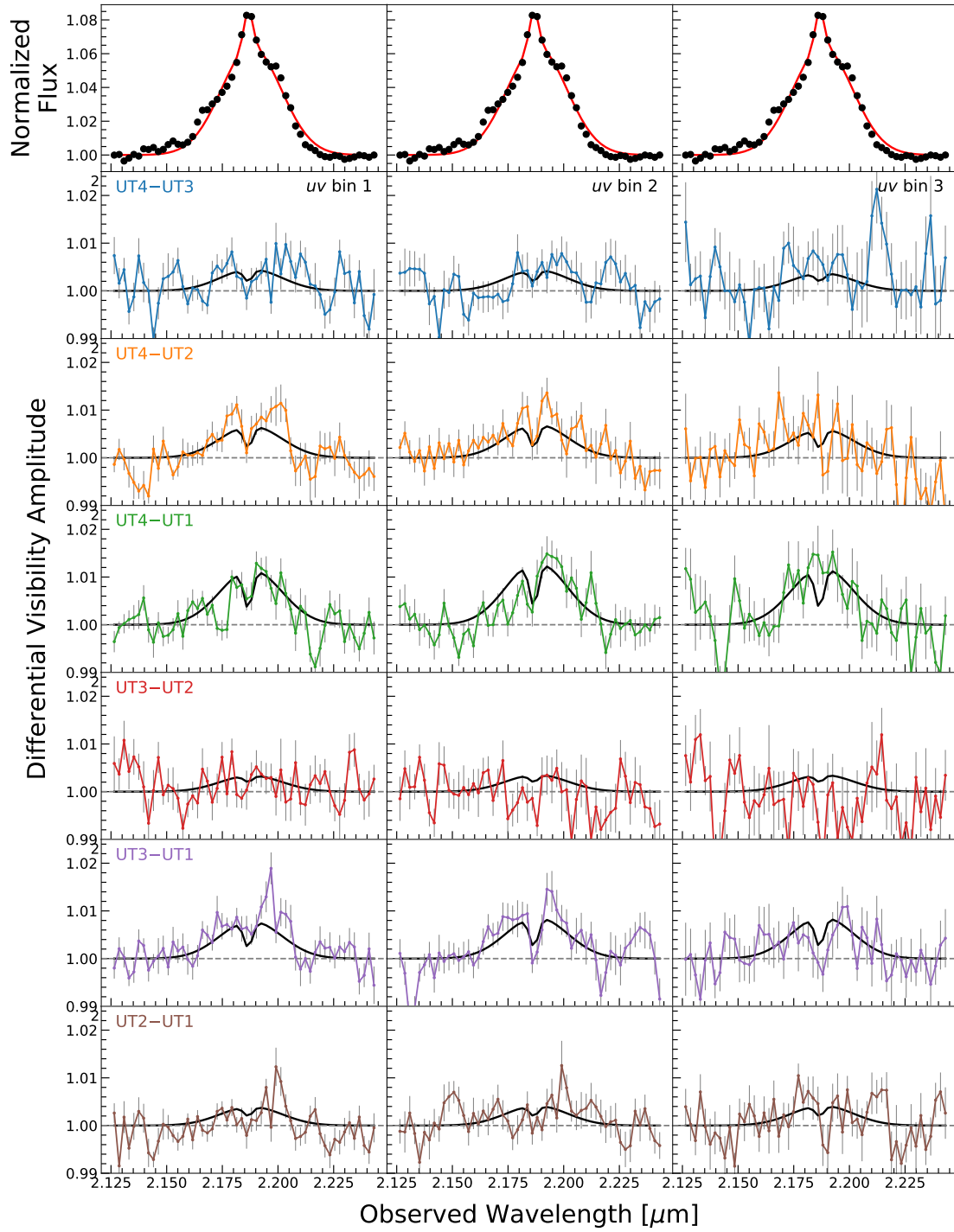
Fig. A.3: top row : Normalized GRAVITY Br \gamma profile (black points) with best fit model line profile (red line) from our coronal line region analysis. bottom rows : uv-binned differential visibility amplitude spectra for each baseline (coloured points and lines) with the best fit CLR model (solid lines).
