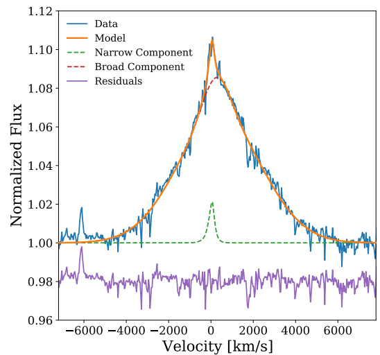
Fig. 4: Normalized Br \gamma profile from SINFONI (blue) with the best fit line profile model (orange). The model is the combination of a narrow line template determined by the [O III] \lambda 5007\text{\AA} line from X-Shooter spectra (green) and a broad component consisting of 2 Gaussians (red). The residuals (purple) show that our fit very well matches the observed Br \gamma profile.
