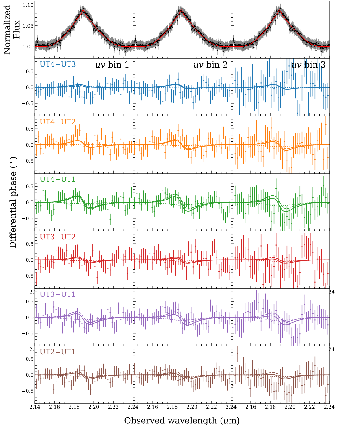
Fig. A.1: top row : Normalized Br \gamma profile (black points) with best fit model line profile (red line). bottom rows : uv-binned, continuum phase subtracted differential phase spectra for each baseline (coloured points) with the best fit BLR model spectra (solid lines). Model spectra for the BLR component are shown as dashed lines while the offset component is shown as dotted lines.
