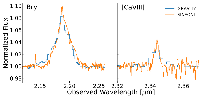
Fig. 3: The normalised Br \gamma and [Ca VIII] line profiles observed by GRAVITY (blue) and SINFONI (orange).
