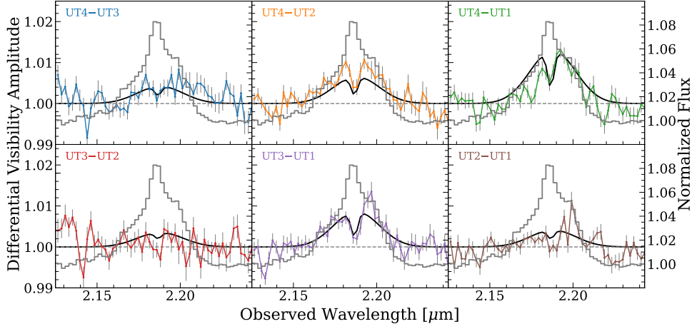
Fig. 5: Baseline averaged differential visibility amplitude spectra spanning the Br \gamma line (coloured points and grey error bars). The grey profile in each panel plots the same normalised Br \gamma spectrum from GRAVITY. The black curves represent the best fit model from our CLR analysis in Sec. 5.
