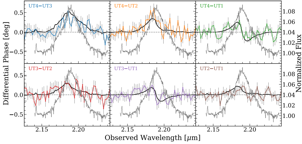
Fig. 6: Baseline averaged differential phase spectra spanning the Br \gamma line (coloured points and grey error bars). The grey profile in each panel plots the same normalised Br \gamma spectrum from SINFONI with the narrow component removed. The black curves represent the best fit BLR model summed with the continuum phase calculated from our image reconstruction. The model line profile looks noisy due to the continuum phase contribution being calculated based on the observed line profile.
