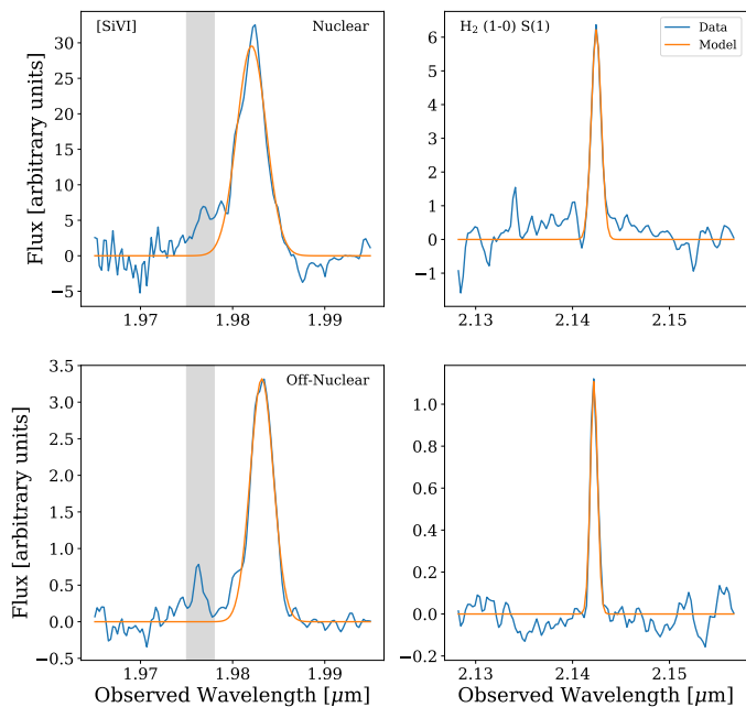
Fig. 17: Example fits to individual spectra for the [Si VI] (left panels) and H_2 (1–0) S(1) (right panels). The observed spectra are shown in blue while the best fit Gaussian models are shown in orange. The top row shows the spectral regions from a nuclear pixel while the bottom row shows the spectral regions from an off-nuclear pixel. The specific pixels used are shown as white crosses in Fig. 16. The grey shaded region in the [Si VI] panels show the masked region corresponding to the expected location of the H_2 (1–0) S(3).
