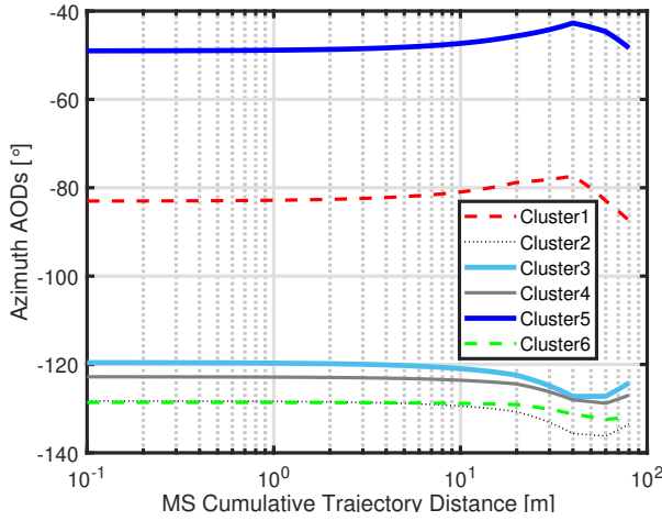
Fig. 12. Spatially consistent azimuth AODs vs. cumulative distance of MS trajectory.
