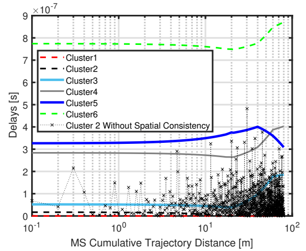
Fig. 11. Cluster delays with and without spatial consistency vs. cumulative distance of MS trajectory.
