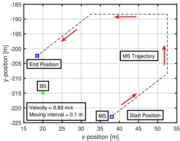
Fig. 10. Investigated scenario where the MS communicates with the BS while moving along a trajectory shown by red arrows with a predefined velocity and moving interval.
