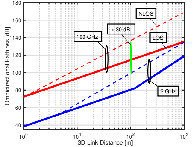
Fig. 1. 3GPP TR 38.901 standardized pathloss model for the 3D UMa LOS and NLOS scenarios across 2 GHz and 100 GHz. The NLOS cases at both frequencies are depicted in dashed line, while the solid lines are used to denote LOS cases. For further information, see [38].
