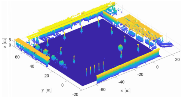
Fig. 7. A sample point cloud of an open square. Points are colored according to their heights above the ground.
