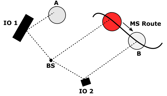
Fig. 5. Example of visibility areas (gray circles) and IO positions (black rectangles). The red circle is the local scattering cluster, which moves with the MS. Along the particular MS trajectory shown, only one of the two clusters (B) will be activated.
