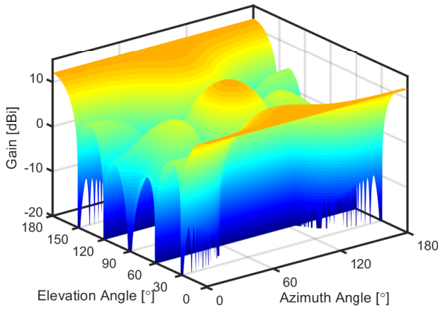
Fig. 4. Directional antenna gain of a 16 element (2 (rows) \times 4 (columns) \times 2 (polarizations)) planar array with identical parameters as Fig. 3.
