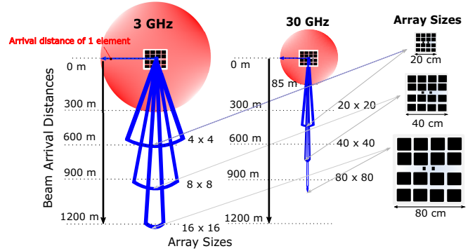
Fig. 2. Demonstration of beamforming effects (in terms of beam arrival distances) relative to operating frequency and array sizes.
