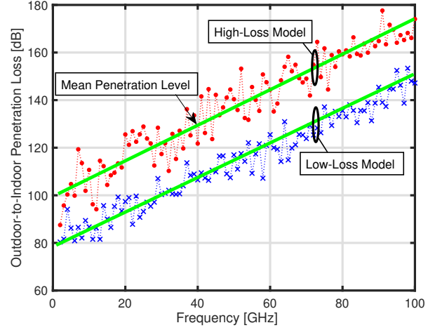
Fig. 9. 3GPP TR 38.901 quoted outdoor-to-indoor penetration loss model as a function of the carrier frequency for an UMi scenario with a 3D link distance of 25 m. Both the low-loss and high-loss models are depicted with the mean penetration levels with varying frequency.
