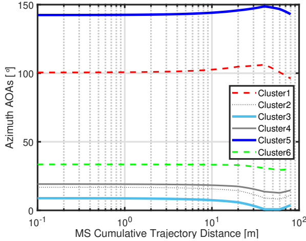
Fig. 13. Spatially consistent azimuth AOAs vs. cumulative distance of MS trajectory.
