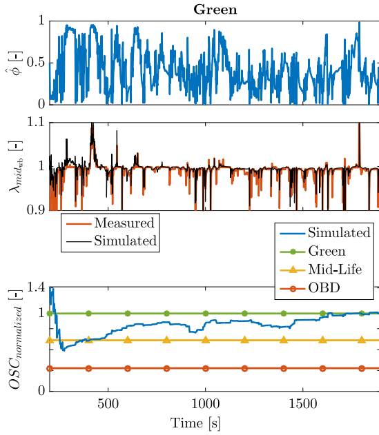
Fig. 9. Simulation results of the estimated and measured \lambda_{mid_{ab}} , \hat{\phi} is the average value of oxygen level from all the three spatially discretized cells and \widehat{OSC} is the estimate of oxygen storage capacity (normalized with respect to the OSC of a fresh catalyst) for the Green catalyst.
