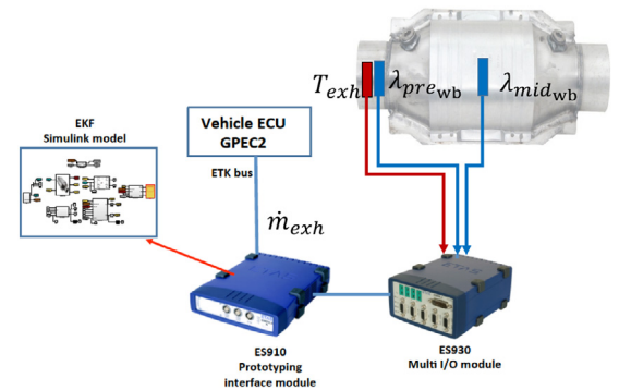
Fig. 15. Rapid test prototyping setup.
