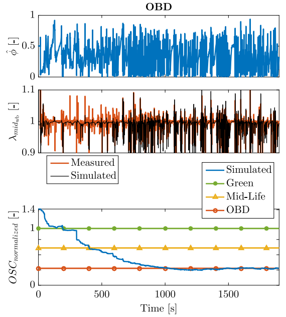
Fig. 11. Simulation results of the estimated and measured \lambda_{mid_{ab}} , \hat{\phi} is the average value of oxygen level from all the three spatial discretization cells and \widehat{OSC} is the estimate of oxygen storage capacity (normalized with respect to the OSC of a fresh catalyst) for the OBD catalyst.
