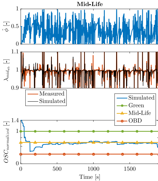
Fig. 10. Simulation results of the estimated and measured \lambda_{mid_{ab}} , \hat{\phi} is the average value of oxygen level from all the three spatially discretized cells and \widehat{OSC} is the estimate of oxygen storage capacity (normalized with respect to the OSC of a fresh catalyst) for the Mid-Life catalyst.
