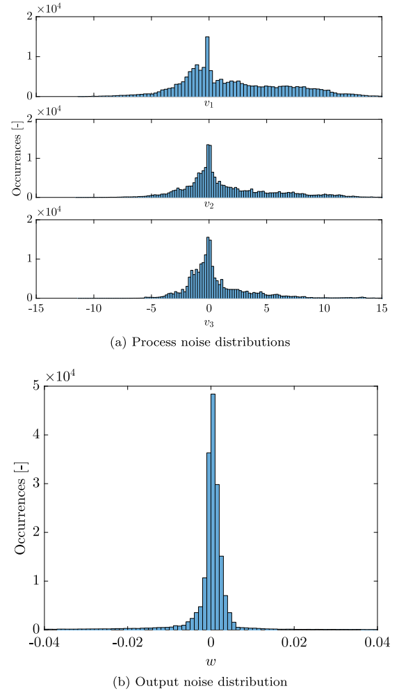
Fig. 8. In (a), the process noise distributions v_i , with i = 1, 2, 3 , evaluated over the FTP drive cycle for the Green catalyst, are shown. In (b), the output noise distribution between the real measurements \lambda_{mid_{wb}} and the model output \lambda_{wide} is depicted.
