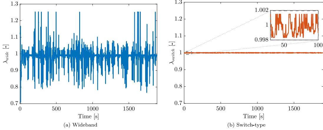
Fig. 6. Post-catalyst (a) wideband lambda sensor \lambda_{wb} , and (b) switch-type lambda sensor reading, \lambda_{mid_{sw}} (within the 0.998–1.002 range — as zoomed in the time interval 30–100 s) recorded simultaneously during the FTP driving cycle.
