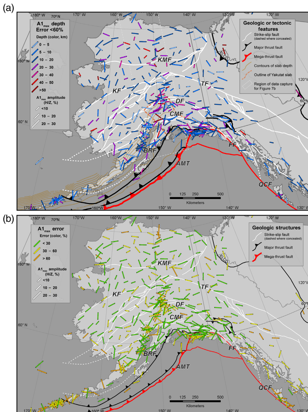
Figure 6. (a) Bars are the largest A1 arrival at each station where uncertainty is less than or equal to 60% of the A1-arrival amplitude. Bar fill is depth, length is binned by amplitude of the arrival, and orientation of the bar corresponds to the strike of the foliation at a contrast or to the strike of a dipping interface. Starburst patterns are collocated with volcanoes and resolve into concentric circles (Fig. 10c). The dashed inset box shows the region of data captured and plotted in Figure 7b. (b) Station maximum arrivals and their strikes as in A, but fill here shows amplitude uncertainty from bootstrapping. Fault names are provided in Figure 2. H/Z, horizontal-to-vertical-component amplitude ratio. The color version of this figure is available only in the electronic edition.
