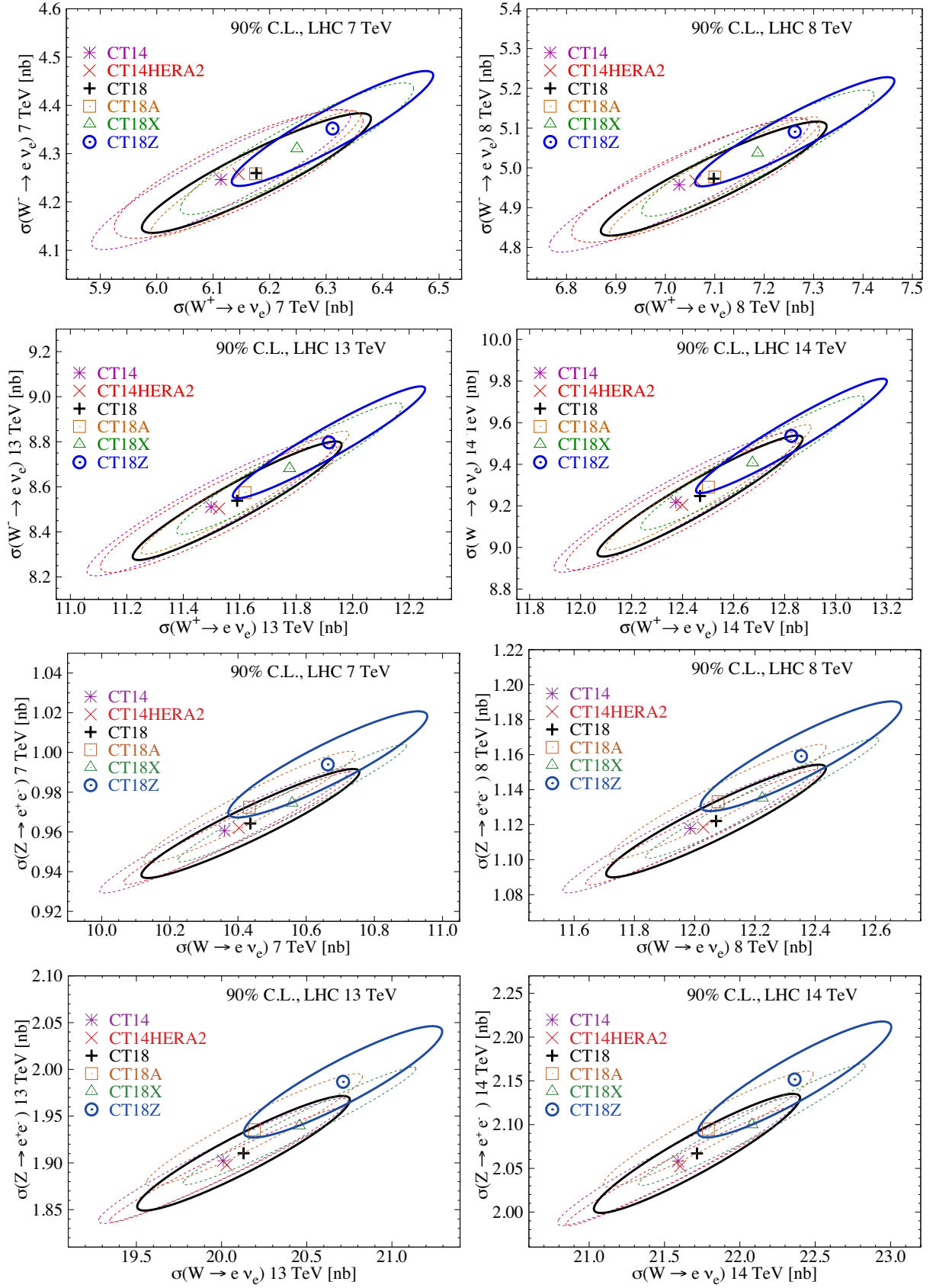
FIG. 48: Same as Fig. 47, but for the W^+ , W^- and Z^0 inclusive cross sections.
