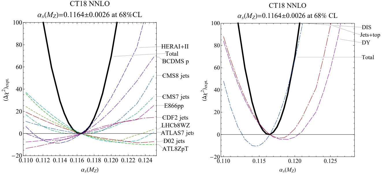
FIG. 13: The scan of the strong coupling constant at the scale of M_Z for CT18 at NNLO. Left: changes of \chi^2 of all the data sets together (heavy black line) and of several individual experiments with especially strong pull on \alpha_s(M_Z) . Right: Values for the change in \chi^2 for all experiments fitted in CT18, but separately collected into combined DIS, DY and top/jets data sets. The growth in \Delta\chi^2 for the “Jets+top” curve in the right panel is mainly driven by the constraints from jet production. While t\bar{t} production has important sensitivity to \alpha_s , the comparatively small number of top data points leads to a more intermediate impact in the full fit.
