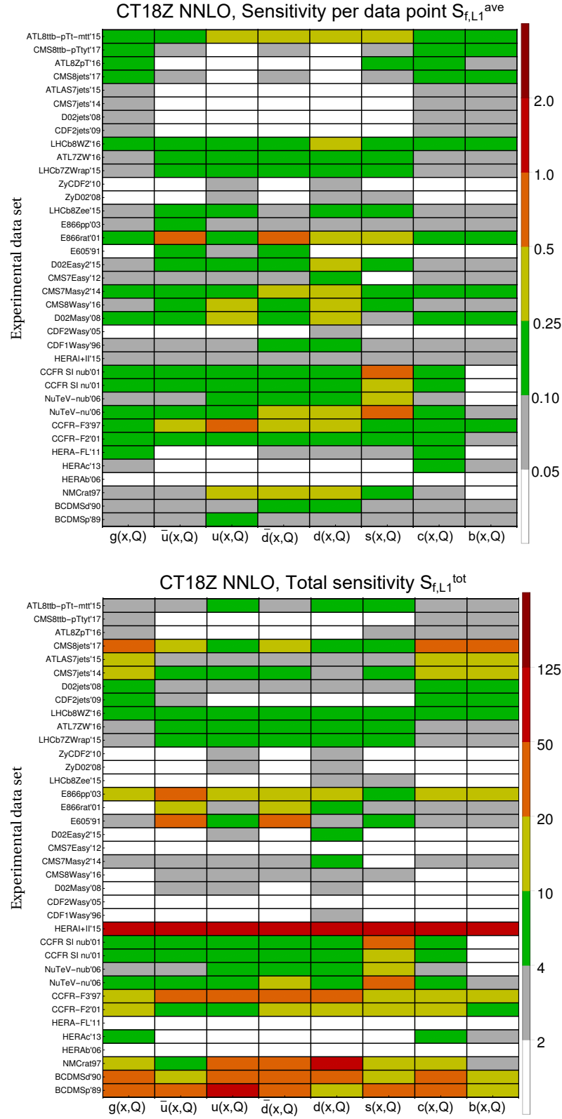
FIG. 83: L_1 sensitivities of experimental data sets to PDF flavors in the CT18Z NNLO analysis, computed according to the methodology in Ref. [20]. The color of the cells in the upper (lower) inset, chosen according to the palettes on the right, indicates the point-average (cumulative) sensitivity of the experimental set on the vertical axis to the PDF flavor on the horizontal axis.
