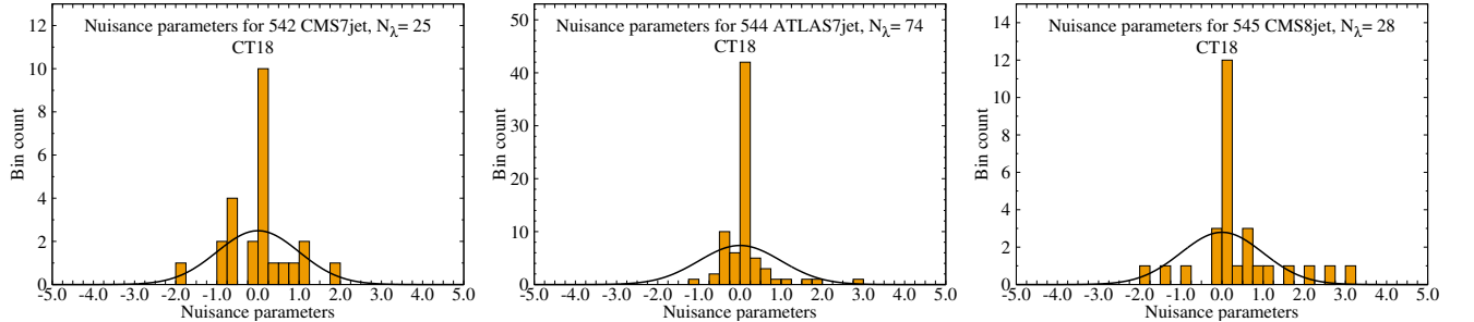
FIG. 87: Like Fig. 86, but now for the distribution of nuisance parameters obtained for the CMS 7 TeV data (Exp. ID=542, left), ATLAS 7 TeV (Exp. ID=544, center), and the CMS 8 TeV jet data (Exp. ID=545, right).
