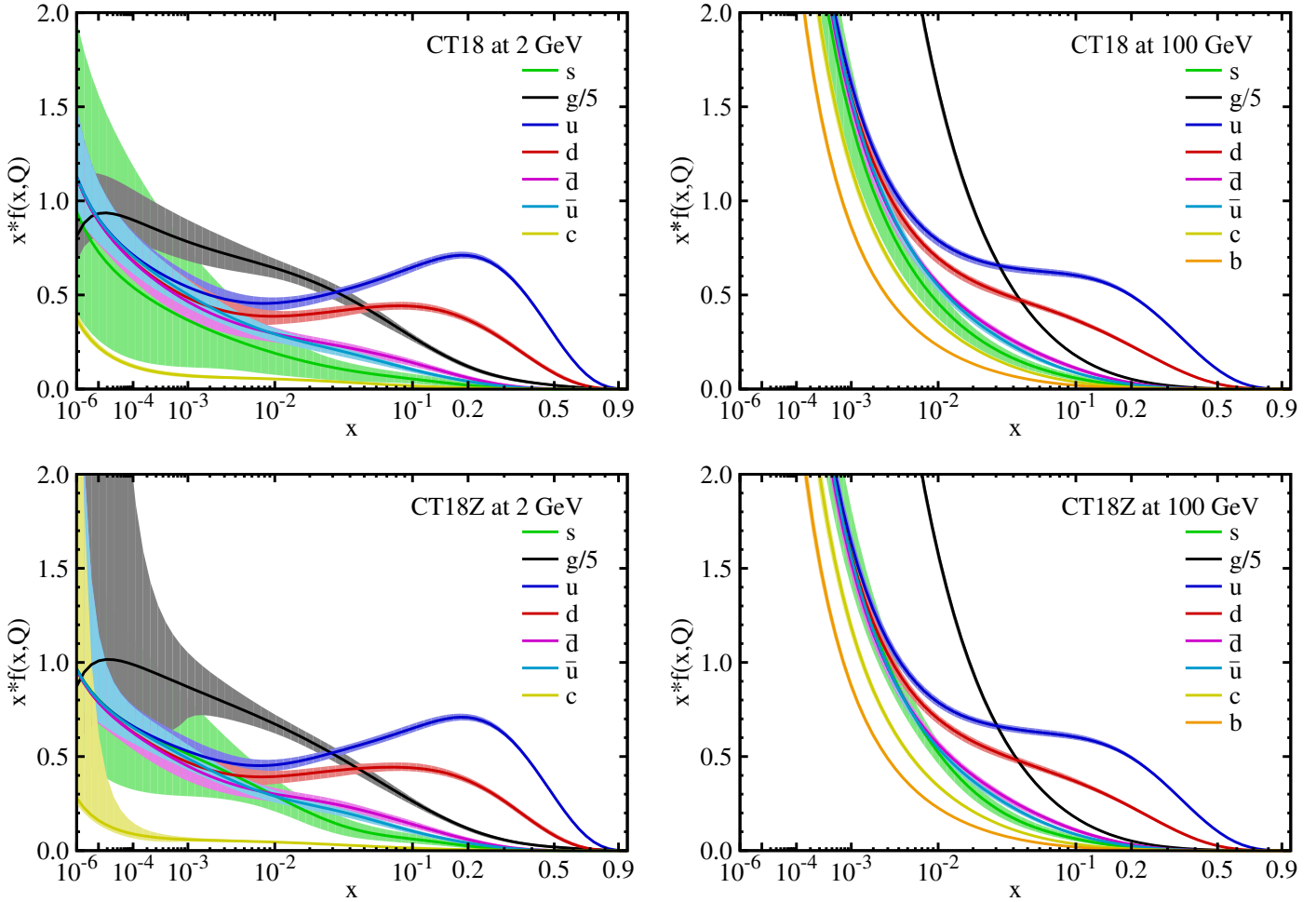
FIG. 2: Upper panels: The CT18 parton distribution functions at Q=2 GeV and Q=100 GeV for u, \bar{u}, d, \bar{d}, s, \bar{s} , and g . Lower panels: The analogous curves, but obtained for CT18Z. In all instances, the gluon PDF has been scaled down as g(x, Q)/5 . The charm distribution, c(x, Q) , which is perturbatively generated by evolving from Q_0=1.3 and 1.4 GeV, respectively, in CT18 and CT18Z, is also shown.
