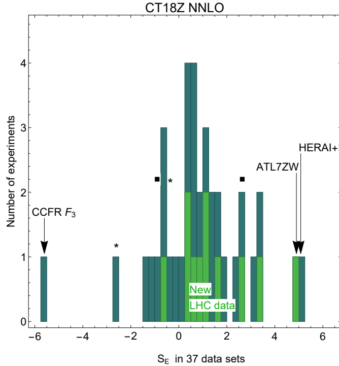
FIG. 59: Analogous to Fig. 4, the effective Gaussian variable ( S_E ) distribution of all CT18Z data sets. Two squares and two stars indicate the S_E values for the NuTeV dimuon and CCFR dimuon experiments, respectively.
