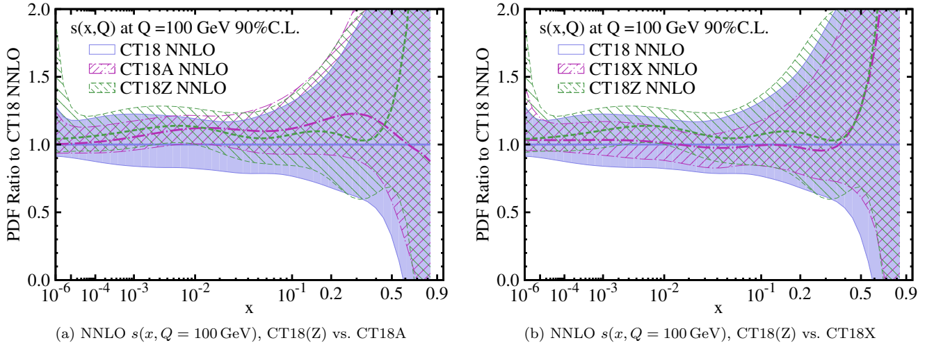
FIG. 79: Like Fig. 78, but now comparing alternative distributions for the nucleon strangeness, s(x, Q) .
