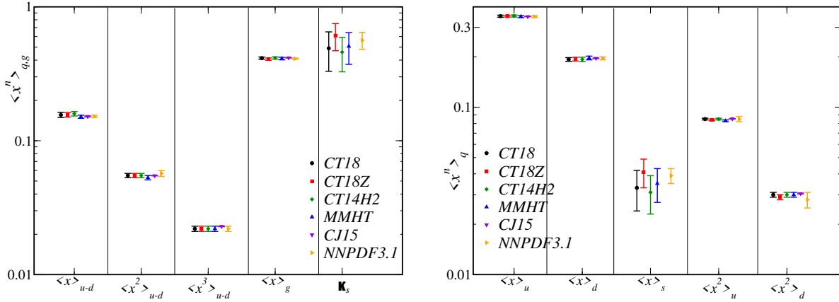
FIG. 19: A graphical comparison of the PDF moments summarized in Table VI, with the exception of the results for the zeroth moment of \bar{d} - \bar{u} combination, relevant for studies of the Gottfried Sum Rule; this latter quantity is given in Fig. 20. The CJ15 global fit does not determine \kappa_s and \langle x \rangle_s as independent entities from the data, their respective predictions are not shown.
