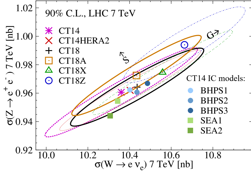
FIG. 49: Theoretical predictions of the total production cross sections of W and Z bosons at \sqrt{s} = 7 TeV as relevant for the ATLAS 7 TeV W/Z data (Exp. ID=248). Here, we also include several calculations which include an intrinsic charm (IC) PDF based upon either the BHPS valence-like model (with three different normalizations) or a sea-like model (with two different normalizations) in addition to CT14, as described in Ref. [149].
