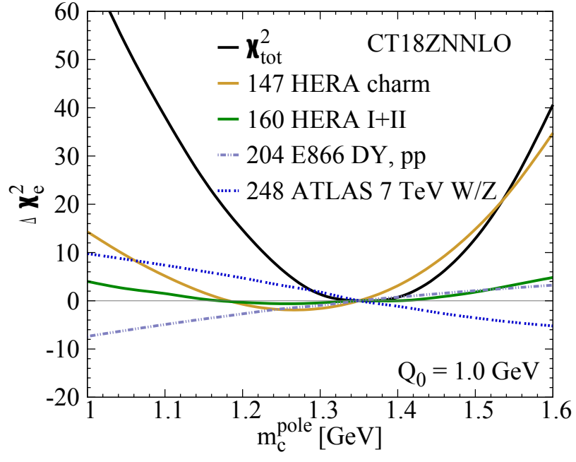
FIG. 71: Analogously to Fig. 15, the scan over values of the charm pole mass, m_c , computed here using CT18Z NNLO following the procedure described in Sec. IV B.
