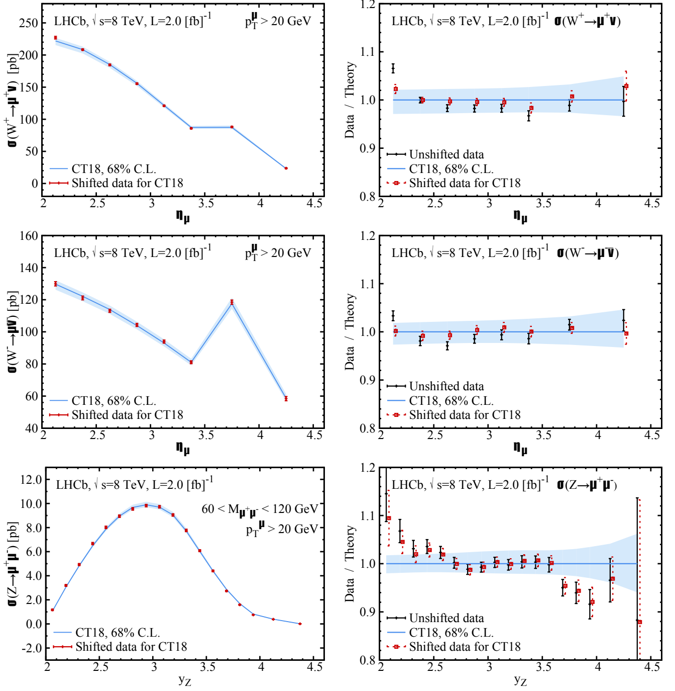
FIG. 29: A comparison of the CT18 theoretical predictions to the W^+ (top), W^- (middle), and Z^0 (bottom) cross section measurements by LHCb at 8 TeV in the muon decay channel (Exp. ID=250). The data are presented as cross sections for each bin, \sigma = \frac{d\sigma}{d\eta_\mu} \Delta\eta_\mu, \frac{d\sigma}{dy_Z} \Delta y_Z , rather than as differential cross sections. The bump in the histogram bin 3.5 < \eta_\mu < 4.0 of W^- plot thus results from its larger bin width. A similar bump occurs in the plots for the LHCb 7 TeV W/Z data (Exp. ID=245).
