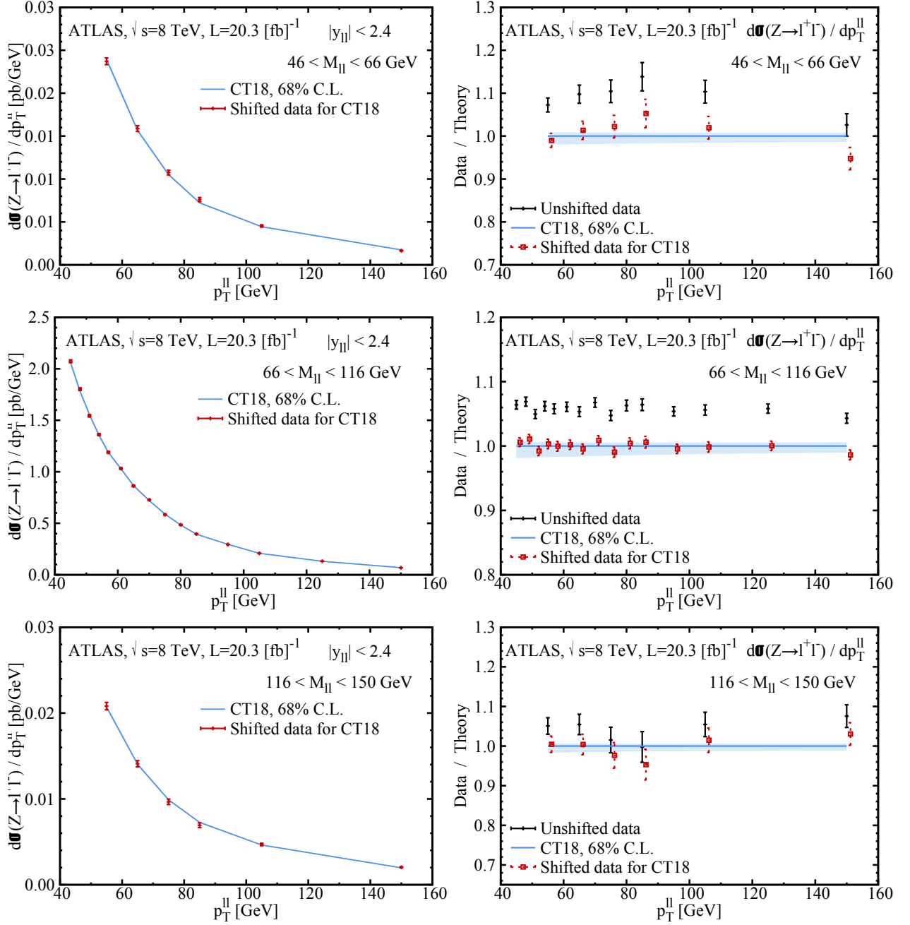
FIG. 84: A comparison of the CT18 theoretical predictions to the ATLAS 8 TeV Z p_T data (Exp. ID=253), using QCD scales \mu_R = M_{T,\ell\bar{\ell}} , \mu_F = M_{T,\ell\bar{\ell}} . Predictions for the p_T spectra measured by the ATLAS in 3 bins of the dilepton invariant mass, 46 < M_{\ell\bar{\ell}} < 66 GeV, 66 < M_{\ell\bar{\ell}} < 116 GeV, and 116 < M_{\ell\bar{\ell}} < 150 GeV, are shown in the upper, center, and lower rows, respectively. The right panels give the corresponding Data/Theory profiles for these data. The blue band represents the PDF uncertainty at the 68% C.L. The renormalization and factorization scales are chosen as \mu_R = \mu_F = M_{T,\ell\bar{\ell}} .
