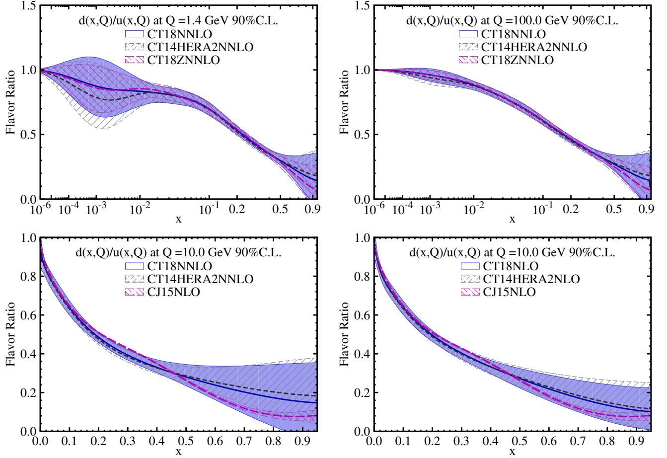
FIG. 9: Top: 90% C.L. uncertainties on the ratio d(x,Q)/u(x,Q) for CT18, CT14 HERAII , and CT18Z NNLO ensembles at Q = 1.4 and 100 GeV. Bottom: Same, comparing CT18 and CT14 HERAII NNLO ratios (bottom-left) and respective NLO ratios (bottom-right) to the CJ15 NLO ensemble at Q = 10 GeV.
