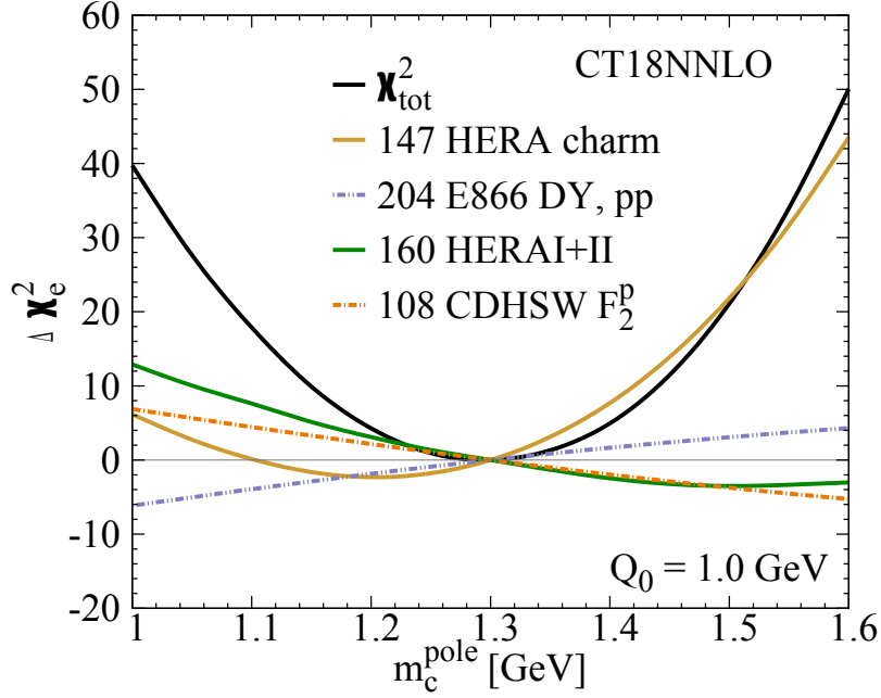
FIG. 15: A \chi^2 scan over values of the charm pole mass, m_c , at NNLO, using the CT18 data set. The settings of the fit are described in the text. The CT18Z counterpart to this m_c scan is presented in Fig. 71 in App. A.
