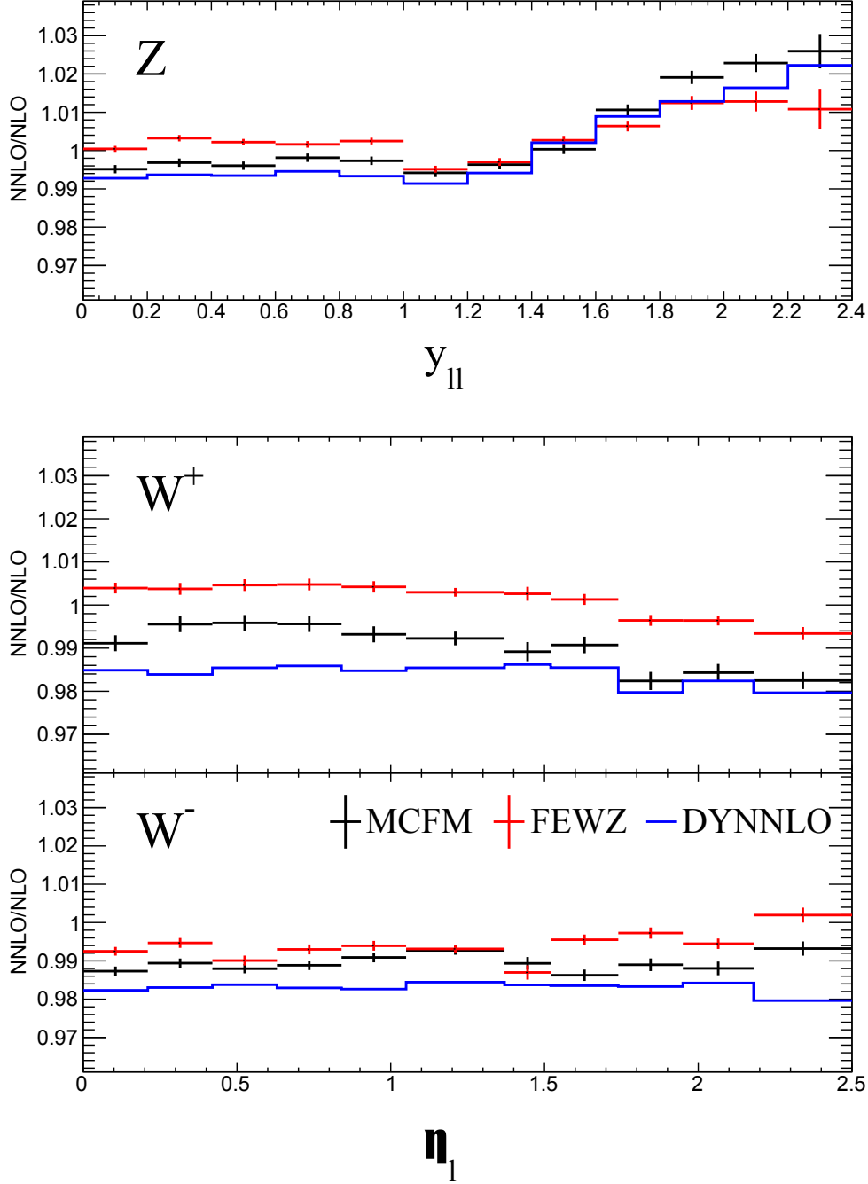
FIG. 74: The comparison of K -factors for the ATLAS 7 TeV W/Z data calculated with DYNNLO, FEWZ and MCFM. The error bars indicate the theoretical Monte-Carlo uncertainties. The DYNNLO curves are extracted from xFitter and include NLO EW corrections.
