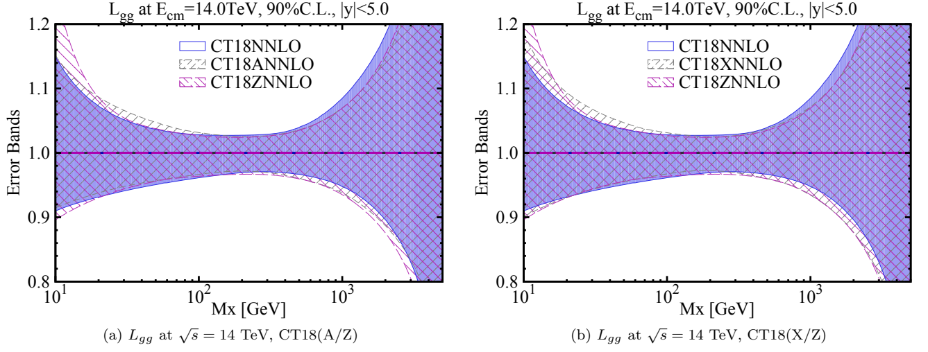
FIG. 82: Like Fig. 81, but normalizing each result for L_{gg} to its respective central-fit calculation to directly compare relative uncertainties.
