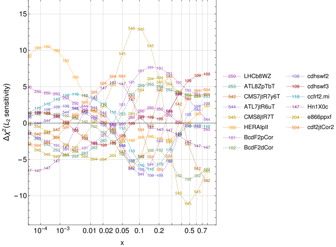
FIG. 26: The x -dependent L_2 sensitivity of the CT18 data sets with strongest pull upon the gluon PDF, g(x, Q=100 \text{ GeV}) . A number of tensions among the leading data sets are revealed by examining those regions of x where S_{f,L2}(E) peaks for certain experiments in the ‘positive direction’ while S_{f,L2}(E) is sharply negative for others. For instance, at x=0.4 , the sensitivity curves indicate a strong competition of the CMS 8 TeV jet data (Exp. ID=545) and the BCDMS F_2^d data (Exp. ID=102), both preferring a larger g(0.4, 100 \text{ GeV}) , against the combined downward pull on the gluon by the BCDMS F_2^p (101), CDHSW F_3 (109), E866 pp Drell-Yan (204), and high- p_T Z boson production (253) data sets. At x \approx 0.1 , the CMS 8 TeV jet data (Exp. ID=545) strongly pulls against the ATLAS (544) and CMS 7 TeV (542) jet production, as well as measurements by CDHSW (108), CCFR (110), and BCDMS (102) of the DIS structure function F_2(x, Q) on various targets.
