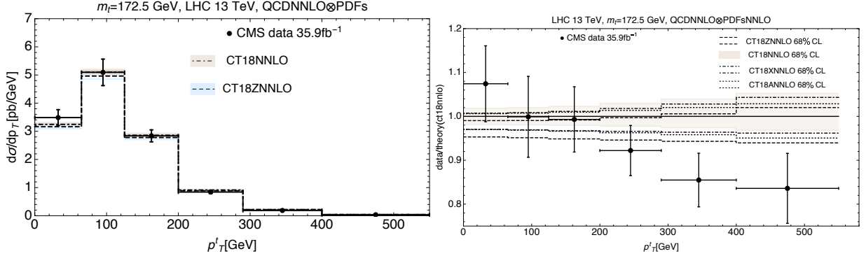
FIG. 53: Left: Top-quark transverse momentum p_{T,t} distribution. Right: Unshifted data vs. theory plot including CT18Z, CT18X, CT18A NNLO. In the right figure, data and theory predictions are normalized to CT18NNLO theory. The error bars indicate statistical and total systematic errors summed in quadrature.
