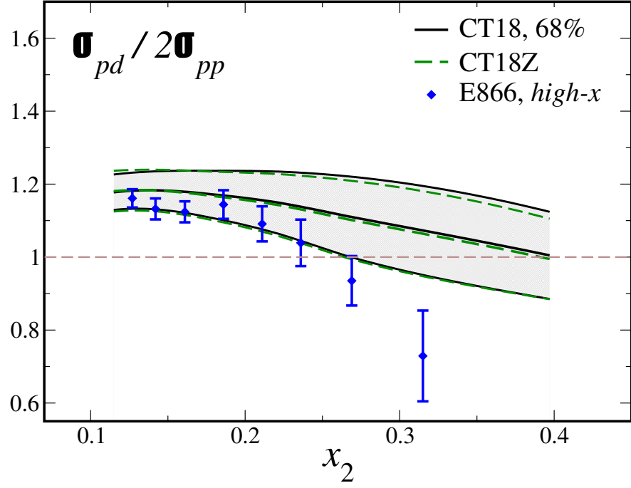
FIG. 58: Theoretical predictions based on CT18 (black outer band) and CT18Z (Green inner band) for the fixed-target Drell-Yan cross section, \sigma_{pd}/2\sigma_{pp} , in the region of larger x_2 \gtrsim 0.1 to be probed by the SeaQuest experiment [181] at Fermilab. For comparison, we also plot the higher- x_2 portion of the older E866 data [73] (blue diamonds).
