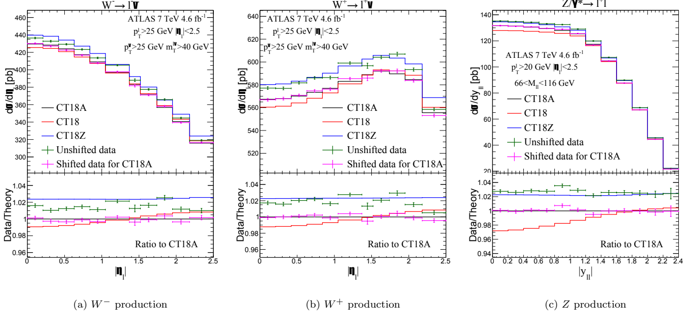
FIG. 63: (a) A comparison of theoretical predictions for the ATLAS 7 TeV 4.6 fb -1 data based on CT18 and CT18A/Z NNLO.
