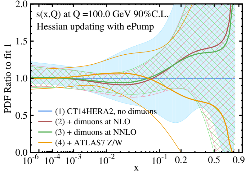
FIG. 45: Comparison of s PDF at Q = 100 GeV for various fits. See the main text for its detail.
