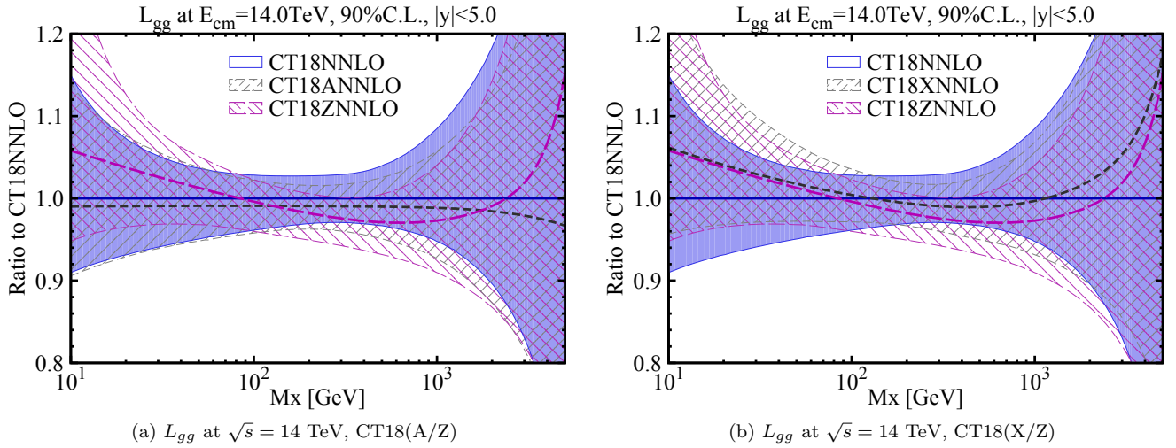
FIG. 81: A comparison of the glue-gluon parton luminosities, L_{gg} , at \sqrt{s} = 14 \text{ TeV} computed using CT18 NNLO as well as CT18A/Z (left panel) and CT18X/Z (right). All results are normalized to the central CT18 NNLO calculation.
