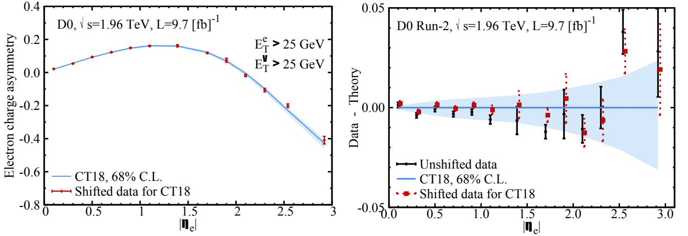
FIG. 28: A comparison of the CT18 theory with the D0 Run II electron charge-asymmetry data (Exp. ID=281). Since the asymmetry crosses zero in the shown range, the right panel shows the difference , Data–Theory, rather than the ratio , Data/Theory, as done elsewhere in this section.
