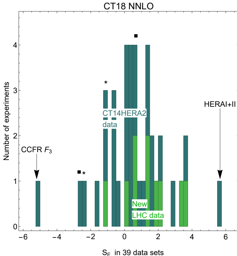
FIG. 4: A histogram of the effective Gaussian variable ( S_E ) distributed over all CT18 data sets. Two squares and two stars indicate the S_E values for the NuTeV dimuon and CCFR dimuon data, respectively.
