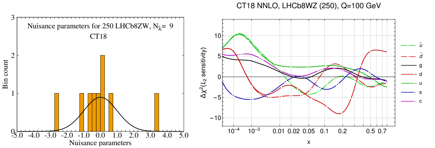
FIG. 33: Left: distribution of nuisance parameters for the LHCb 8 TeV W/Z cross sections (Exp. ID=250). Right: the pulls of these data on the CT18 NNLO PDFs at Q = 100\text{ GeV} , computed in terms of the L_2 sensitivity of Eq. (21) [166].
