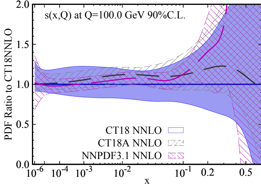
FIG. 62: A comparison of the fitted strangeness PDF, s(x, Q) , at Q=100 GeV as obtained with CT18 (solid violet) as well as with CT18A (short-dashed gray) and NNPDF3.1 (long-dashed magenta).
