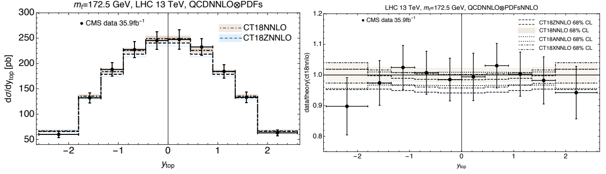
FIG. 54: Left: Top-quark rapidity y_t distribution. Right: Unshifted data vs. theory plot including CT18, CT18Z, CT18X, CT18A NNLO. Data and theory predictions are normalized to CT18NNLO theory. The error bars indicate statistical and total systematic errors summed in quadrature.
