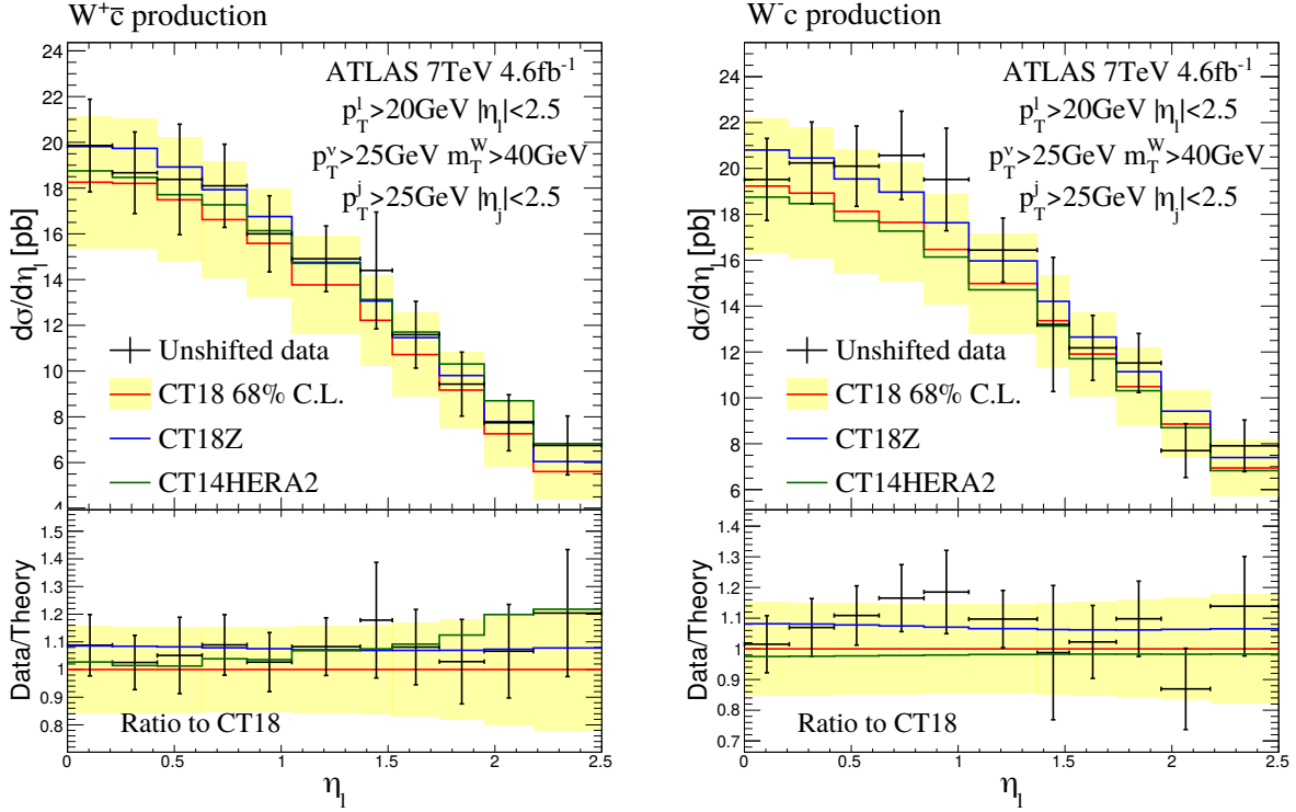
FIG. 51: Comparison of the CT18(Z) and CT14 HERAII NNLO predictions for ATLAS 7 TeV W^+ + \bar{c} -jet (left) and W^- + c -jet (right) production, respectively, for the combined electron and muon decay channels. The CT18 PDF uncertainty is evaluated at 68% CL. The scale choice is \mu_R = \mu_F = M_W .
