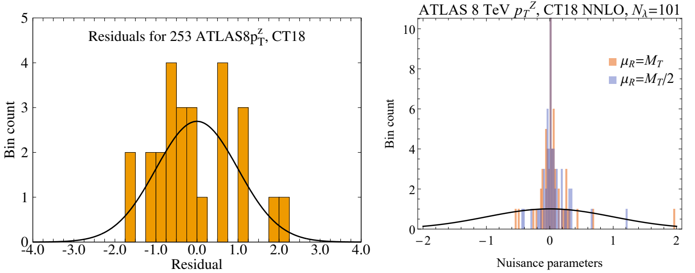
FIG. 36: Left: Distribution of the \chi^2 residuals for the ATLAS 8 TeV Z p_T data (Exp. ID=253) obtained using the nominal QCD scales in Eq. 27. Right: distributions of the respective nuisance parameters obtained for \mu_R = M_{T,\ell\bar{\ell}} (default) and M_{T,\ell\bar{\ell}}/2 , with \mu_F = M_{T,\ell\bar{\ell}} in both cases.
