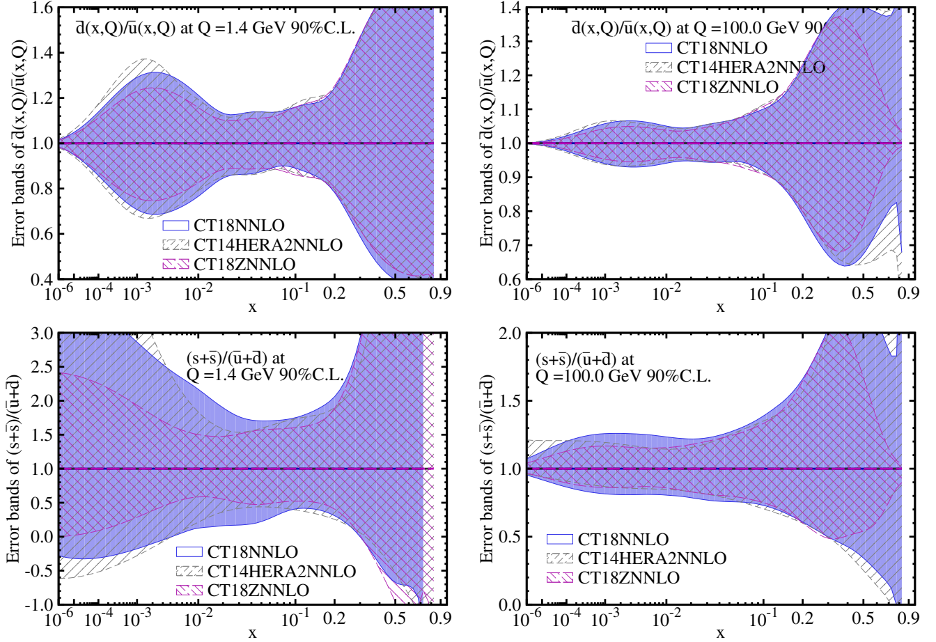
FIG. 12: A comparison of 90% C.L. uncertainties on the ratios \bar{d}(x, Q)/\bar{u}(x, Q) and (s(x, Q) + \bar{s}(x, Q)) / (\bar{u}(x, Q) + \bar{d}(x, Q)) , for CT18 (solid blue), CT18Z (magenta long-dashed), and CT14 HERAII NNLO (gray short-dashed) ensembles at Q = 1.4 or 100 GeV, relative to their own central fit.
