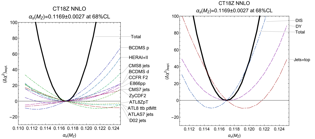
FIG. 70: Scans over the strong coupling at the scale of M_Z for CT18Z, analogous to Fig. 13 for CT18. As before, we show in the left panel the \Delta\chi^2 variations for a number of experiments with leading sensitivity to \alpha_s(M_Z) , while the right panel again shows the change in \chi^2 for all experiments fitted in CT18Z, separately collected into combined DIS, DY and top/jets data sets. Also as before, the “Jets+top” curve in the right panel is primarily influenced by the jet production data sets. Due to the intermediate impact of the t\bar{t} data noted in Fig. 13, variations in the CT18 fit leading to CT18Z are such that the ATLAS 8 TeV t\bar{t} data (Exp. ID=580) are now selected with the ensemble of sensitive experiments in the left panel.
