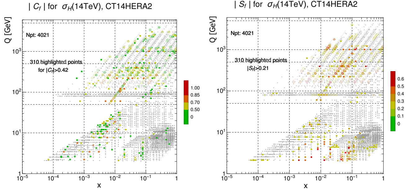
FIG. 5: Left: Candidate data considered for inclusion in CT18 evaluated according to the magnitude of the Pearson correlation C_f between the total Higgs cross section at 14 TeV, \sigma_H(14\text{TeV}) and the residual of each point as determined within the PDFSense framework [20]. Right: A similar assessment of the CT18 candidate data, but computed on the basis of the sensitivity , |S_f|(x_i, Q_i) . In both panels, a highlighting cut has been imposed to draw attention to the \sim 300 highest-impact points according to each metric.
