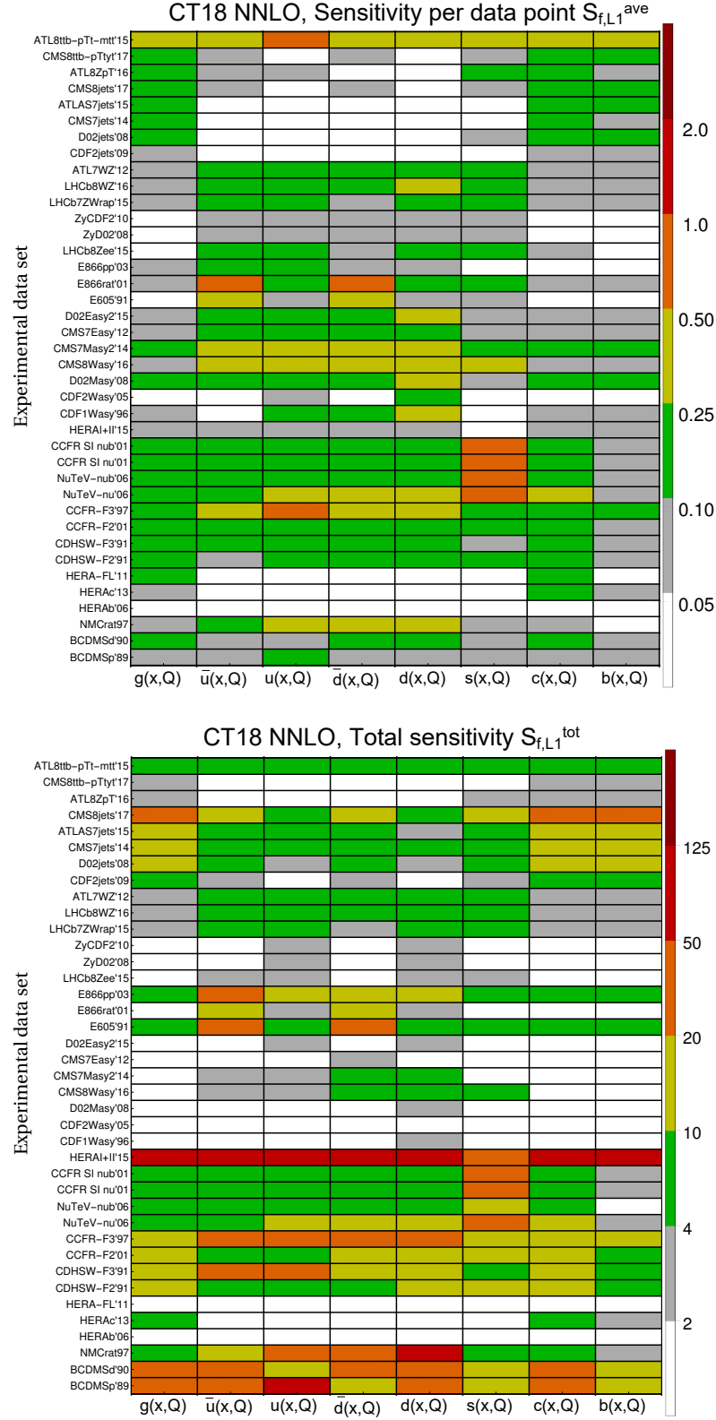
FIG. 27: L_1 sensitivities of experimental data sets to PDF flavors in the CT18 NNLO analysis, computed according to the methodology in Ref. [20]. The color of the cells in the upper (lower) inset, chosen according to the palettes on the right, indicates the point-average (cumulative) sensitivity of the experimental set on the vertical axis to the PDF flavor on the horizontal axis.
