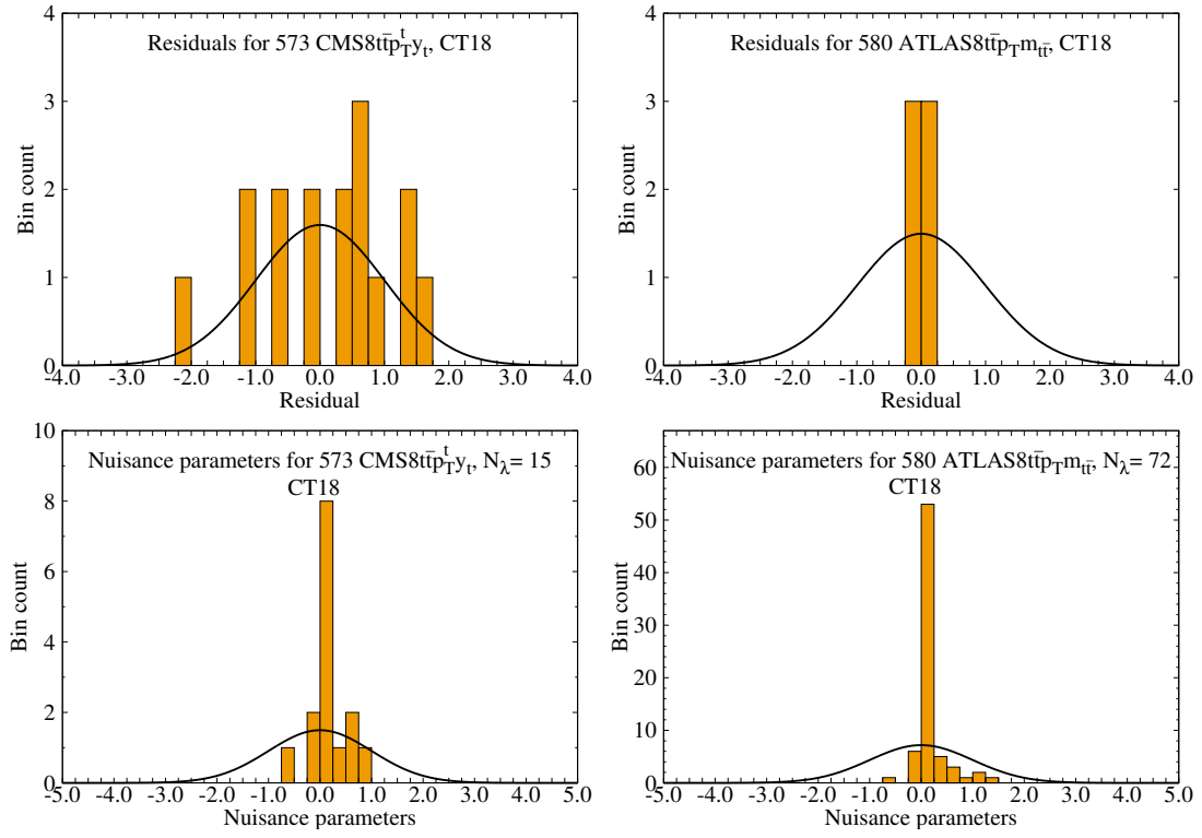
FIG. 88: Distribution of residuals (upper panels) and nuisance parameters (lower panels) for the CMS (left panels, Exp. ID=573) and ATLAS (right panels, Exp. ID=580) 2D top quark pair data.
