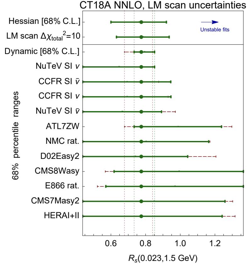
FIG. 69: 68% C. L. uncertainty ranges on R_s(0.023, 1.5 \text{ GeV}) obtained based on \chi^2 variations and Hessian estimates. For the dynamic tolerance and tolerance ranges for individual experiments, the green solid (red dashed) bands correspond
