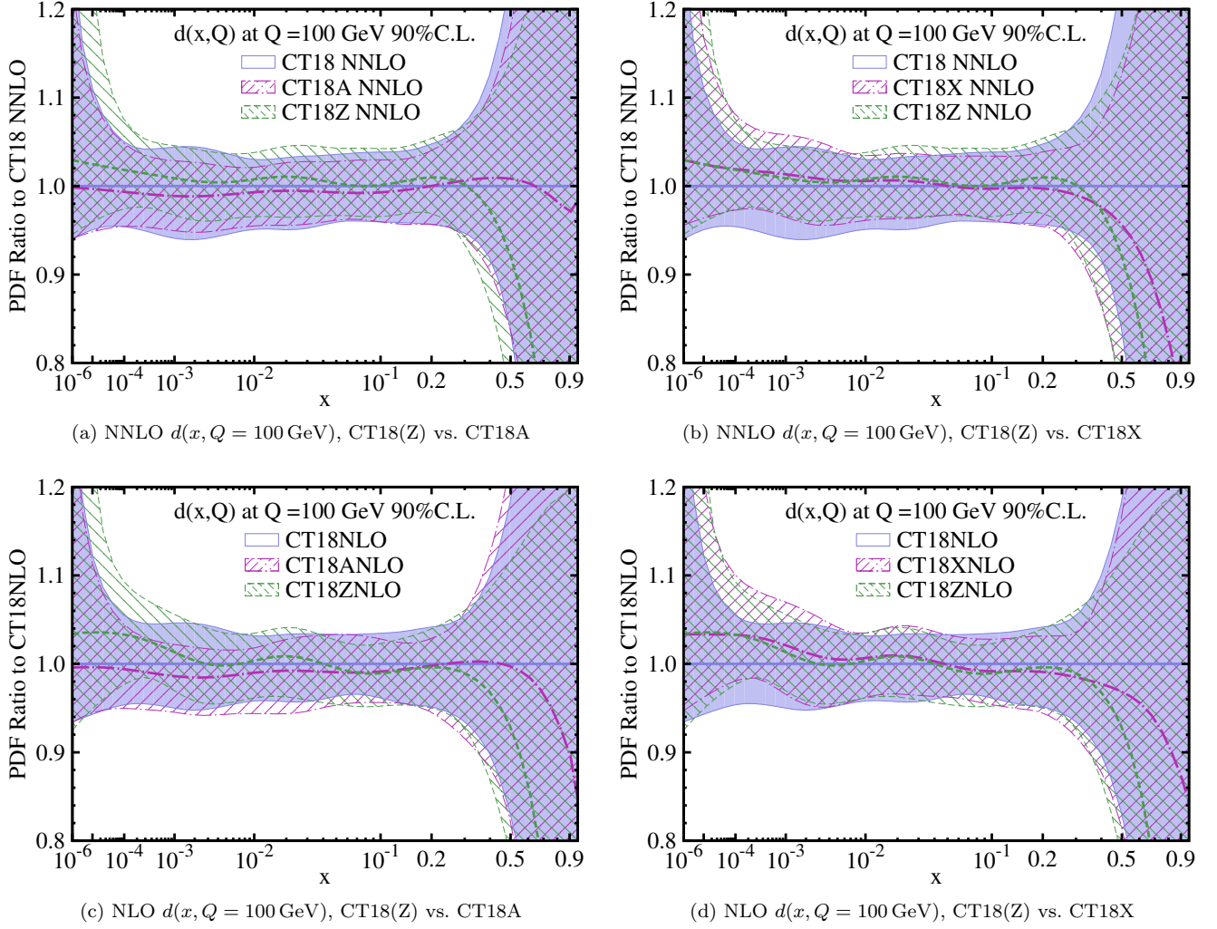
FIG. 77: A comparison of the d -quark PDF ratios with respect to CT18 for the CT18(Z) PDFs vs. the CT18A/X alternative fits. The plots here are analogous to those shown for the gluon in Fig. 76.
