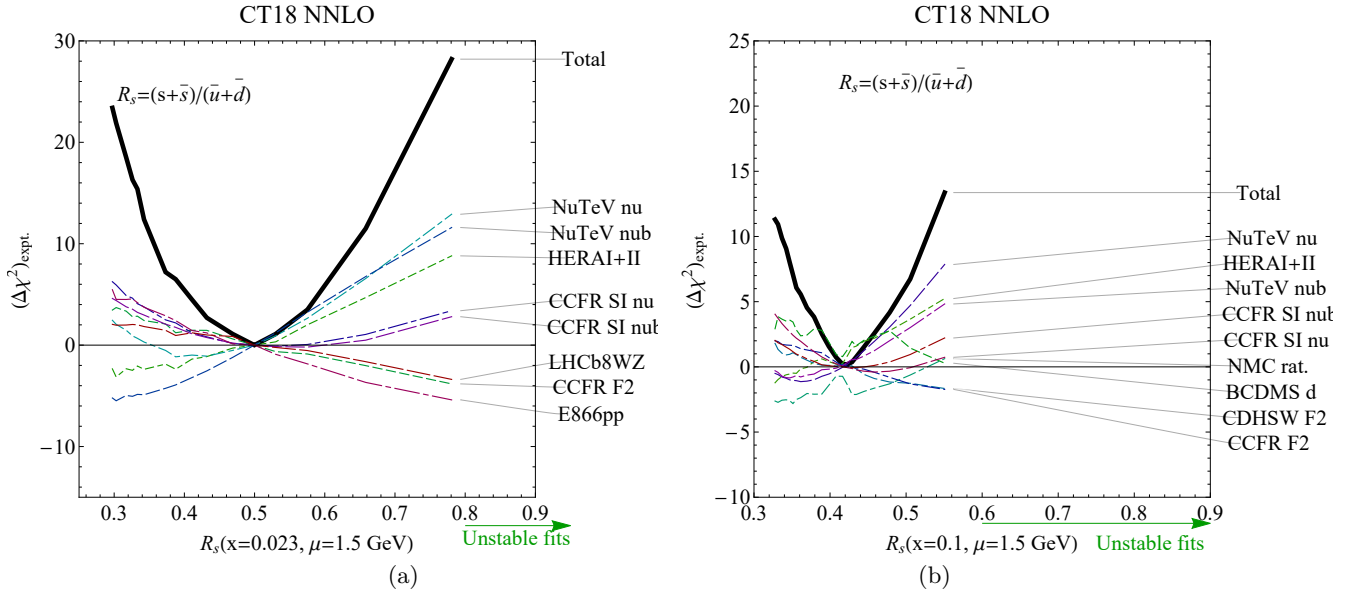
FIG. 24: The LM scan over R_s at Q = 1.5 GeV, with x = 0.023 and x = 0.1 respectively, for the CT18 NNLO fit.
