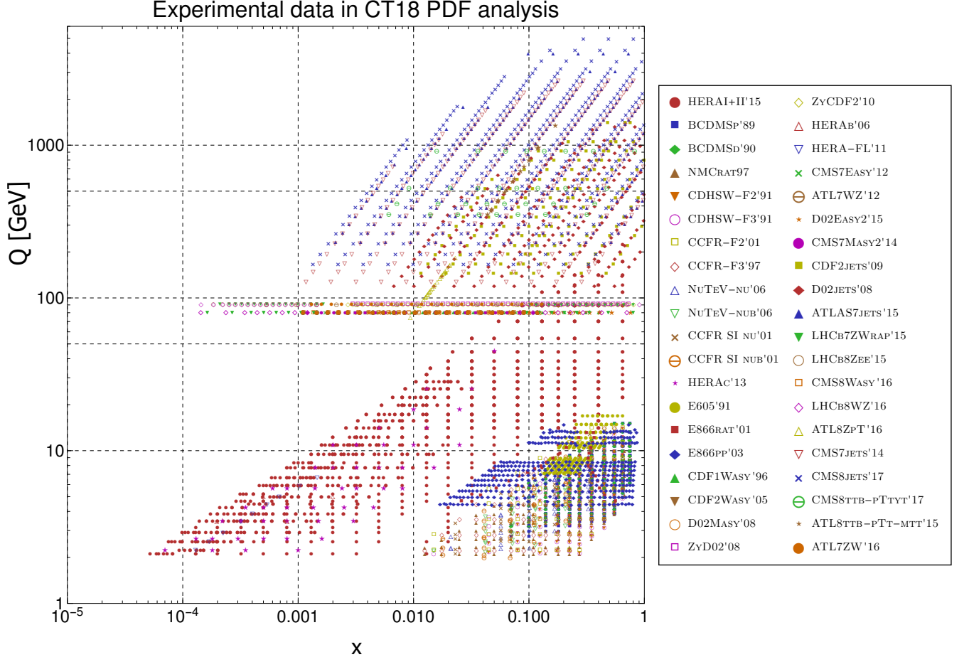
FIG. 1: The CT18 data set, represented in a space of partonic (x, Q) , based on Born-level kinematical matchings, (x, Q) = (x_B, Q) , in DIS, etc. . The matching conventions used here are described in Ref. [20]. Also shown are the ATLAS 7 TeV W/Z production data (ID=248), labeled ATL7WZ'12, fitted in CT18Z.
