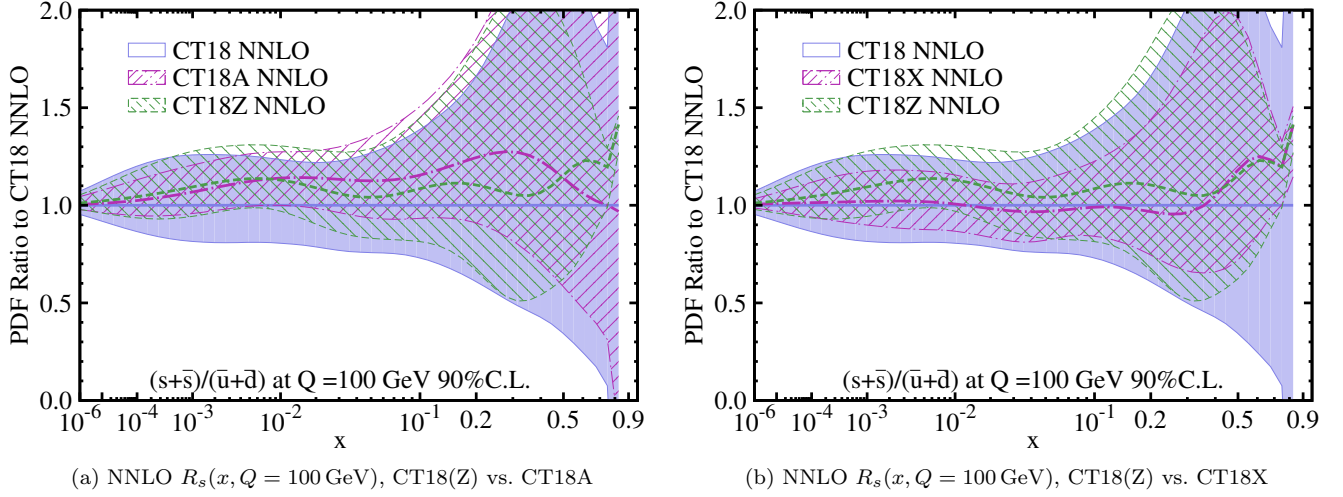
FIG. 80: The strange suppression factor, R_s \equiv (s + \bar{s})/(\bar{u} + \bar{d}) , for the CT18(Z) and CT18A/X NNLO alternative fits, evaluated with respect to the primary, CT18 NNLO result.
