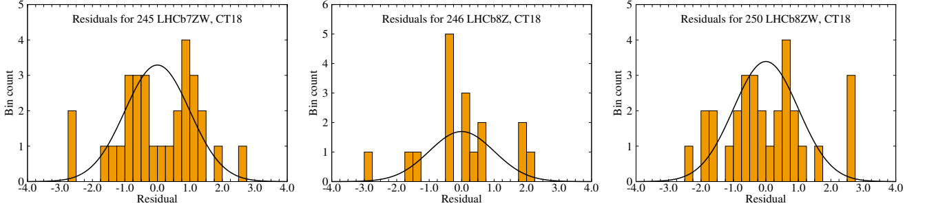
FIG. 32: Distributions of the residuals for the LHCb W/Z production cross sections at 7 and 8 TeV: Exp. ID=245 (left), 246 (center), and 250 (right).
