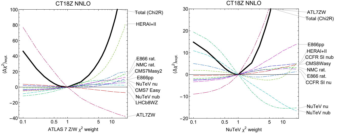
FIG. 67: (Left panel) The change in total \chi^2 , \Delta\chi^2 , of the leading data sets included in the CT18Z NNLO fit when varying the weight of the ATL7ZW data away from weight w=1 as in the default fit. (Right panel) The analogous plot for the NuTeV \nu, \bar{\nu} SIDIS dimuon data (Exp. IDs=124, 125).
