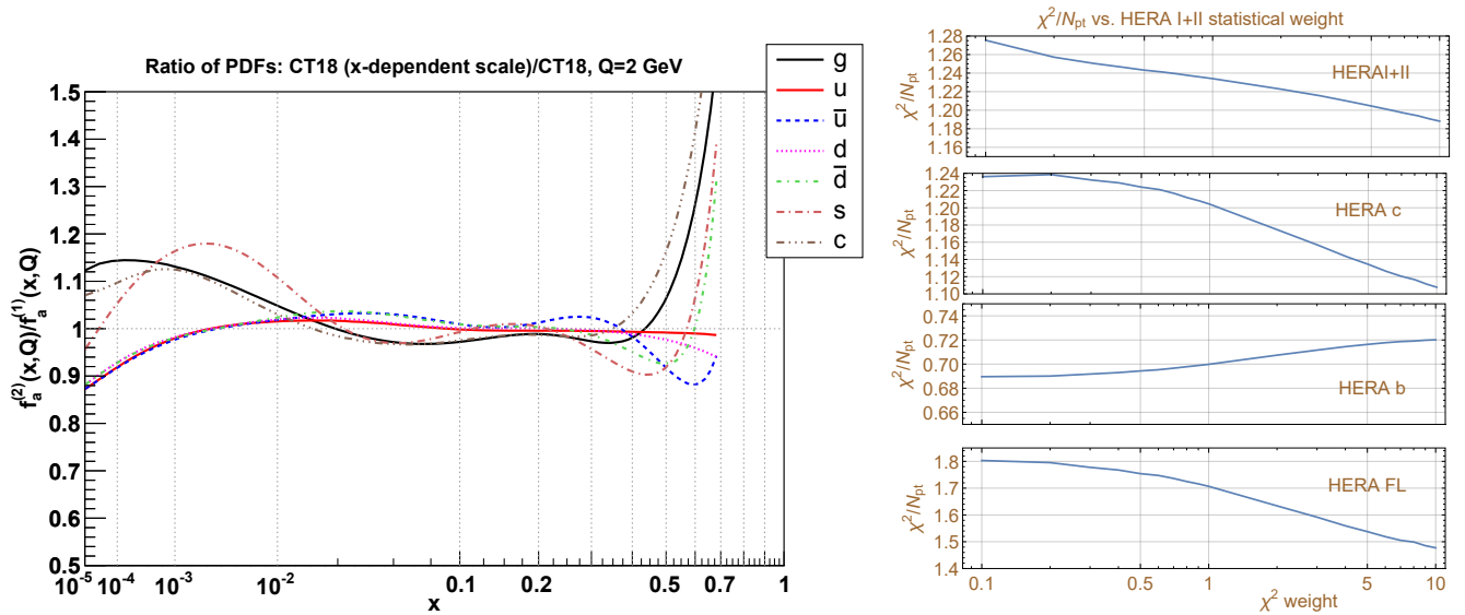
FIG. 3: Left: The ratios of the candidate CT18 NNLO PDFs obtained with the x_B -dependent and standard factorization scales in DIS data sets. Right: The \chi^2/N_{pt} values for four HERA data sets in the CT18Z fit with the x_B -dependent DIS factorization scale and varied statistical weight of the HERA I+II inclusive DIS data set.
