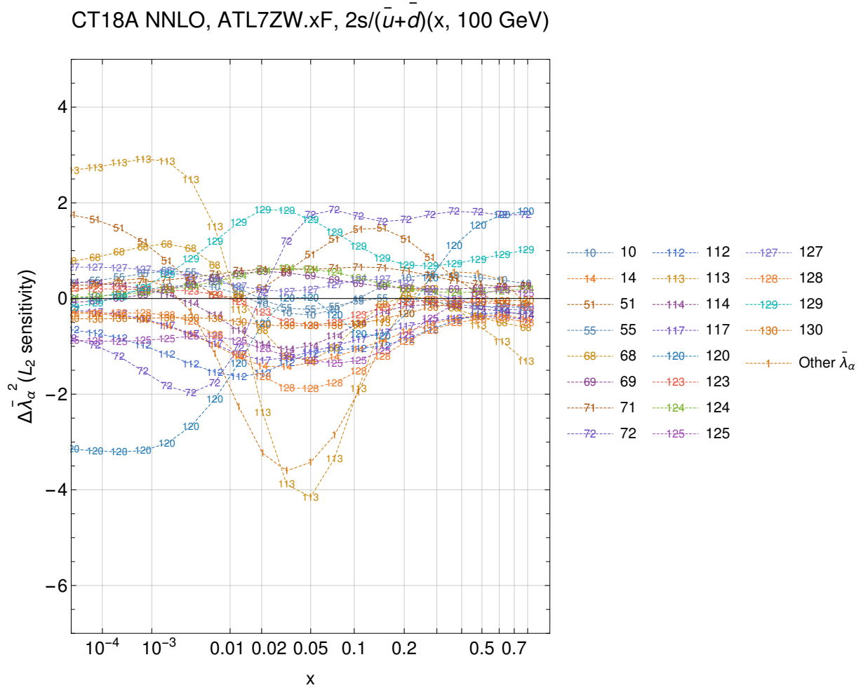
FIG. 66: A plot, analogous to the L_2 sensitivity plots given above, showing the pulls of the correlated systematic uncertainties of the ATLAS W/Z data on R_s(x, Q = 100 \text{ GeV}) in CT18A NNLO, as represented by shifts in the associated squared nuisance parameters, \Delta\bar{\lambda}_\alpha^2 .
