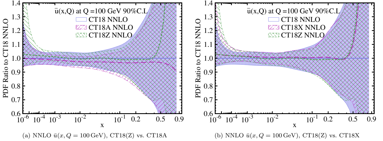
FIG. 78: As with Fig. 77, we explore the \bar{u} -antiquark PDF ratios at NNLO, comparing CT18(Z) with CT18A NNLO in panel (a), and with CT18X in panel (b).
