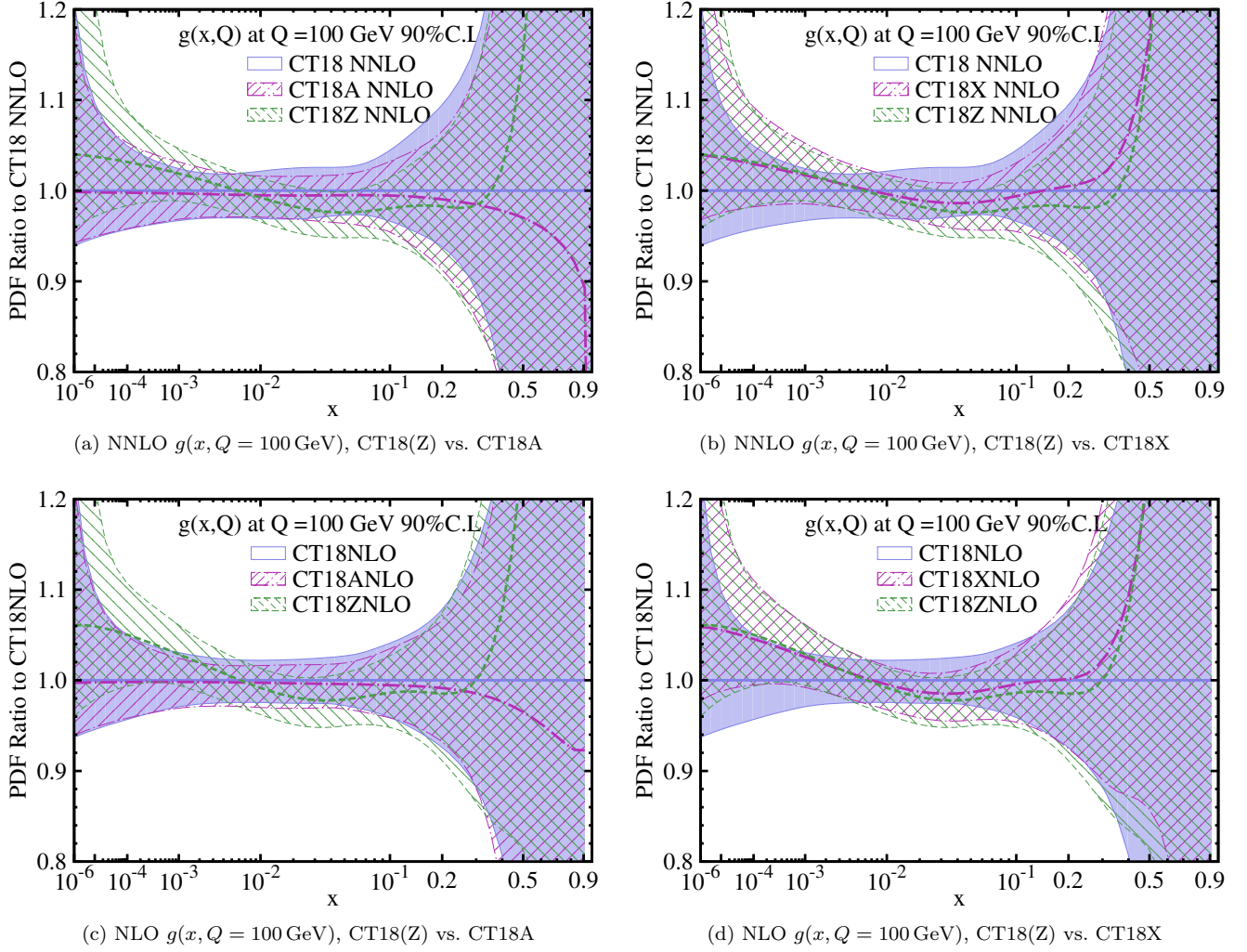
FIG. 76: Gluon PDF ratios for the CT18Z and CT18A/X alternative fits, evaluated with respect to the primary, CT18 result. In the left panels [(a) and (c)], we compare CT18(Z) against CT18A, whereas the right panels [(b) and (d)] overlay CT18(Z) with CT18X. In addition, we examine differences for NNLO and NLO fits; the upper panels [(a) and (b)] are NNLO, and the lower panels [(c) and (d)] are NLO.
