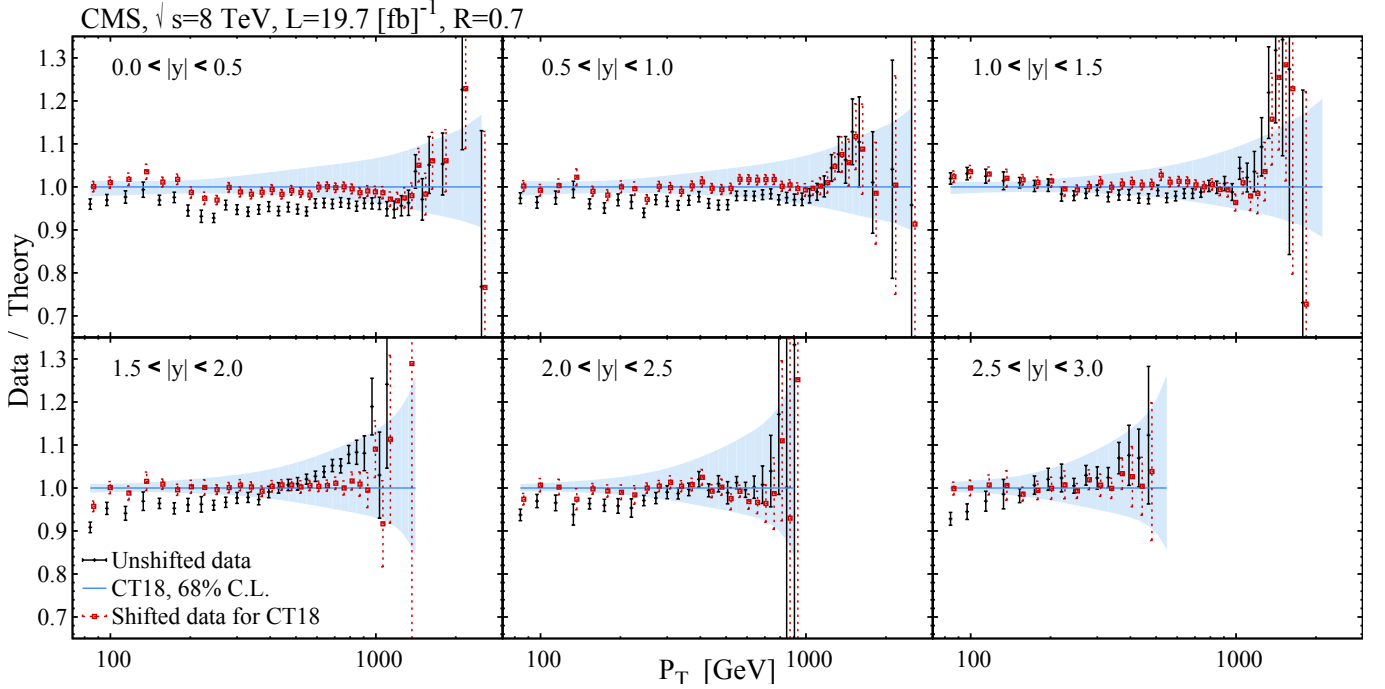
FIG. 41: Data/Theory values for CT18 NNLO and CMS 8 TeV inclusive jet production (Exp. ID=545).
