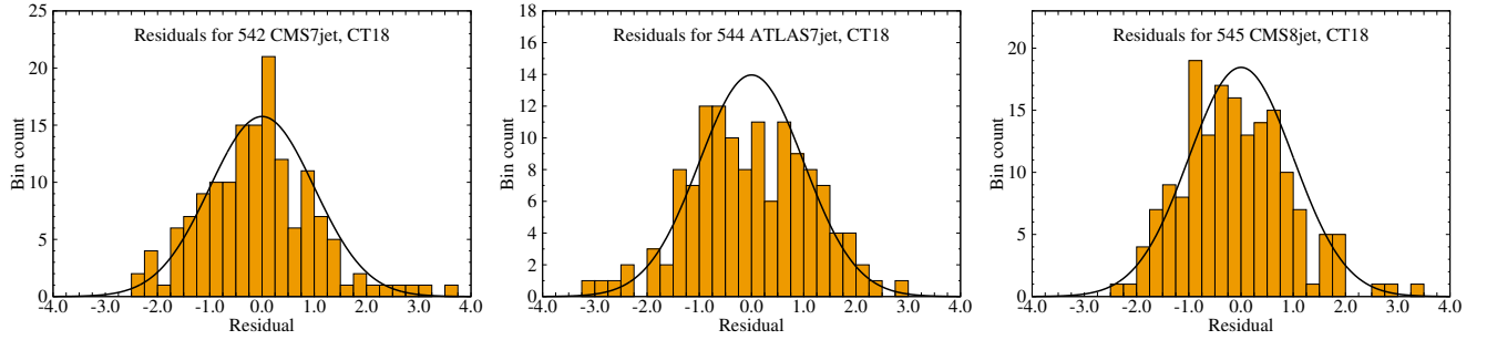
FIG. 86: We plot histograms giving the distribution of shifted residuals, r_i of Eq. (3), for each of the newly-included LHC jet experiments: the CMS 7 TeV data (Exp. ID=542, left), ATLAS 7 TeV (Exp. ID=544, center), and the CMS 8 TeV jet data (Exp. ID=545, right).
