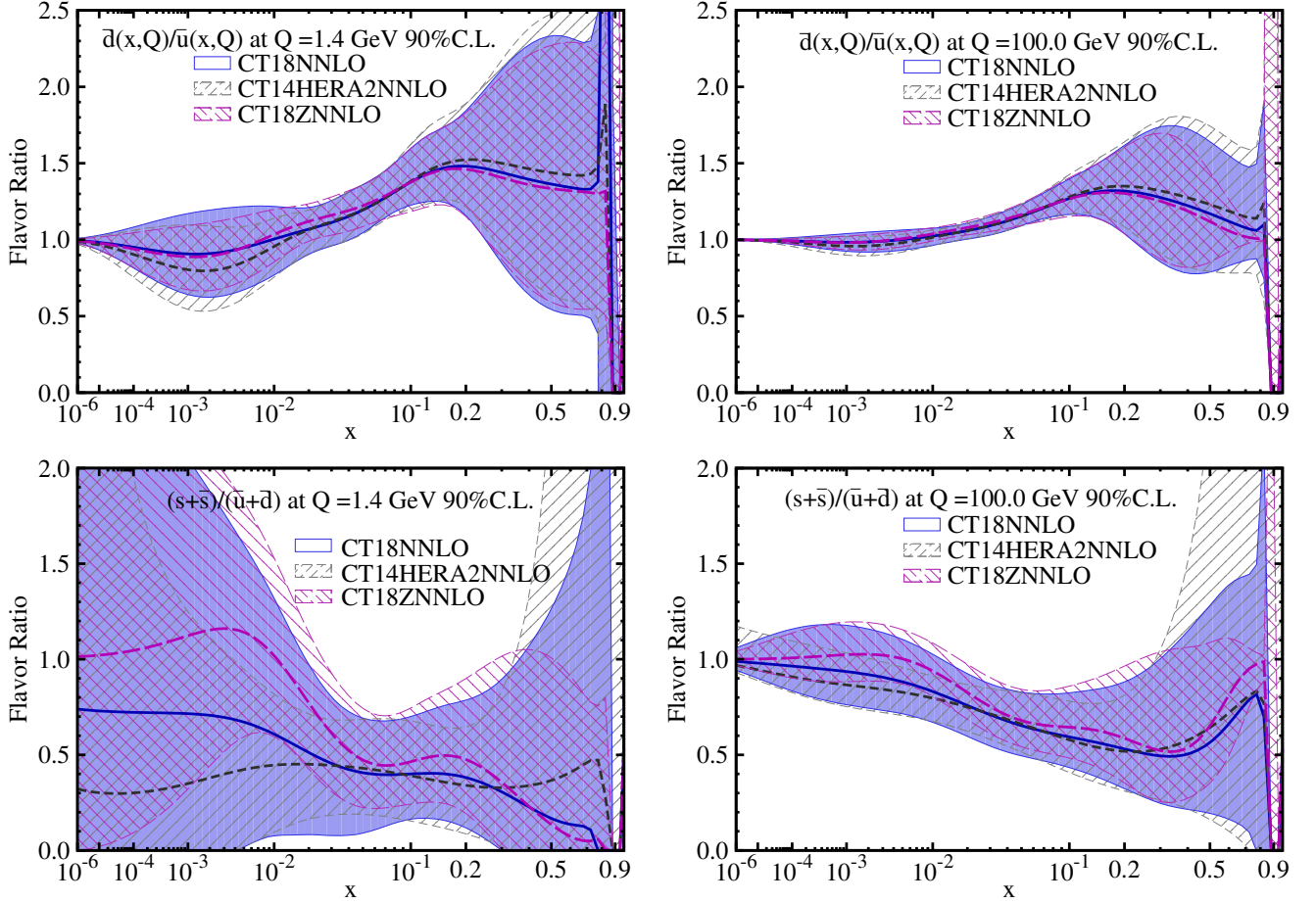
FIG. 11: A comparison of 90% C.L. uncertainties on the ratios \bar{d}(x,Q)/\bar{u}(x,Q) and (s(x,Q) + \bar{s}(x,Q)) / (\bar{u}(x,Q) + \bar{d}(x,Q)) , for CT18 (solid blue), CT18Z (magenta long-dashed), and CT14 HERAII NNLO (gray short-dashed) ensembles at Q = 1.4 or 100 GeV.
