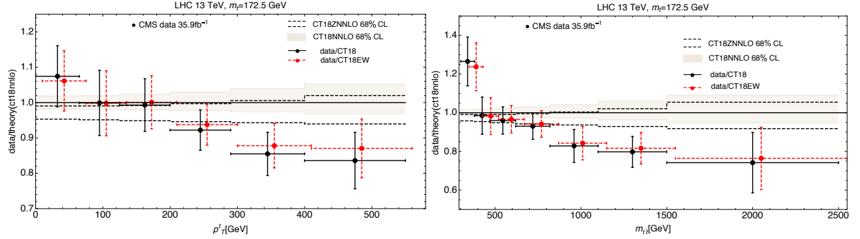
FIG. 56: Impact of NLO EW corrections. Unshifted data vs. theory plot for top-quark p_T distribution and the invariant mass distribution of the t\bar{t} pair. The error bars are statistical and total systematic errors summed in quadrature. The red data points with dashed error bars represent data divided by the CT18NNLO theory with NLO EW corrections. The black data points with solid error bars represent data normalized to the CT18NNLO theory. The CT18ZNNLO theory prediction (black dashed error band) is also normalized to CT18NNLO. The data vs (theory+EW) points are slightly shifted to the right in the same bin to improve visualization.
