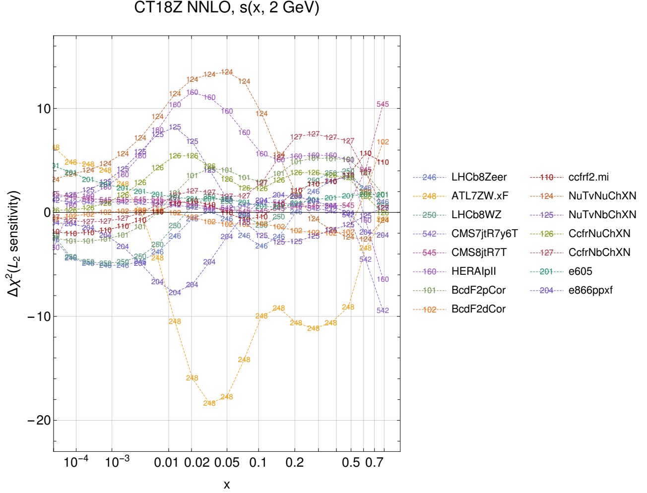
FIG. 61: The L_2 sensitivity of the data fitted in CT18Z to the x -dependent strange PDF at Q = 2 \text{ GeV} . Given that the fitted behavior for R_s(x, Q) is substantially driven by s(x, Q) , the information shown here is complementary to the LM scans in Fig. 68.
