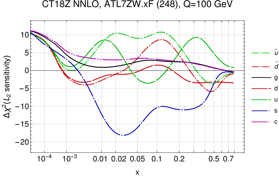
FIG. 60: The L_2 sensitivity of the ATL7ZW data to the PDFs of several individual parton flavors. The pull on the strangeness distribution, s(x, Q) , is particularly large, peaking at S_{s, L2} \sim -20 for x \sim 0.02 - 0.05 ; although opposing pulls on the d -, \bar{u} -, and \bar{d} -quark PDFs are also significant in a similar region of x .
