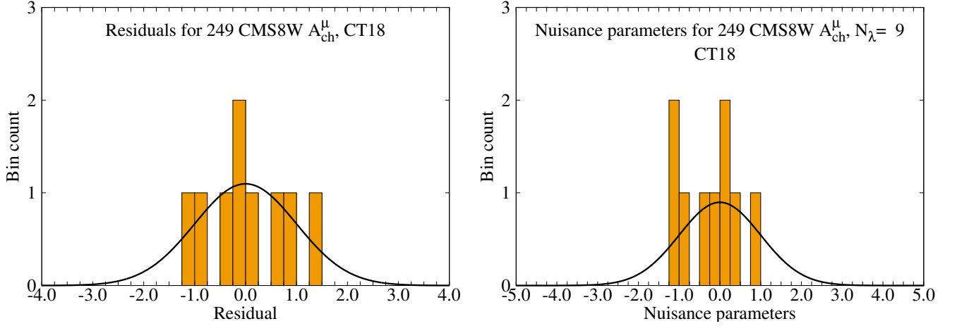
FIG. 85: Distribution of residuals (left) and nuisance parameters (right) for the CMS 8 TeV W -lepton charge asymmetry data (Exp. ID=249).
