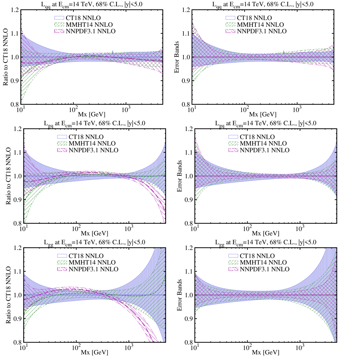
FIG. 18: Same as Fig. 16, comparing the CT18, MMHT'2014, and NNPDF3.1 NNLO parton luminosities with \alpha_s(M_Z) = 0.118 .
