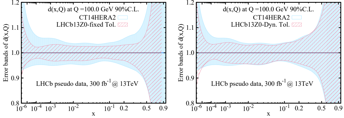
FIG. 13: PDF uncertainties associated with the d quark distribution, as a function of x , in the CT14HERA2 PDFs and \text{EPUMP} updated new PDFs. The denominator is the central set of each PDF sets. The rapidity distribution of Z boson events ( 300\text{fb}^{-1} ) is used as input to the \text{EPUMP} update. (left) The result with fixed tolerance of \Delta\chi^2 = (1.645)^2 at the 90% CL, and (right) the result with dynamical tolerance.
