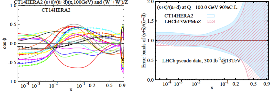
FIG. 12: (left) \cos \phi between the PDF ratio \frac{s+\bar{s}}{\bar{u}+\bar{d}} and the (W^+ + W^-)/Z ratio. Lines with different color represent different bins, and the same index as Fig. 1 is used. (right) The PDF uncertainties associated with \frac{s+\bar{s}}{\bar{u}+\bar{d}} distribution, using the 300 \text{ fb}^{-1} data, as a function of x , in the CT14HERA2 PDFs and ePUMP updated new PDFs. The denominator is the central value of each PDF set. The single (W^+ + W^-)/Z boson differential cross sections are taken as the ePUMP input.
