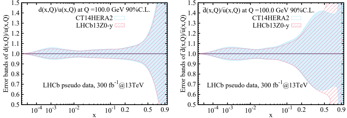
FIG. 6: PDF uncertainties associated with d/u (left) and \bar{d}/\bar{u} (right), as a function of x , in the CT14HERA2 PDFs and ePUMP updated new PDFs. The denominator is the central value of each PDF set. The rapidity distribution of Z boson events is used as input of the ePUMP update. (left) The d/u quark result using 300 \text{ fb}^{-1} data, and (right) the \bar{d}/\bar{u} quark result using 300 \text{ fb}^{-1} data.
