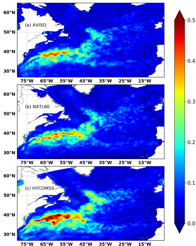
Figure 3. Standard deviation of sea surface height based on 1 year datasets for (a) AVISO, (b) NATL60 and (c) HYCOM50. The SSH values for NATL60 and HYCOM50 were degraded to 0.25^\circ spatial resolution. In this comparison, we have used AVISO mean dynamical topography data set from October 2012 to September 2013. SSH, sea surface height.
