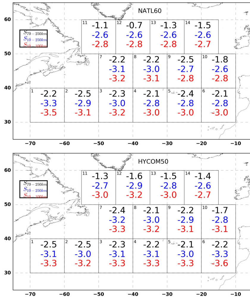
Figure 8. Map of spectral slope estimated from the surface kinetic energy spectral density for three different selected wavenumber ranges. Color red, blue and black represent 10–100 km, 10–250 km and 70–250 km respectively.
