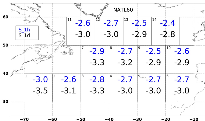
Figure 10. Map of spectral slope from the surface kinetic energy spectral density computed from daily versus hourly Fields. The slope is estimated between the model effective resolution ( E_p ) and the energy containing scale ( \lambda_e ).
