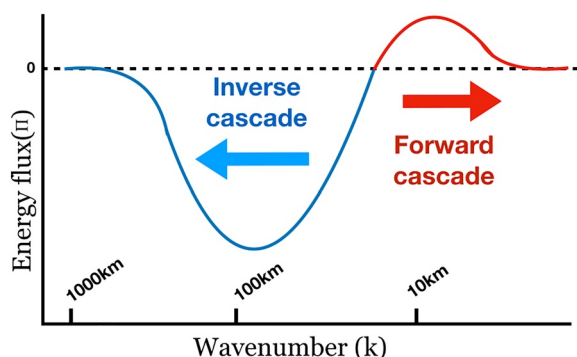
Figure 1. Schematics of kinetic energy spectral flux in the ocean at mid-latitude. Blue: inverse cascade of energy, Red: forward cascade of energy.
