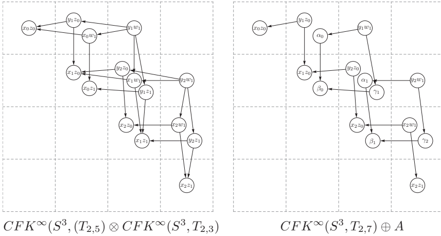
Figure 16. Notation: x_i z_{i'} = [x, i, k-i] \otimes [z, i', 1-i'] , x_i w_1 = [x, i, k-i] \otimes [w, 1, 1] , y_i z_{i'} = [y, i, k+1-i] \otimes [z, i', 1-i'] , y_i w_1 = [y, i, k+1-i] \otimes [w, 1, 1] , \alpha_i = x_i w_1 + y_{i+1} z_0 , \beta_i = x_i z_1 + x_{i+1} z_0 , and \gamma_i = y_i z_1 + x_i w_1 .
