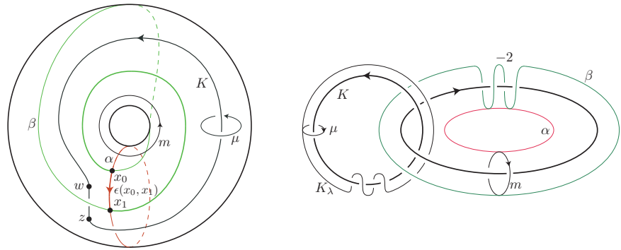
Figure 6. Surgery diagram of lens space L(5, 2)
