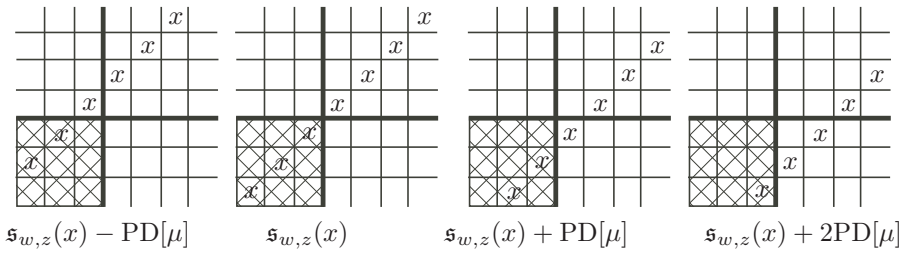
Figure 7. CFK^\infty(Y, K)
