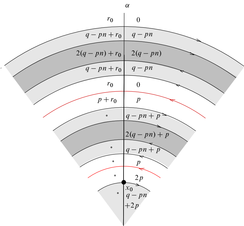
Figure 3: A 2-fold finger and the multiplicities of the periodic domain \mathcal{P}_n given by equation (5). (The case P = 3 , n = 2 is illustrated.) The meridian \beta is shown in black, the longitude \lambda in red. (The dots in the bottom regions to the left of \alpha replace the multiplicities that are not shown to save space. The multiplicities in these regions differ by r_0 from the multiplicities in the corresponding regions to the right of \alpha .) When n is large, the multiplicities inside the finger are smaller than the multiplicities outside, and the multiplicities increase as we move towards the center of the \lambda -spiral in Figure 2.
