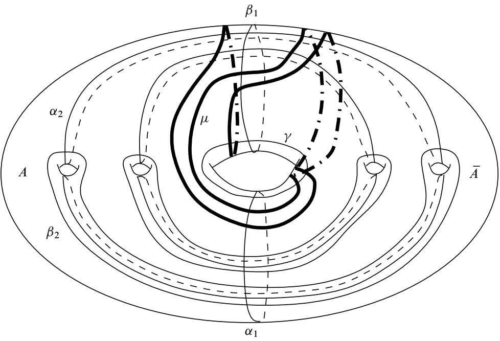
Figure 5: Constructing a Heegaard diagram from rational open book. The figure shows the Heegaard diagram arising form the open book with trivial monodromy. (To avoid overloading the picture, we have not drawn some of the \alpha -curves here. The missing curves lie in the back of the surface, in the top part of the diagram.) For a general open book, the \beta -curves in the \bar{A} region will be affected by the action of the open book monodromy (this is not shown in the figure).
