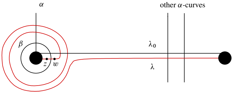
Figure 1: A diagram (\Sigma, \alpha, \beta, w, z) for the knot K . The meridian \beta , the longitude \lambda_0 , and the n -framed longitude \lambda are shown. (Here, n = 2 .) Note that \lambda_0 is drawn with a shift to make the figure clearer (both \lambda and \lambda_0 must pass through w and z ).
