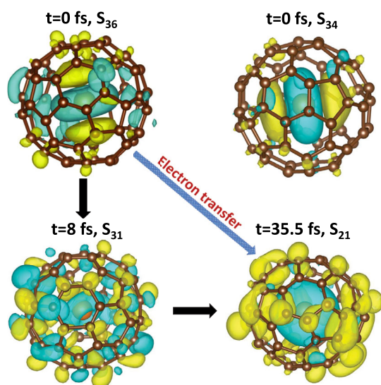
FIG. 4. Electron density difference (excited minus ground) of \text{Mg}@C_{60} with isodensity value of \pm 0.0005 a.u. with positive (golden) and negative (green) values. Results at t = 0 for S_{36} and S_{34} , and the electron transfer for S_{36} in a molecular dynamics trajectory, are shown.
