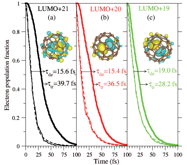
FIG. 2. Time evolutions of the decay and transfer population fractions after three initial excitations to (a) \text{LUMO}+21 , (b) \text{LUMO}+20 , and (c) \text{LUMO}+19 , corresponding to \text{Mg } 3p threefold degenerate orbitals. The decay ( \tau_{de} ) and transfer ( \tau_{tr} ) times shown are extracted by curve fittings (see text) and the fit curves for the decay are shown by the dashed lines.
