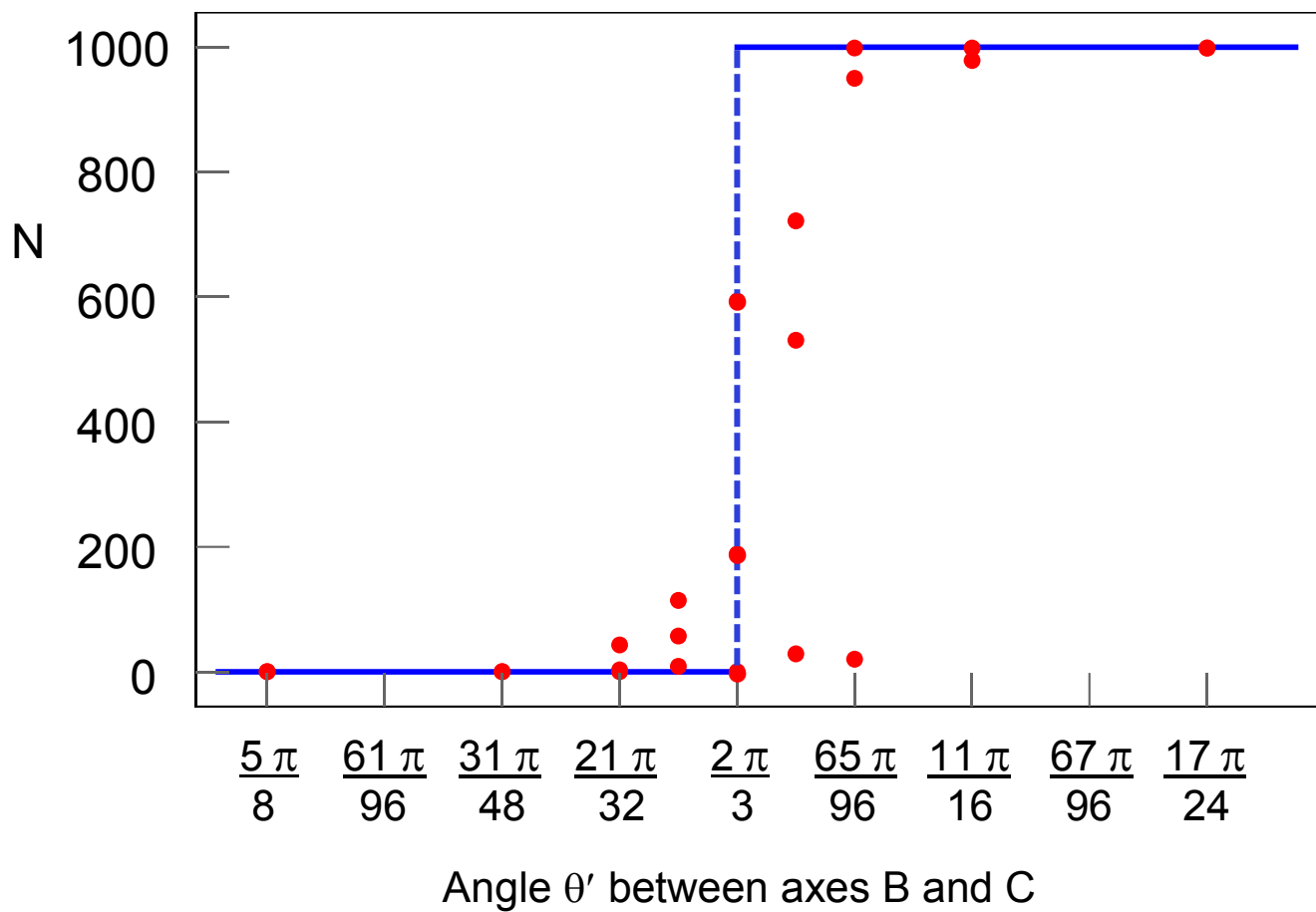
Figure 7. Number of cases where the quantum computer gave negative values of \Delta , out of 1000 cases generated by taking all possible combinations of 10 runs at each of the pairs of angles (A, B), (B, C), and (A, C). Results from multiple calculations are plotted as a function of the angle \theta' between axes B and C. Calculations run on the IBM ourense 135 quantum computer.
