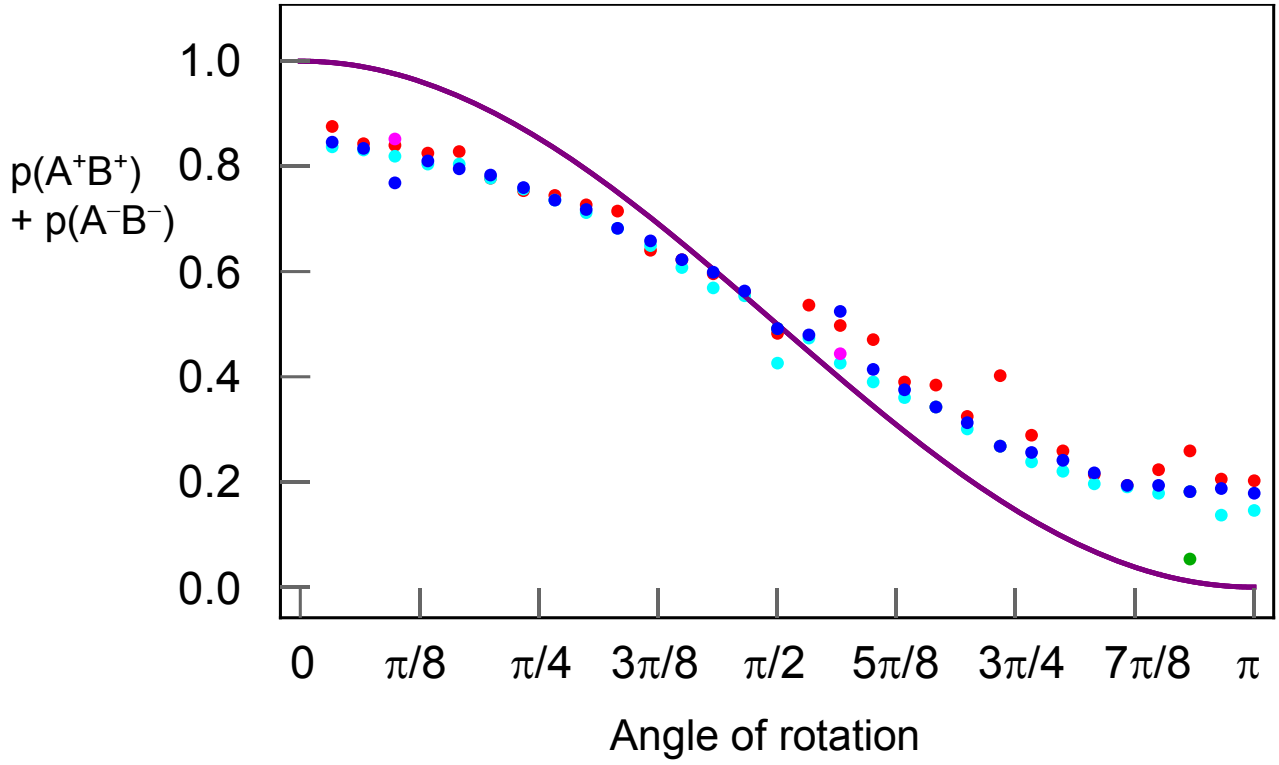
Figure 3. Values of p(A^+B^+) + p(A^-B^-) for the Bell states plotted as a function of \theta , from sets of ten runs each on the burlington quantum computer 131 with 1024 shots (in red), 4096 shots (in cyan), and 8192 shots (in blue). Where outliers were observed in the initial runs, the outcomes of repeat runs are shown in green or magenta (see text for details). Purple curve: quantum mechanical prediction.
