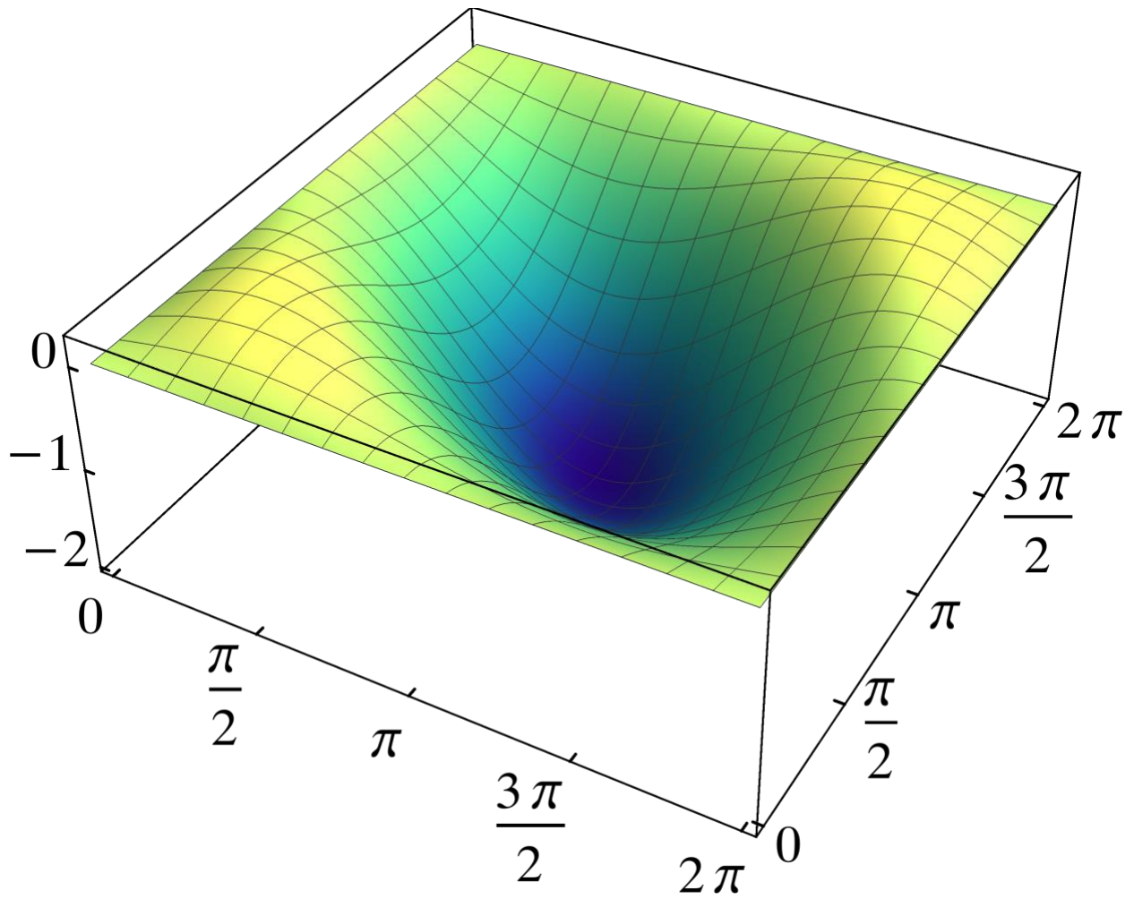
Figure 2a. Plot of the function f(\theta, \theta') \equiv \cos^2(\theta/2) - \cos^2[(\theta + \theta')/2] - \sin^2(\theta'/2) , as \theta and \theta' range from 0 to 2\pi .
