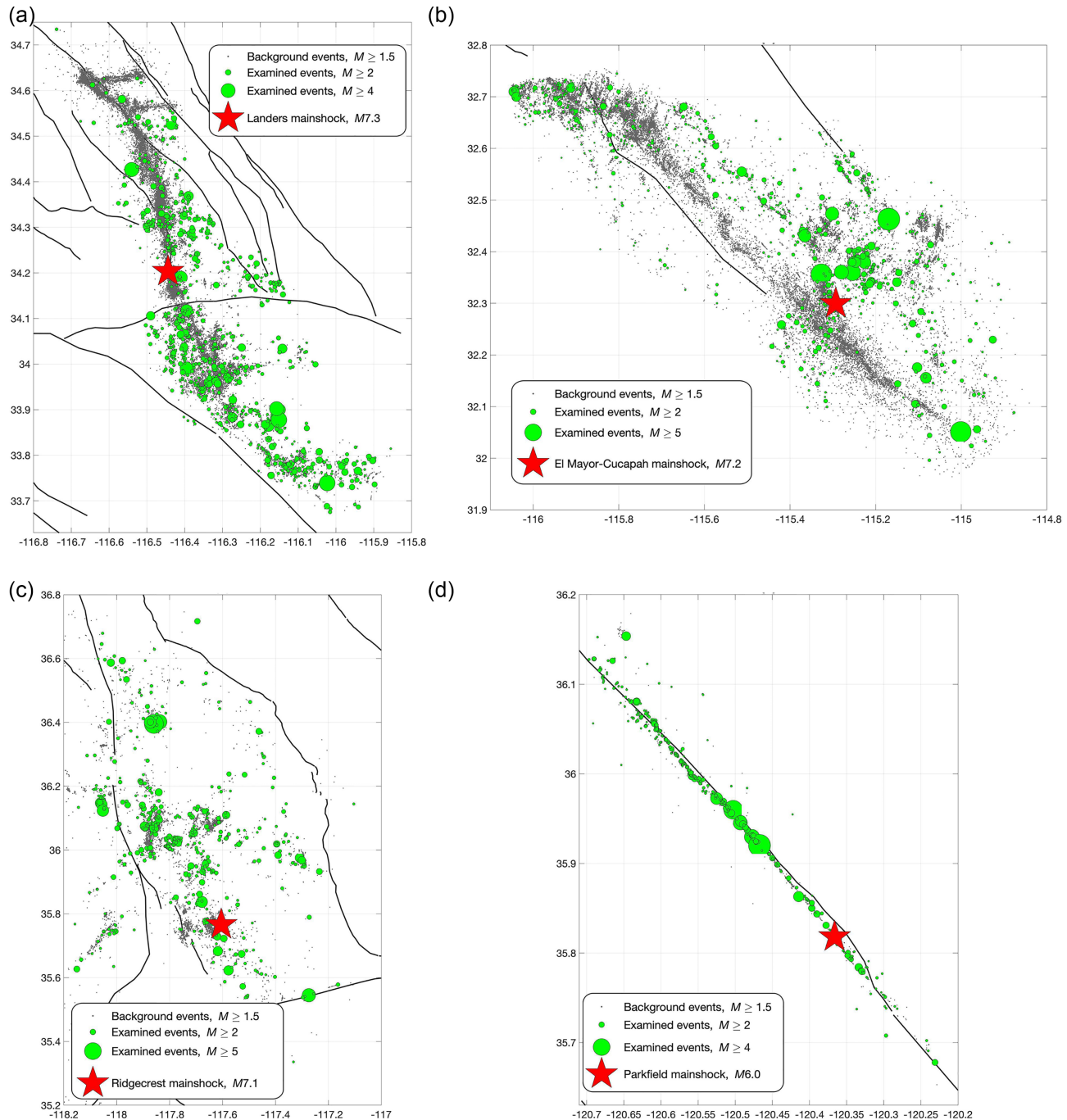
Figure 8. Regions examined for localization of background seismicity before large earthquakes in Figs 9 and 10. (a) Landers, M7.3. (b) El Mayor-Cuapah, M7.2. (c) Ridgecrest, M7.1. (d) Parkfield, M6. The analysis parameters are listed in Table 1.
