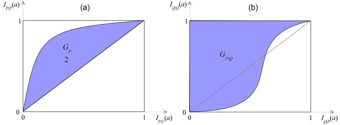
Figure A2. Statistics used to quantify localization of measure P(x) . (a) Absolute localization of P(x) is quantified by the Gini coefficient G_P (twice the shaded area) calculated for the set R(P|U, P) , which is shown by the curve above the diagonal. (b) Relative localization of P(x) with respect to measure Q(x) is quantified by the coefficient G_{P|Q} (the shaded area) calculated for the set R(Q|P, Q) , which is shown by the curve that wanders about the diagonal.
