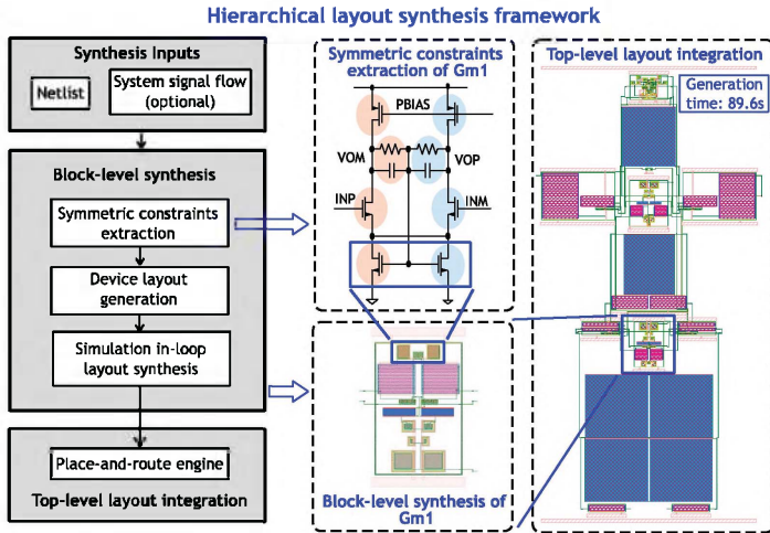
Fig. 1. The proposed hierarchical layout synthesis framework.
