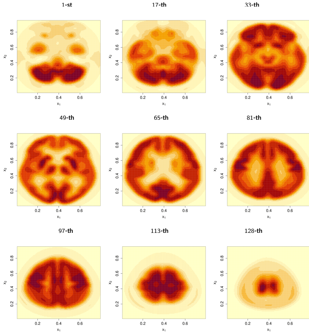
FIGURE 4 Recovered higher resolutions of selected nine slices in 3D case.
