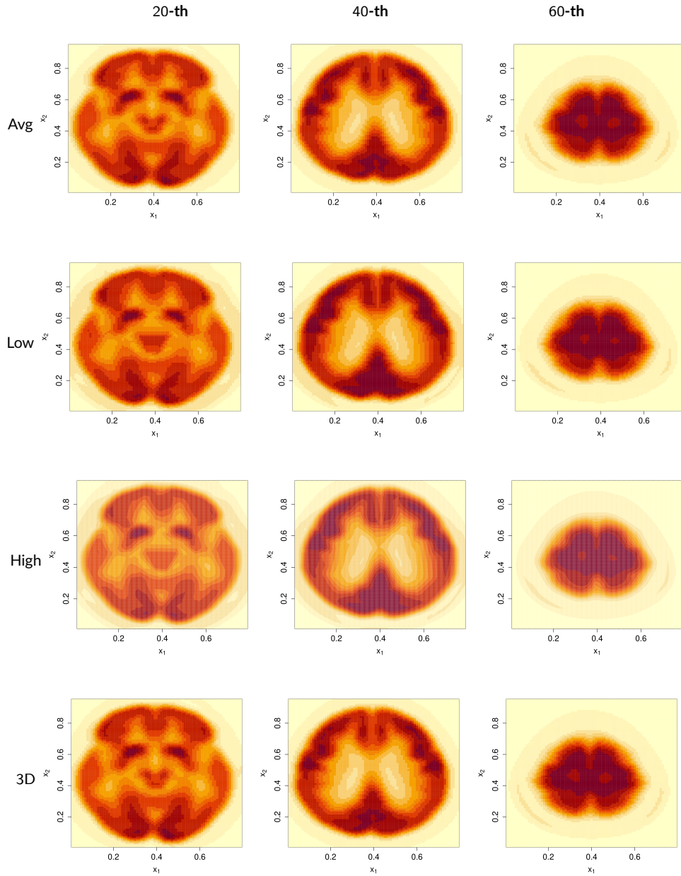
FIGURE 3 From top to bottom are averaged images \{\bar{Y}_{\cdot j}\}_{j=1}^{7505} , recovered images \hat{f}(x_{1j}, x_{2j'}) , j = 1, \dots, 79 , j' = 1, \dots, 95 , recovered high resolution ( 128 \times 128 ) images \hat{f}(x_{1j}, x_{2j}) , j = 1, \dots, 128 and recovered images from 3D image. Left: The 20-th slices; Middle: The 40-th slices; Right: The 60-th slices.
