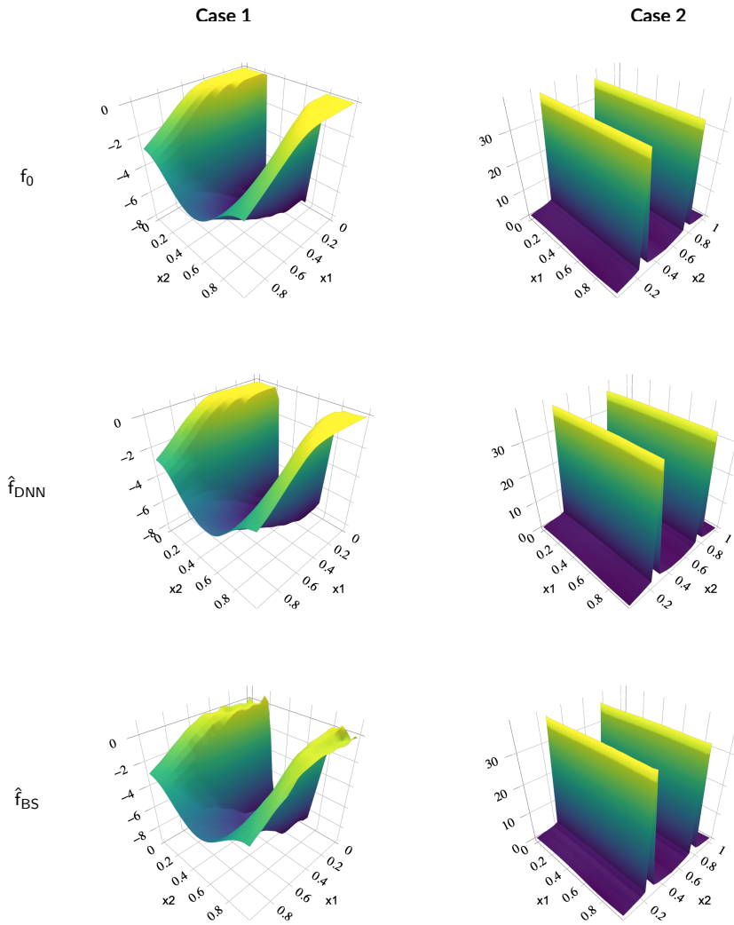
FIGURE 1 2D simulation. Left: from the top to bottom, they are true function f_0 (Case 1) and its estimators \hat{f}_{DNN} and \hat{f}_{BS} . Right: from the top to bottom, they are true function f_0 (Case 2) and its estimators \hat{f}_{DNN} and \hat{f}_{BS} . ( n = 200 , N = 625 and \sigma = 1 )
