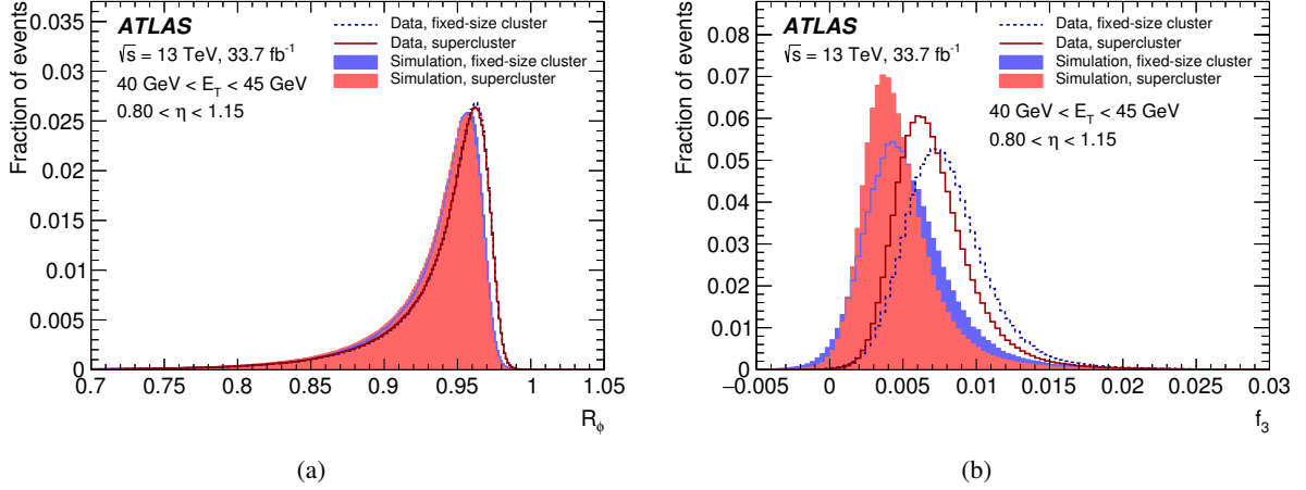
Figure 15: The distributions of (a) R_\phi and (b) f_3 obtained from 33.7 \text{ fb}^{-1} of data recorded in 2016 at \sqrt{s} = 13 TeV and simulation for prompt electrons that satisfy 40 < E_T < 45 GeV and 0.80 < |\eta| < 1.15 . The variables are shown for fixed-size EM clusters and superclusters. The detector simulation of the corresponding distributions is performed with the GEANT4 versions 4.9.6 and 4.10, respectively. The distributions for both the simulation and the data are obtained using the Z \rightarrow ee tag-and-probe method and KDE smoothing has been applied.
