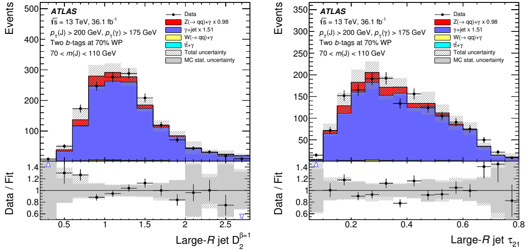
Figure 20: Z \rightarrow b\bar{b} candidate D_2^{\beta=1} and \tau_{21} distributions after requiring the Z \rightarrow b\bar{b} candidate jet mass to be between 70 and 110 GeV. Events with two b -tagged track-jets are used. The \gamma +jets background and the Z \rightarrow b\bar{b} signal are normalised to data by applying a scale factor of 1.51 and 0.98, respectively. The upward- or downward-pointing arrows indicate that the Data/Fit ratio is out of the histogram range for these bins.
