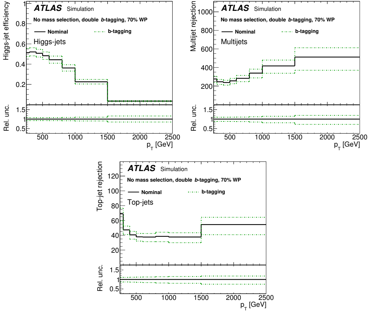
Figure 2: The Higgs-jet efficiency (top left) and rejection against multijet (top right) and top-jet backgrounds (bottom) as a function of the jet p_T for the 70% double- b -tagging working point. The nominal curves correspond to the requirement on the MV2c10 discriminant described in Section 6.2. The b -tagging-related uncertainties defined in Section 5 are shown.
