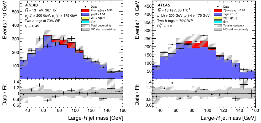
Figure 19: Z \rightarrow b\bar{b} candidate jet mass after applying the \tau_{21} < 0.45 (left) or D_2^{\beta=1} < 1.3 (right) requirement. Events with two b -tagged track-jets are used. The \gamma +jets background and the Z \rightarrow b\bar{b} signal are normalised to data by applying a scale factor of 1.51 and 0.98, respectively.
