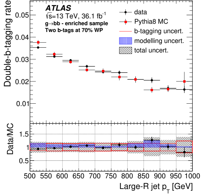
Figure 16: Comparison of data and MC simulation double- b -tagging rates as a function of the large- R jet p_T . The flavour-tagging correction factors and the flavour-fit corrections have been applied. The two largest systematic uncertainties, generator modelling and the b -tagging-related uncertainties, are shown as well. The total uncertainty includes all systematic uncertainties listed in Section 5 and the fit uncertainty summed in quadrature. The size of the flavour-fit uncertainty is below 1%.
