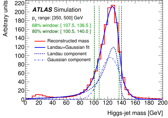
Figure 4: The Higgs-jet mass distribution for jet transverse momenta in the range 350 to 500 GeV after reweighting the p_T spectrum. The dotted and dash-dotted blue curves correspond to the two components of the fit function, while the solid blue curve shows the combination thereof. The vertical lines indicate the boundaries of the mass ranges for 68% (light green) and 80% (dark green) containment.
