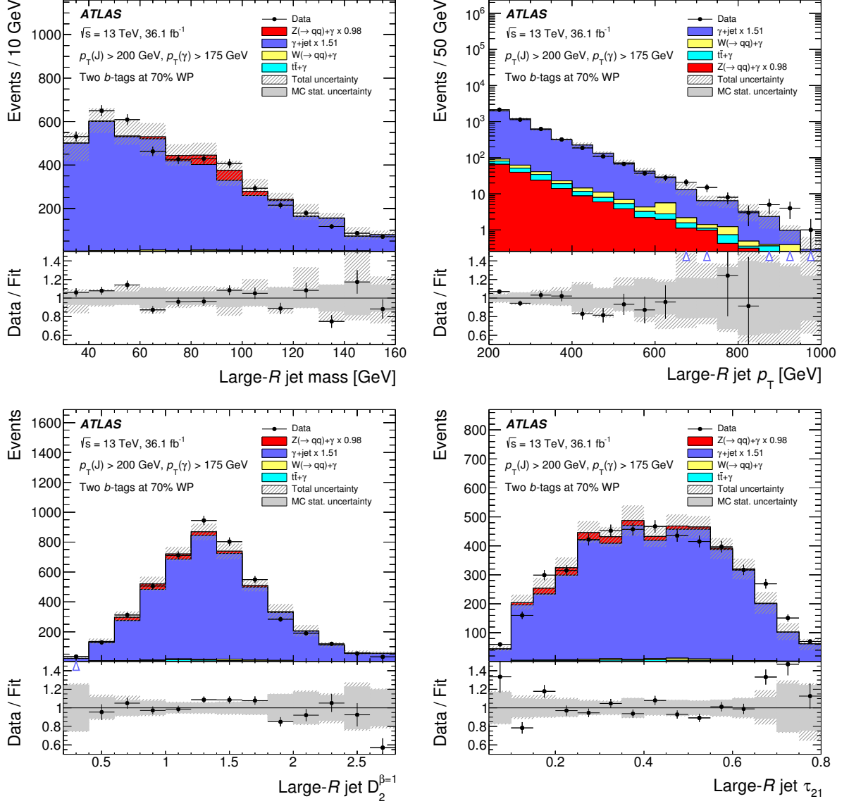
Figure 18: Jet mass, p_T , D_2^{\beta=1} and \tau_{21} distributions. Events with two b -tagged track-jets are used. The \gamma + jets background and the Z \rightarrow b\bar{b} signal are normalised to data by applying a scale factor of 1.51 and 0.98, respectively. The upward- or downward-pointing arrows indicate that the Data/Fit ratio is out of the histogram range for these bins.
