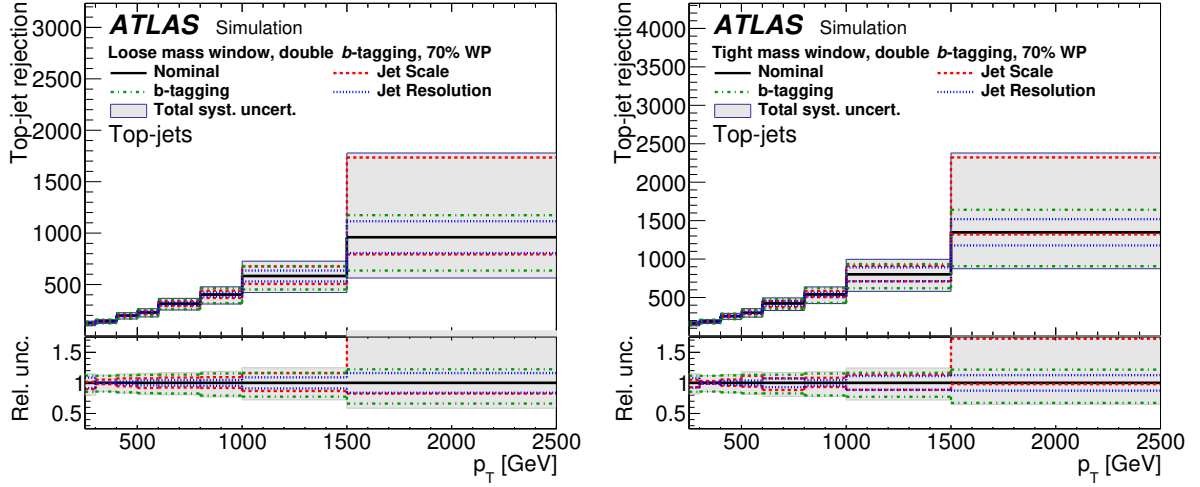
Figure 9: Rejection of the top-jet background as a function of the Higgs-jet p_T for the loose (left) and tight (right) mass window requirements, in combination with the 70% double- b -tagging working point. The nominal curves correspond to the requirement on the MV2c10 discriminant described in Section 6.2. Systematic uncertainties defined in Section 5 as well as their sum in quadrature (total uncertainty) are shown. ‘Jet Scale’ refers to the sum in quadrature of the jet energy and mass scale uncertainties and ‘Jet Resolution’ refers to the sum in quadrature of the jet energy and mass resolution uncertainties.
