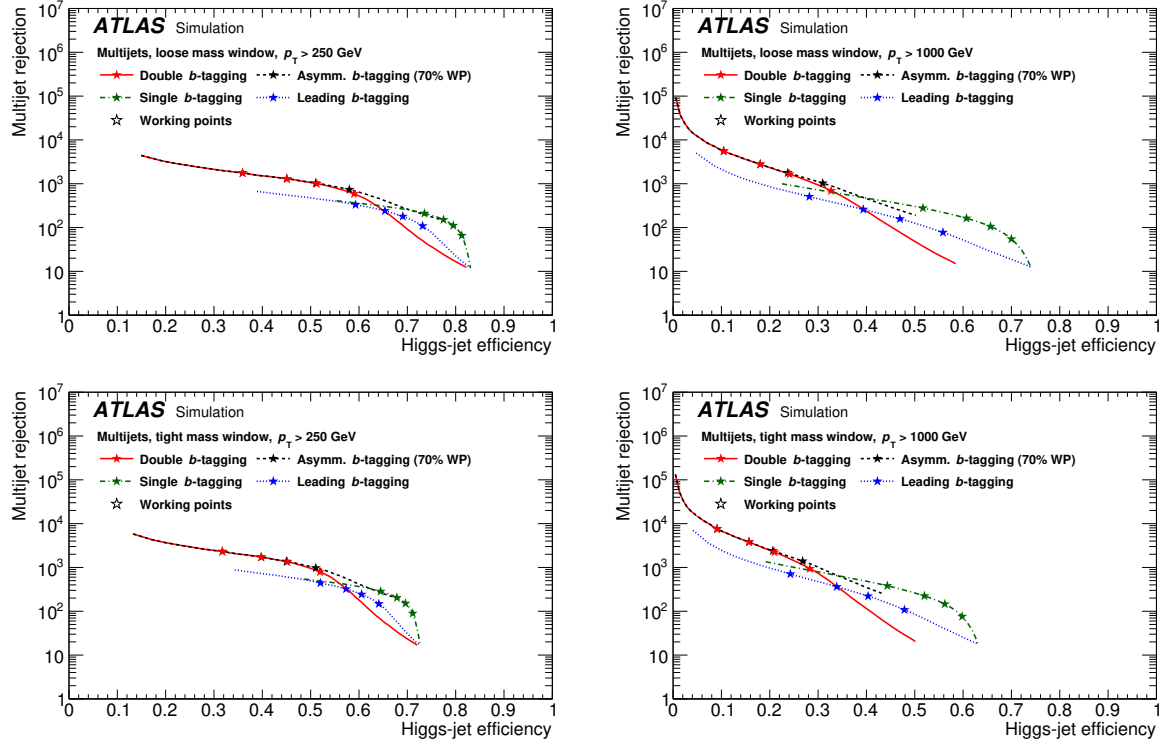
Figure 8: Rejection of multijet background as a function of the Higgs boson tagging efficiency for loose (top) and tight (bottom) mass window requirements for large- R jet p_T above 250 GeV (left) and above 1000 GeV (right) for various b -tagging benchmarks. The stars correspond to the 60%, 70%, 77% and 85% b -tagging WPs (from left to right). The curves for the double- and asymmetric- b -tagging working points coincide over a large range of Higgs-jet efficiency.
