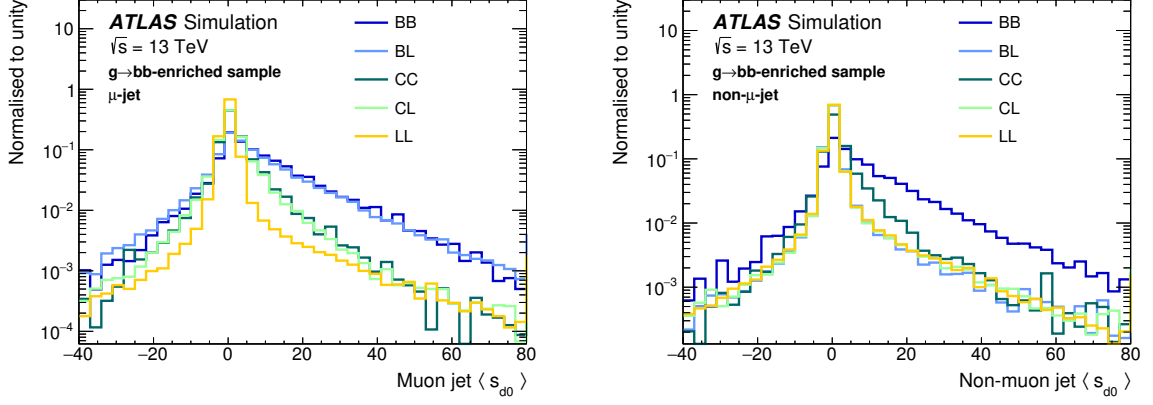
Figure 13: Averaged impact parameter significance, \langle s_{d_0} \rangle , distributions for the muon (left) and non-muon jets (right) inclusive in j_{\mu}^{\text{trk}} and j_{\text{non-}\mu}^{\text{trk}} transverse momenta. The double flavour labels denote the true flavour of the jet pair, with the j_{\mu}^{\text{trk}} given first.
