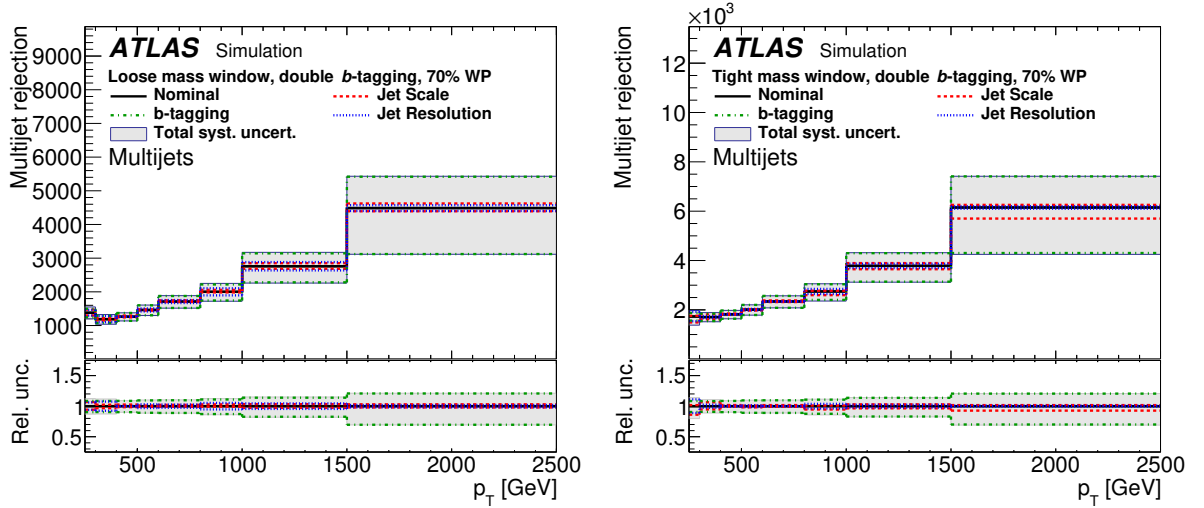
Figure 7: Rejection of multijet background as a function of the Higgs-jet p_T for the loose (left) and tight (right) mass window requirements, in combination with the 70% double- b -tagging working point. The nominal curves correspond to the requirement on the MV2c10 discriminant described in Section 6.2. Systematic uncertainties defined in Section 5 as well as their sum in quadrature (total uncertainty) are shown. ‘Jet Scale’ refers to the sum in quadrature of the jet energy and mass scale uncertainties and ‘Jet Resolution’ refers to the sum in quadrature of the jet energy and mass resolution uncertainties.
