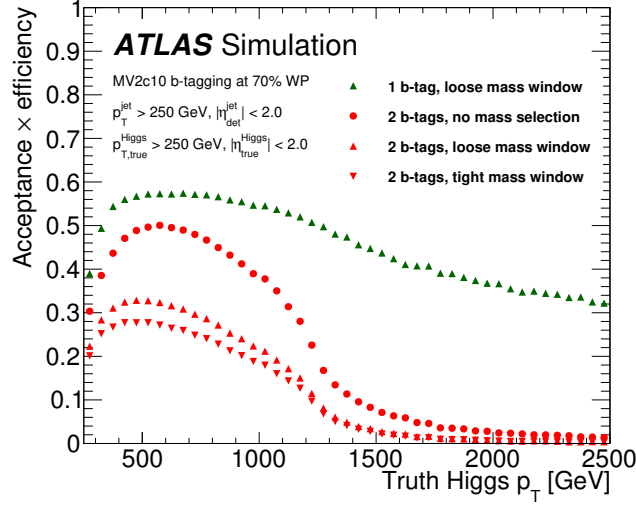
Figure 6: The Higgs boson acceptance times efficiency is shown for a few working points: the double and single b -tagging with the loose mass window requirement and the double b -tagging with the tight, loose and no mass window requirements.
