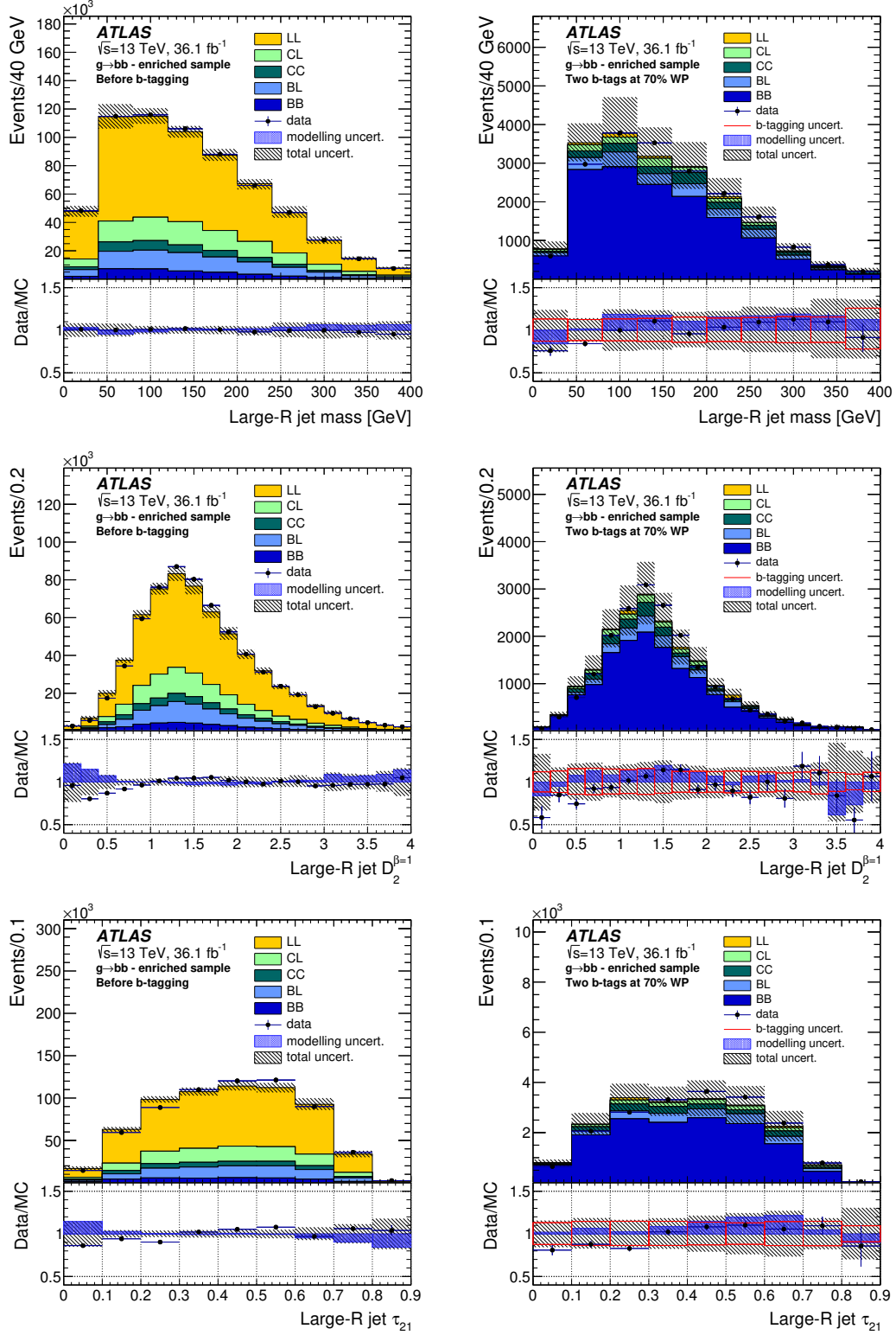
Figure 17: Distributions of large- R jet mass (top), D_2^{\beta=1} (middle) and \tau_{21} (bottom) before (left) and after (right) double b -tagging. The flavour-tagging correction factors and the flavour-fit corrections have been applied. The two largest systematic uncertainties, generator modelling and the b -tagging-related uncertainties, are shown as well. The total uncertainty includes all systematic uncertainties listed in Section 5 and the fit uncertainty summed in quadrature. The D_2^{\beta=1} and \tau_{21} uncertainty bands include additional substructure variable uncertainties [48].
