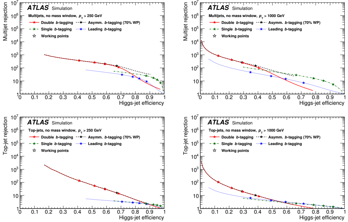
Figure 3: The multijet (top) and the top-jet (bottom) rejection as a function of the Higgs tagging efficiency for large- R jet p_T above 250 GeV (left) and above 1000 GeV (right) for various b -tagging benchmarks defined in Section 6.2. The stars correspond to the 60%, 70%, 77% and 85% b -tagging WPs (from left to right). The curves for the double- b -tagging and asymmetric- b -tagging working points coincide over a large range of Higgs-jet efficiency.
