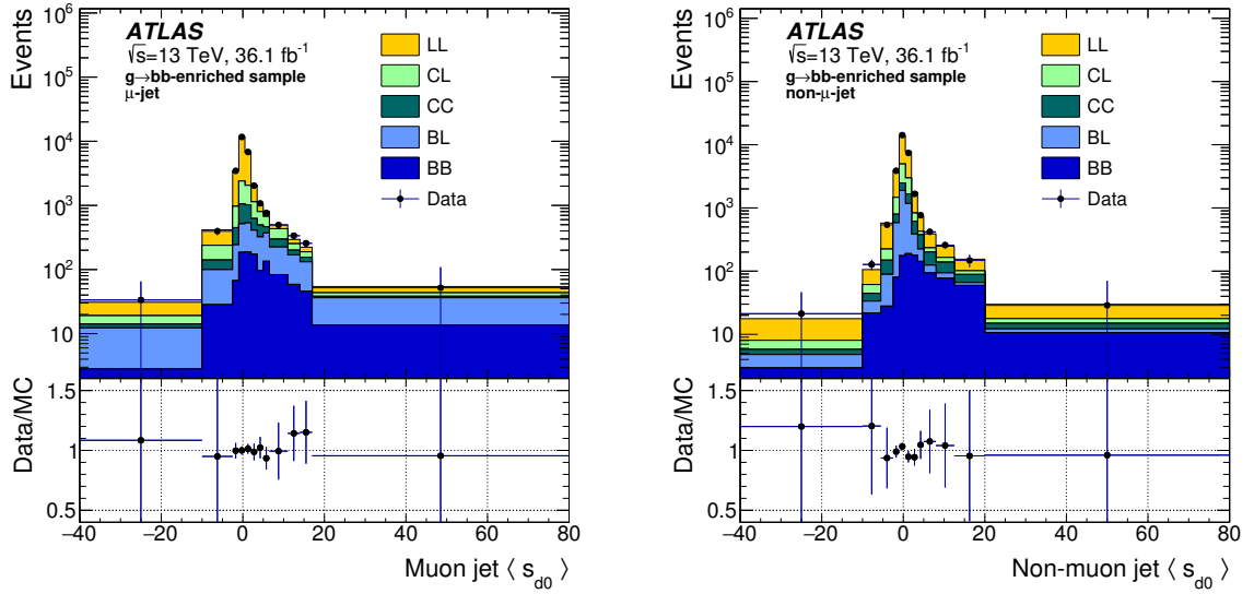
Figure 14: Averaged impact parameter significance, \langle s_{d_0} \rangle , distributions of the muon (left) and non-muon jet (right) in the (100–200) GeV bin of the j_{\mu}^{\text{trk}} and j_{\text{non-}\mu}^{\text{trk}} transverse momenta.
