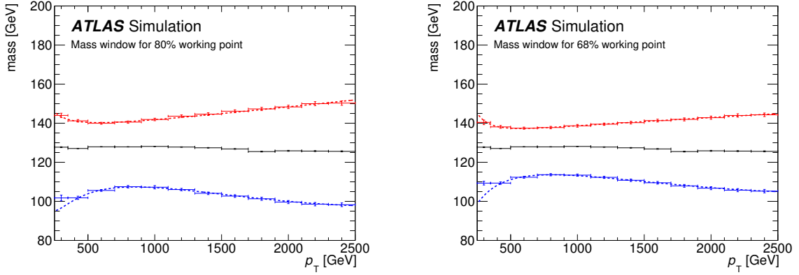
Figure 5: The Higgs-jet mass window interval for a loose (left) and a tight (right) working point. The dashed lines show a fit to the derived intervals (blue and red markers) as a function of the Higgs-jet p_T . The black markers show the position of the maximum of the Higgs-jet mass distribution.
