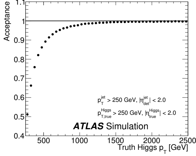
Figure 1: Fraction of Higgs bosons in simulation which are reconstructed and labelled as a Higgs-jet following the definition in Section 4, as a function of Higgs boson p_T . Only Higgs bosons with p_T > 250 GeV, |\eta| < 2.0 and with associated b -hadrons from its decay are considered. Same p_T and \eta requirements are applied to the Higgs-jets.
