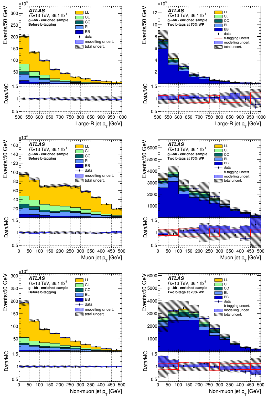
Figure 15: Transverse momentum distributions of the large- R jet (top), j_{\mu}^{\text{trk}} (middle) and j_{\text{non-}\mu}^{\text{trk}} (bottom) before (left) and after (right) double b -tagging. The flavour-tagging correction factors and the flavour-fit corrections have been applied. The two largest systematic uncertainties, generator modelling and the b -tagging-related uncertainties, are shown as well. The total uncertainty includes all systematic uncertainties listed in Section 5 and the fit uncertainty summed in quadrature.
