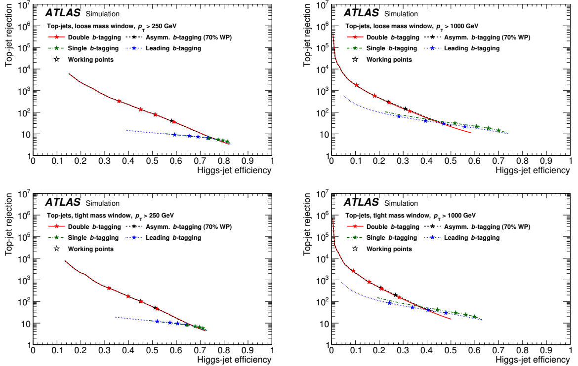
Figure 10: Rejection of the top-jet background as a function of the Higgs tagging efficiency for loose (top) and tight (bottom) mass window requirements for large- R jet p_T above 250 GeV (left) and above 1000 GeV (right) for various b -tagging benchmarks. The stars correspond to the 60%, 70%, 77% and 85% b -tagging WPs (from left to right). The curves for the double- and asymmetric- b -tagging working points coincide over a large range of Higgs-jet efficiency.
