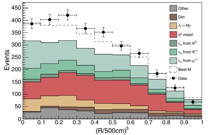
FIG. 22. The MiniBooNE radial vertex distribution, corresponding to the total 18.75 \times 10^{20} POT data in neutrino mode in the 200 < E_\nu^{\text{QE}} < 1250 MeV energy range, for \nu_e CCQE data (points with statistical errors) and background (histogram). The dashed histogram shows the best fit to the neutrino-mode data assuming two-neutrino oscillations.
