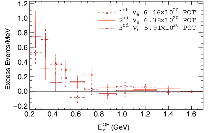
FIG. 10. The total event excesses in neutrino mode as a function of E_\nu^{\text{QE}} for the first, second, and third running periods. Error bars include only statistical uncertainties.
