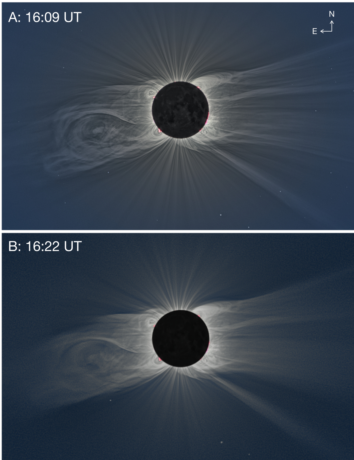
Figure 1. (A) White-light data from the 2020 December 14 TSE from N  uquen, Argentina, at 16:09 UT (see Section 2). Solar cardinal directions are noted in the top right corner. An animation of the CME propagation during the eclipse at N  uquen from 16:08:37 to 16:09:58 UT is available. The realtime duration of the video is 7 s. (B) Same as A, but from R  o Negro, Argentina, at 16:22 UT. These images have been processed to enhance fine-scale structures and are not in absolute units. (An animation of this figure is available.)
