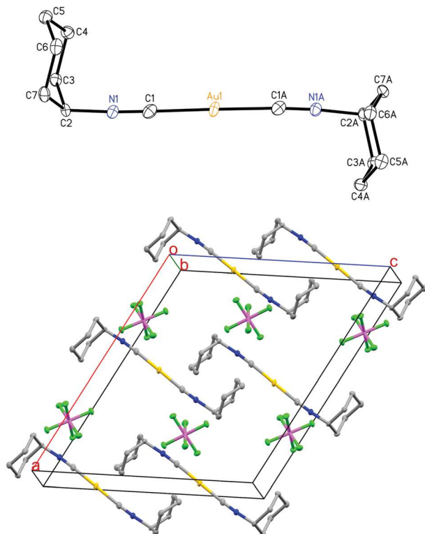
Fig. 1 Top, the structure of the cation in non-luminescent [(C_6H_{11}NC)_2Au]PF_6 ( 3 ). Bottom, crystal packing structure of the non-luminescent [(C_6H_{11}NC)_2Au]PF_6 ( 3 ) showing the lack of auriphilic interactions. The closest Au(I)–Au(I) contact is 7.985 Å. Atom colors: gold, yellow; carbon, grey; nitrogen, blue; phosphorus, violet; fluorine, green.
