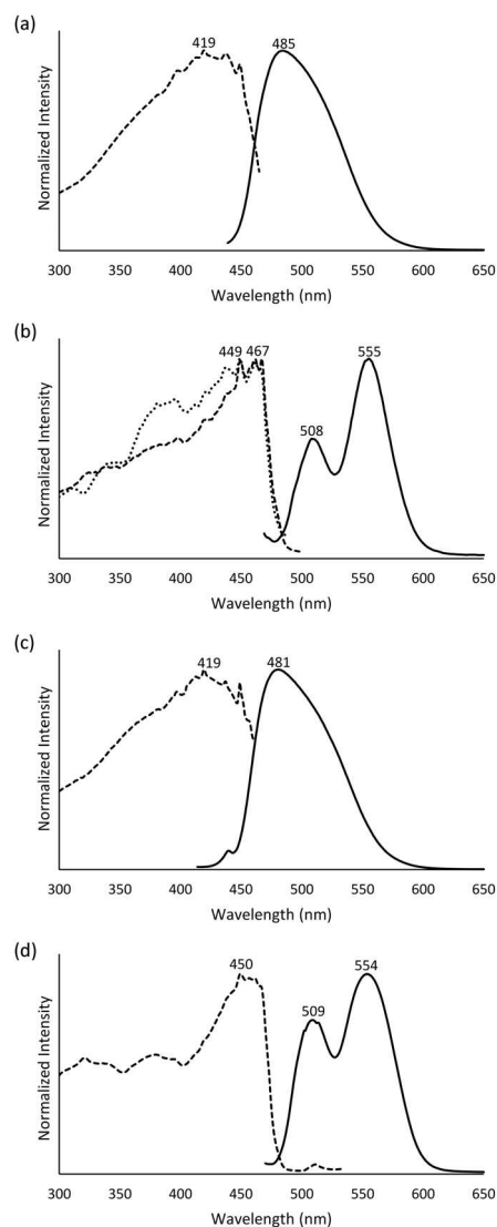
Fig. 3 The luminescence spectra of non-luminescent [(C_6H_{11}NC)_2Au]PF_6 ( 3 ) after grinding (final color and luminescence: yellow and green, respectively). (a) Excitation (dashed) and emission (solid) spectra at 298 K. (b) Excitation (dotted) and emission (solid) spectra at 77 K. These spectra are consistent with the formation of green luminescent [(C_6H_{11}NC)_2Au]PF_6 ( 1 ) upon grinding. The excitation (dashed) and emission (solid) spectra of green luminescent [(C_6H_{11}NC)_2Au]PF_6 ( 1 ) are shown in (c) at 298 K and (d) at 77 K.
