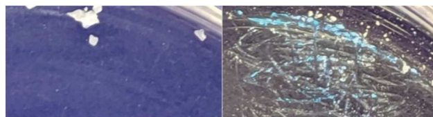
Fig. 2 Left, a photograph, taken under UV and ambient light, showing colorless crystals of the non-luminescent [(C_6H_{11}NC)_2Au]PF_6 ( 3 ). Right, a photograph, taken under UV light, showing the luminescence of the crystals of ( 3 ) after they were ground using a glass stir rod.
