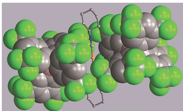
Fig. 3 Two (\text{BARF}_{24})^- anions (drawn with space-filling contours) surrounding a [(\text{C}_6\text{H}_{11}\text{NC})_2\text{Au}]^+ cation in (6). Atom colors are: Au, orange; C, grey; N, blue; B, pink; F, green.
