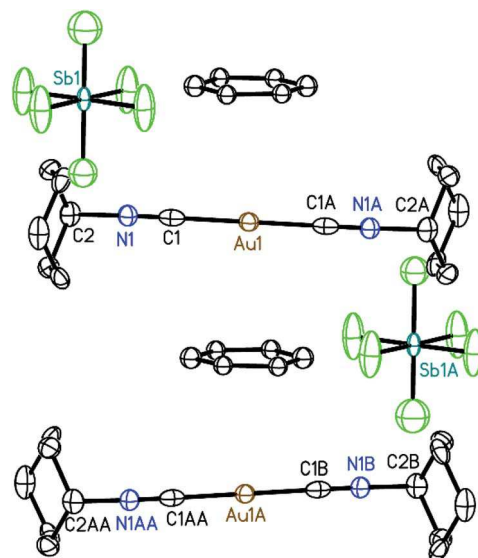
Fig. 5 A portion of the structure of [(\text{C}_6\text{H}_{11}\text{NC})_2\text{Au}](\text{SbF}_6) \cdot \text{C}_6\text{H}_6 (7) that depicts the sandwich of benzene between two of the gold(I) cations with 50% thermal contours. Hydrogen atoms and the alternate position for the benzene molecules are omitted for clarity.
