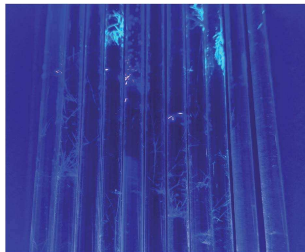
Fig. 4 Spatially separated formation of crystals from a benzene solution of [(\text{C}_6\text{H}_{11}\text{NC})_2\text{Au}](\text{AsF}_6) with diethyl ether layered on top in 5 mm outside diameter glass tubes. The photograph was taken under UV irradiation. The non-luminescent crystals of [(\text{C}_6\text{H}_{11}\text{NC})_2\text{Au}](\text{AsF}_6) \cdot \text{C}_6\text{H}_6 (8) are seen at the lower part of each tube. Above that the pink-tinged crystals are the colorless [(\text{C}_6\text{H}_{11}\text{NC})_2\text{Au}](\text{AsF}_6) (4), but the camera captures the emission color as pink rather than the blue seen by eye. Further up the tubes are crystals of the yellow [(\text{C}_6\text{H}_{11}\text{NC})_2\text{Au}](\text{AsF}_6) (3), which glow green.
