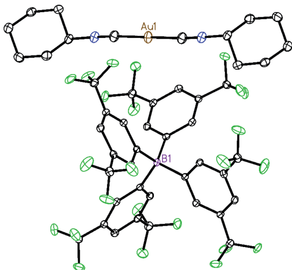
Fig. 2 The structure of [(\text{C}_6\text{H}_{11}\text{NC})_2\text{Au}](\text{BARF}_{24}) (6) with 50% thermal contours. Hydrogen atoms are omitted for clarity. Atom colors are: Au, orange; C, grey; N, blue; B, pink; F, green.
