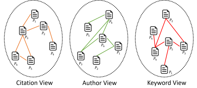
Figure 1: An illustrative network example of 3 views with 6 papers. In the citation view, an edge connects two papers if one paper cites the other. In the author view, an edge exists if two papers share at least one common author. In the keyword view, an edge exists if two papers share at least one common keyword.
