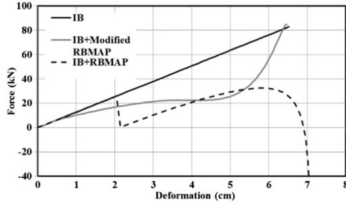
Figure 1.7: Simulated force-displacement profiles of an isolated bridge (IB), the bridge equipped with the RMAP, and the bridge equipped with the modified RMAP; Source: Attary et al. (2017)
