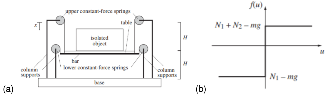
Figure 1.11: (a) Schematic of piecewise-constant restoring force vertical isolator and (b) force-deflection profile of the isolator about its static equilibrium position; Source: Araki et al. (2009)
