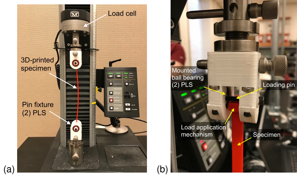
Figure A.4: Images of the experimental setup (a) and pin fixture (b).
