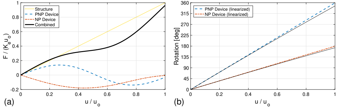
Figure 2.2: (a) Theoretical normalized load-deflection relation of an SNSD in parallel with a linear-elastic structure having stiffness K_e . (b) The associated rotations in the PNP and NP devices based on Eq. (2.8), with the nonlinear relationships (—) given by Eq. (2.6) for comparison
