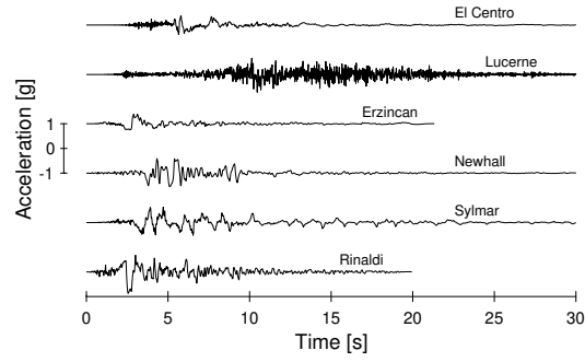
Figure 2.11: Historic ground motion time histories (unscaled).
