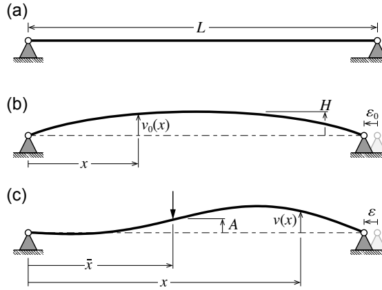
Figure 3.2: Geometry and description of a buckled strut: (a) an initially undeformed strut of length L ; (b) the strut after an end shortening of \varepsilon = \varepsilon_0 resulting in the initial deflected shape v_0(x) with lateral rise H ; (c) the strut when a lateral constraint is enforced such that v(\bar{x}) = A .
