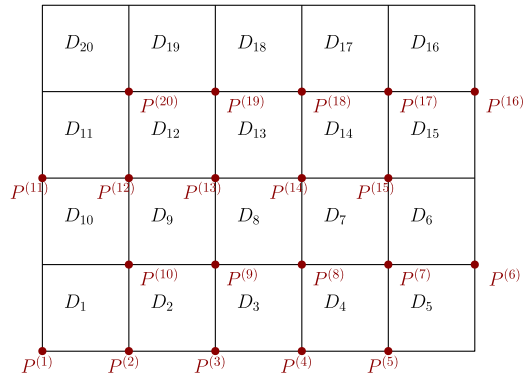
Figure 1. An example of the domain.
