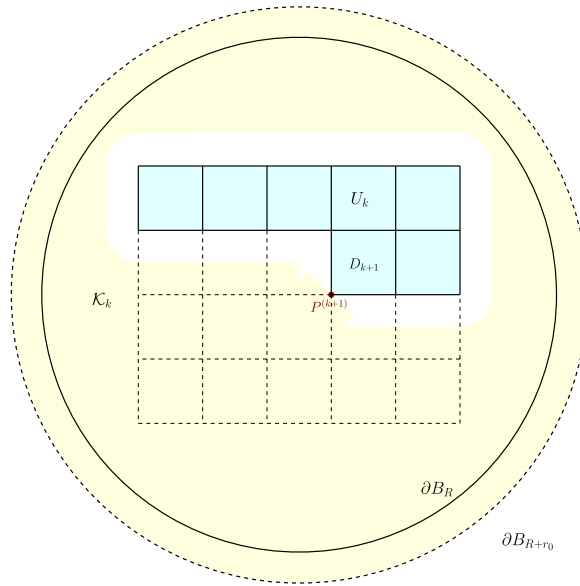
Figure 4. The domains U_k and K_k for k = 13 .
