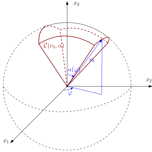
Figure 2. Illustration of \mathcal{C}(r_0, \alpha) .
