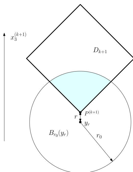
Figure 5. The shaded region is B_{r_0}(y_r) \cap D_{k+1} .
