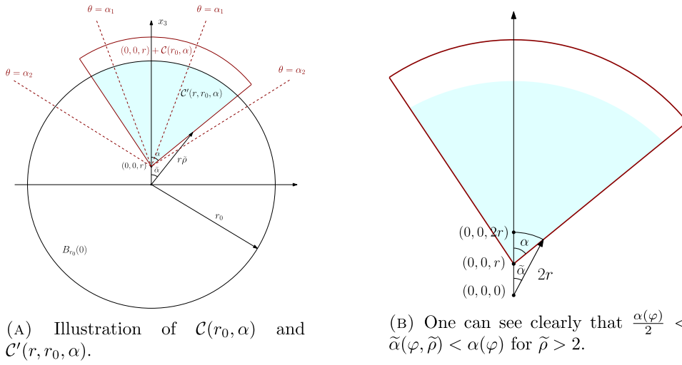
Figure 3. Illustrations of the domains defined.
