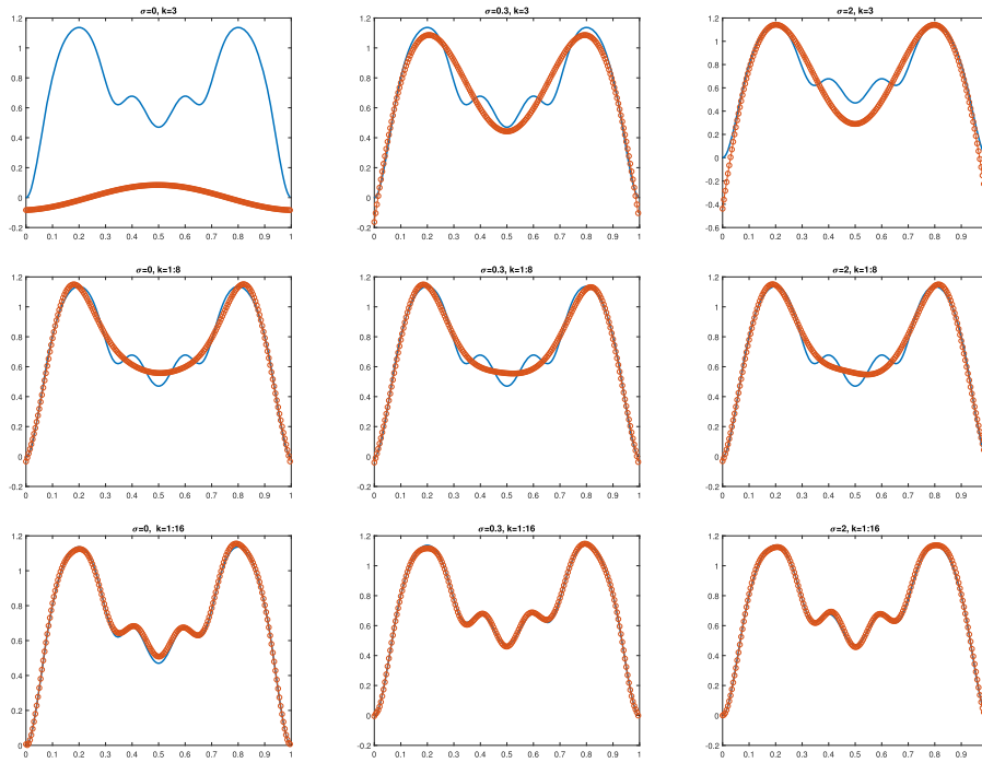
Figure 3. Reconstruction of the strength in example 3. Solid blue line: exact strength; circled red line: reconstructed strength. For \sigma = 0 (left column), \sigma = 0.3 (middle column) and \sigma = 2 (right column), reconstructions get better when data at more frequencies are used (top: k = 3 ; middle: k = 1, \dots, 8 ; bottom: k = 1, \dots, 16 ), and more frequencies are required to properly reconstruct the strength which contains more higher frequency modes.
