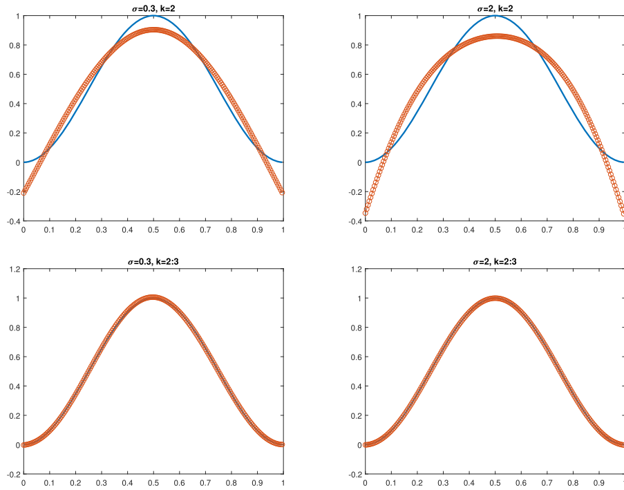
Figure 1. Reconstruction of the strength in example 1. Solid blue line: exact strength; circled red line: reconstructed strength. For both \sigma = 0.3 (left column) and \sigma = 2 (right column), reconstructions based on data at two frequencies k = 2, 3 are better than the ones based on data at a single frequency k = 2 .
