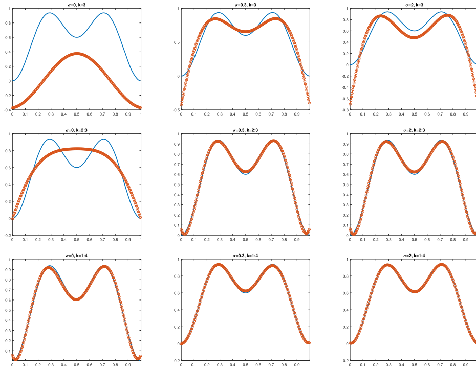
Figure 2. Reconstruction of the strength in example 2. Solid blue line: exact strength; circled red line: reconstructed strength. For \sigma = 0 (left column), \sigma = 0.3 (middle column) and \sigma = 2 (right column), reconstructions get better when data at more frequencies are used (top: k = 3 ; middle: k = 2, 3 ; bottom: k = 1 : 4 ).
