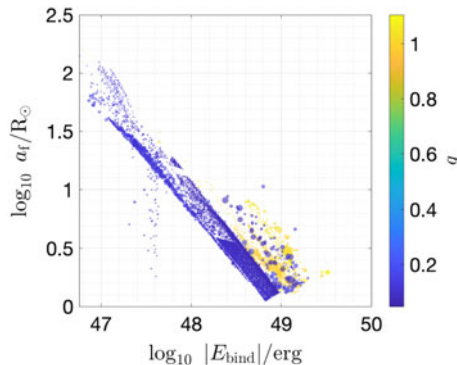
Figure 9. All DNS-forming binaries from our Fiducial model are shown here. We present the post-CEE separation a_t as a function of the absolute value of the envelope binding energy |E_{\text{bind}}| . For the double-core scenario, the binding energy is E_{\text{bind}} = E_{\text{bind,donor}} + E_{\text{bind,comp}} . The size of the marker indicates the sampling weight and its colour shows the mass ratio q . This Figure can be compared to Figures 1 and 2 from Iaconi & De Marco (2019). That study presents simulations of CE binaries and observations of post-CE binaries. Most systems presented here do not feature in Iaconi & De Marco (2019).
