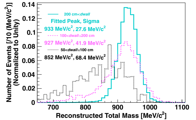
FIG. 2. Reconstructed total mass distribution for free proton decays via p \rightarrow e^+\pi^0 MC events with three rings. The solid cyan histogram shows events reconstructed in the conventional fiducial volume ( 200 \text{ cm} < d_{\text{wall}} ), the pink dashed histogram shows that for the additional fiducial volume ( 100 < d_{\text{wall}} \leq 200 \text{ cm} ) and the black dotted histogram is for the region between d_{\text{wall}} of 50 cm and 100 cm. Gaussian fits have been used to determine the mass peak and width.
