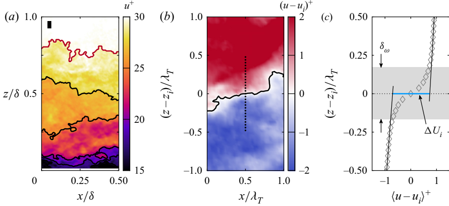
Figure 3. Example shear layers for the Re_\tau = 17\,000 smooth-wall case. (a) Streamwise velocity field from figure 2 of Heisel et al. (2020b), with detected ISLs (black lines) and turbulent/non-turbulent interface (red line). (b) Velocity field in the vicinity of an ISL (black line) relative to the ISL position z_i and velocity u_i . (c) Conditionally averaged velocity profile relative to the ISLs, indicating the average velocity difference \Delta U_i and thickness \delta_\omega . The black box in the upper left of (a) indicates the size of the field in (b).
