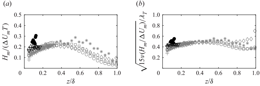
Figure 11. Wall-normal profiles of the turnover time estimated from average local UMZ properties H_m / \Delta U_m . (a) Compared with the large-eddy turnover time T . (b) Compared with the Taylor microscale \lambda_T based on the isotropic relationship \lambda_T \approx \sqrt{15\nu}T . Data symbols correspond to the experimental datasets in table 1.
