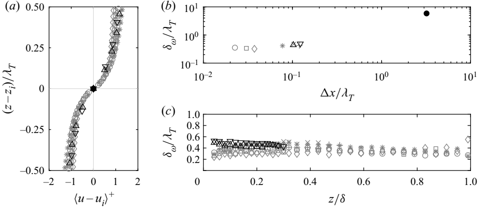
Figure 4. Estimated average thickness \delta_\omega of ISLs normalized by \lambda_T . (a) Conditional average profile of streamwise velocity relative to ISLs in the log region. (b) Thickness \delta_\omega as a function of measurement grid spacing \Delta x , noting the interrogation window size for the PIV cases is 2\Delta x . (c) Wall-normal profile of \delta_\omega . Data symbols correspond to the experimental datasets in table 1.
