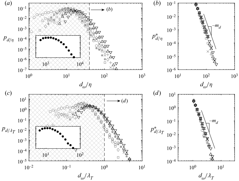
Figure 5. Probability distributions p_d of diameter for all prograde vortex cores in the outer layer of the boundary layer: (a) p.d.f. normalized by the Kolmogorov length scale \eta ; (b) conditional p.d.f. p_{d/\eta}^* = p_{d/\eta}(d_\omega | d_\omega > 40\eta) ; (c) p.d.f. normalized by the Taylor microscale \lambda_T ; (d) conditional p.d.f. p_{d/\lambda_T}^* = p_{d/\lambda_T}(d_\omega | d_\omega > \lambda_T) . Comparison of results in the hatched regions of (a,c) is precluded by variability in measurement resolution across cases, including the ASL case shown in the insets. The conditional p.d.f.s in (b,d) are used to evaluate the distribution tail shape parameterized by the slope m_d . Data symbols correspond to the experimental datasets in table 1 .
