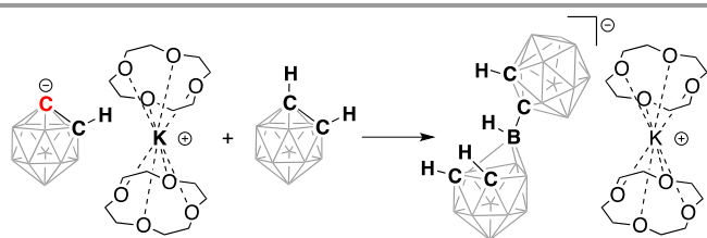
Scheme 4. Reaction of the strongly nucleophilic deprotonated free carboranyl anion with the parent protonated carborane cluster and the formation of the two-cage anion [C_4B_{20}H_{23}]^- . Unlabeled cluster vertices represent BH units.
