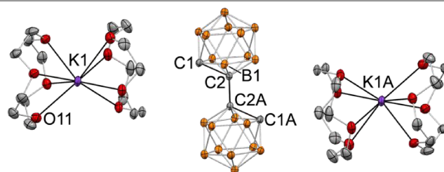
Fig. 5. Displacement ellipsoid plot (50% probability) of [\text{K}(12\text{-crown-4})]_2(\text{C}_2\text{B}_{10}\text{H}_{10})_2 \cdot 4(\text{THF}) ( 6 ). Note the lack of C...K contact and the complete ion separation. Only a half of the asymmetric unit is shown. Hydrogen atoms on the cluster and carbon atoms of the crown ether ligand have been omitted for clarity. Crystallization solvent molecules (THF) are not shown. Selected interatomic distances (Å): K1...C1 = 6.283(1), C1–C2 = 1.712(1), C1–B1 = 1.724(2), C2–B1 = 1.698(2), C2–C2A = 1.532(2) Å.
