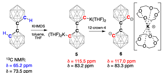
Scheme 3. Double deprotonation of 1,1'-bis( o -carborane) ( \text{C}_2\text{B}_{10}\text{H}_{11} ) 2 with potassium hexamethyldisilazide (KHMDS) and subsequent sequestration of potassium cations by the crown ether. Chemical shifts of the signals in the ^{13}\text{C} NMR spectra from carbon atoms of the parent and deprotonated clusters are listed. Unlabeled cluster vertices represent BH units.
