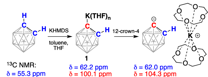
Scheme 2. Deprotonation of ortho - \text{C}_2\text{B}_{10}\text{H}_{12} with potassium hexamethyldisilazide (KHMDs) and subsequent sequestration of the potassium cation by the crown ether. Chemical shifts from the signals in ^{13}\text{C} NMR spectra from the carbon atoms of the parent and deprotonated clusters are listed. Unlabeled cluster vertices represent BH units.
