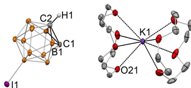
Fig. 3. Displacement ellipsoid plot (50% probability) of [K(12-crown-4) 2 ][C 2 B 10 H 10 I] (4). Note the lack of C...K contact and the complete ion separation. Only a half of the asymmetric unit is shown. Hydrogen atoms on the boron atoms of the cluster and carbon atoms of the crown ether ligand have been omitted for clarity. Selected interatomic distances (Å): K1...C1 = 6.019(3), C1–C2 = 1.677(6), C1–B1 = 1.717(7), C2–B1 = 1.671(8). The analogous distances for another ion pair in the asymmetric unit are K2...C11 = 5.962(5), C11–C12 = 1.674(6), C11–B11 = 1.709(7), C12–B11 = 1.678(7).
