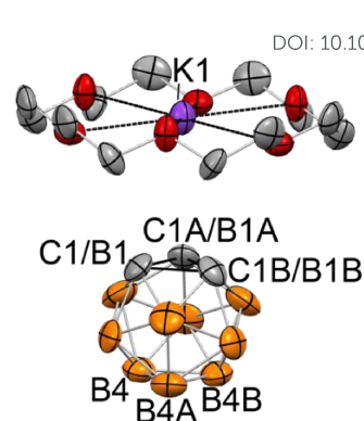
Fig. 1. Displacement ellipsoid plot (50% probability) of [\text{K}(18\text{-crown-6})][\text{C}_2\text{B}_{10}\text{H}_{11}] ( 2 ). Hydrogen atoms have been omitted for clarity. Deprotonated carborane cluster is disordered by the crystal symmetry along its C_3 axis. The closest potassium-cluster contact \text{K1}\cdots\text{C1/B1} is 3.586(1) Å.
