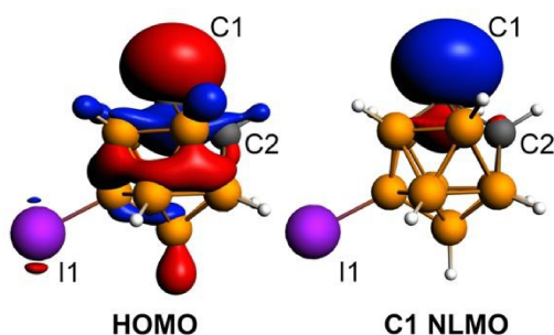
Fig. 4. Plots of the HOMO and the C1 carbon atom lone pair NLMO for the [\text{C}_2\text{B}_{10}\text{H}_{10}]^- anion at the isosurface value of 0.035.
