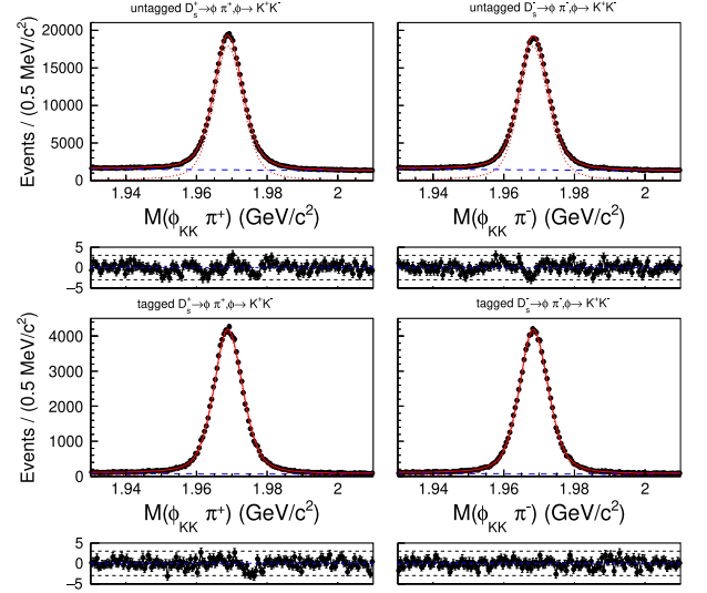
FIG. 3. Data and fit projection for the reference mode D_s^+ \rightarrow \phi \pi^+ . Left side shows D_s^+ candidates, right side shows D_s^- candidates. Upper row is the untagged sample, lower row is the tagged sample. The solid red line is the total fit, the dotted red line is signal, and the dashed blue line is background. The plots beneath the distributions show the residuals.
