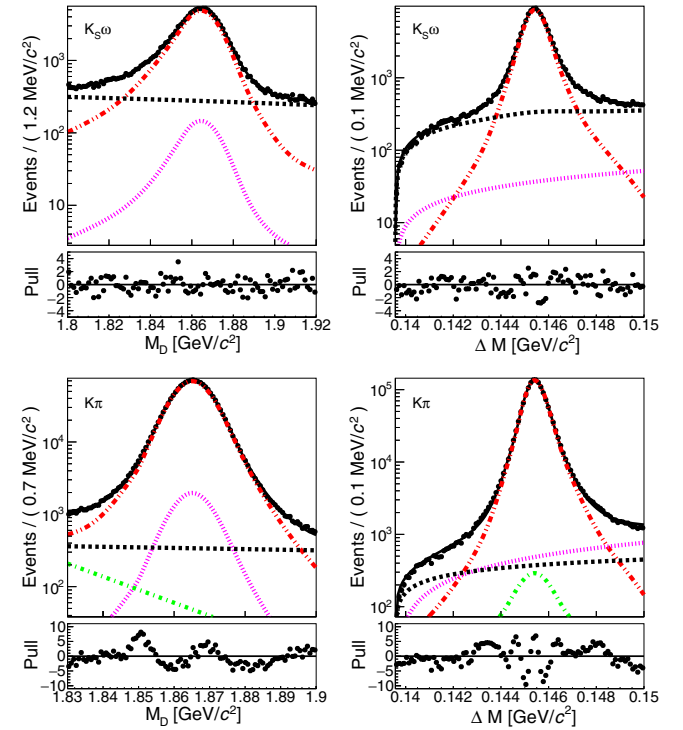
FIG. 1. Projections of the 2D fit on M_D (left) and \Delta M (right) for D^0 \rightarrow K_S^0 \omega (top) and D^0 \rightarrow K^- \pi^+ (bottom). Points with error bars represent the data. The curves show projections of fitted PDF: total PDF projection in solid black, signal contribution in double dot-dashed red, combinatorial background in dashed black, random \pi_{\text{slow}} background in dotted magenta, and multibody background as dash-dotted green. (The total PDF is hard to see as it closely follows the data points.)
