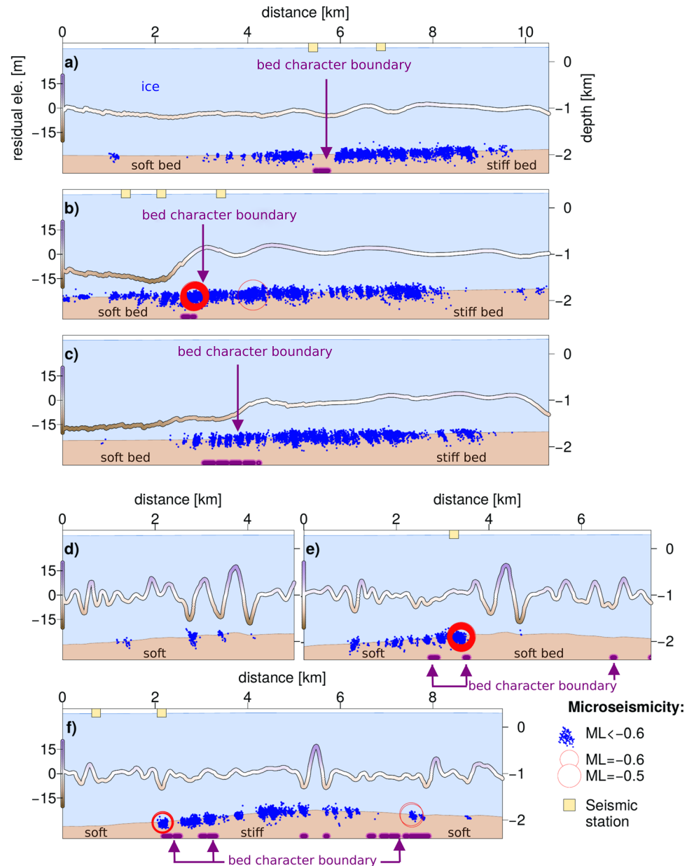
Figure 5. Microseismic event catalog in profile view. (a–c) Flow-parallel and (d–f) flow-perpendicular cross sections. Profile locations are highlighted in Figure 4a. Residual topography is projected onto the profiles for reference. Purple domains at the base of the profiles represent intersection points of the profiles with the bed character boundary.
