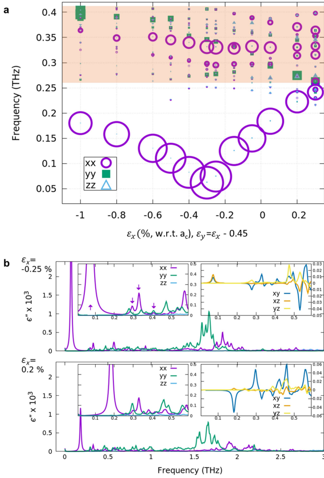
Extended Data Fig. 3 | The dielectric properties of vortex structures as a function of strain and frequency from atomistic calculations.
