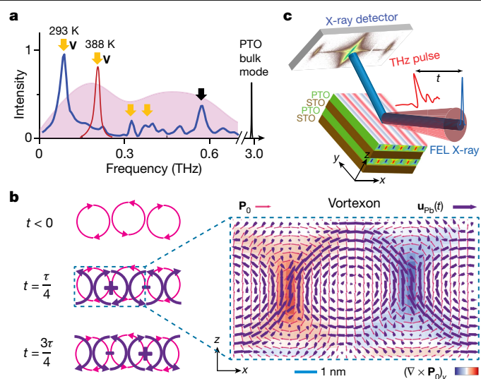
Fig. 1 | Emergence of the collective dynamics of polar vortices and its experimental detection. a , Fourier spectra (blue) of calculated time-dependent response of polar vortices on THz-field excitation. The spectrum of the THz pulse is shown as a broad pink background. The collective modes of polar vortices (orange arrows) are shown as a separate set of modes with respect to the known superlattice acoustic modes (black arrow) and the soft mode of PbTiO 3 at room temperature. The vortexon mode (V) shifts to higher frequency (red peak; note that this is not the calculated peak but a schematic peak to show the temperature dependence) as sample temperature increases. b , Emergence and evolution of the vortexon (atomic displacement vortices, purple circles) during its oscillation period \tau , overlaid with the static polarization vortices (magenta circles). + and –, the signs of vortexon vorticity, which reverse dynamically. Right, zoomed-in view of the region of the dashed box with the calculated static polarization (magenta arrows) and lead-cation displacement (purple arrows) in each unit cell of the vortexon mode at t = \tau/4 . c , Schematic of THz-pump and X-ray-diffraction-probe experiment using an X-ray free-electron laser (FEL). The coloured stripes on the (PbTiO 3 ) 16 /(SrTiO 3 ) 16 (PTO/STO) superlattice film represent in-plane vortex orders with opposite polarization vorticity.
