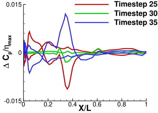
(a) Mode 1
