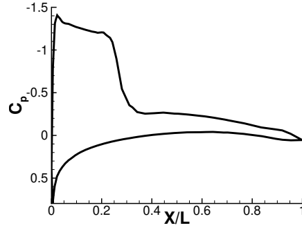
(b) y/b_{\text{semi-span}} = 0.89
