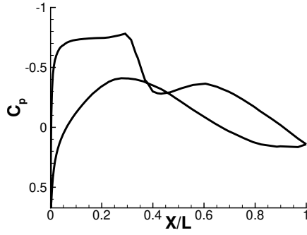
(a) y/b_{\text{semi-span}} = 0.35
