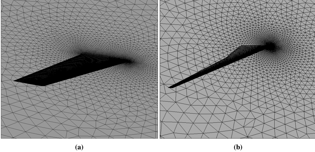
Fig. 3 Aerodynamic surface meshes: (a) AGARD 445.6, and (b) uCRM-13.5
