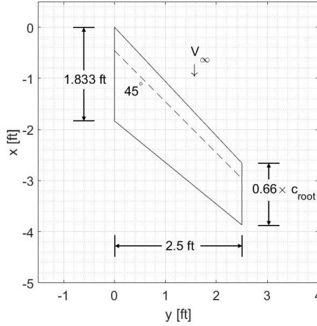
Fig. 4 Planform of the AGARD 445.6 wing
