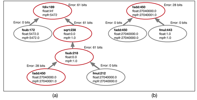
Figure 7: A DAG of instructions generated by PFPSANITIZER while debugging the error in Cholesky. Each node shows the opcode, instruction id, computed value, real value and the numerical error occurred. (a) The DAG for the fddiv instruction that results in infinities ( inf ). (b) The DAG for the fadd instruction that is the root cause of the error.
