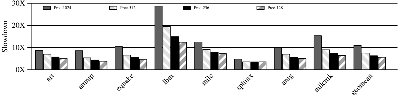
Figure 9: This graph reports the slowdown experienced due to parallel shadow execution with PFPSANITIZER when compared to a baseline without any instrumentation. We report the slowdowns when we vary the number of bits used for the precision in the MPFR data type: 1024 (Prec-1024), 512 (Prec-512), 256 (Prec-256), and 128 (Prec-128) bits of precision.
