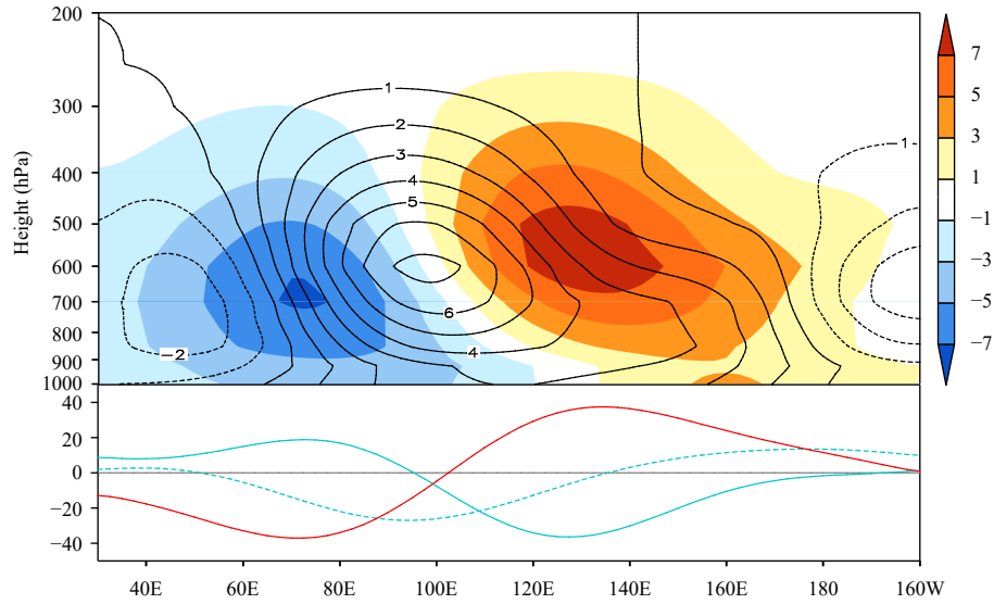
Fig. 2. (Upper panel) Zonal-vertical distributions of 0^{\circ} – 10^{\circ} S averaged MJO-filtered specific humidity (contour, 10^{-4} \text{ kg kg}^{-1} ) and specific humidity tendency (shading, 10^{-10} \text{ kg kg}^{-1} \text{ s}^{-1} ). (Bottom panel) Zonal distributions of 0^{\circ} – 10^{\circ} S averaged MJO-filtered OLR (blue dashed line, \text{W m}^{-2} ), OLR tendency (blue solid line, 10^{-6} \text{ W m}^{-2} \text{ s}^{-1} ), and column-integrated specific humidity tendency (red line, 10^{-7} \text{ kg m}^{-2} \text{ s}^{-1} ) during the active phase of MJO in the eastern Indian Ocean.
