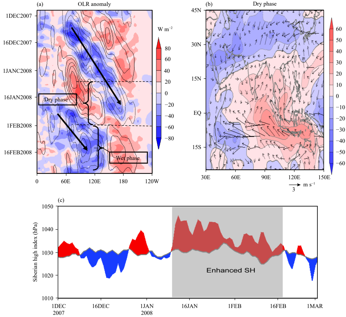
Fig. 13. (a) Hovmöller diagram of 20–70-day filtered OLR anomaly (contour, interval: 20 \text{W m}^{-2} ) averaged over 15°S–5°N. Shading denotes the raw data. (b) Horizontal distribution of the 20–70-day filtered OLR anomaly (shaded) and 925-hPa wind anomaly (vector) fields averaged during the MJO dry phase shown in (a). (c) Time series of the Siberian high index defined as the averaged SLP over 40°–60°N, 80°–120°E. Red (blue) shaded region represents the index higher (lower) than the long-term climatology. From Hong and Li (2009).
