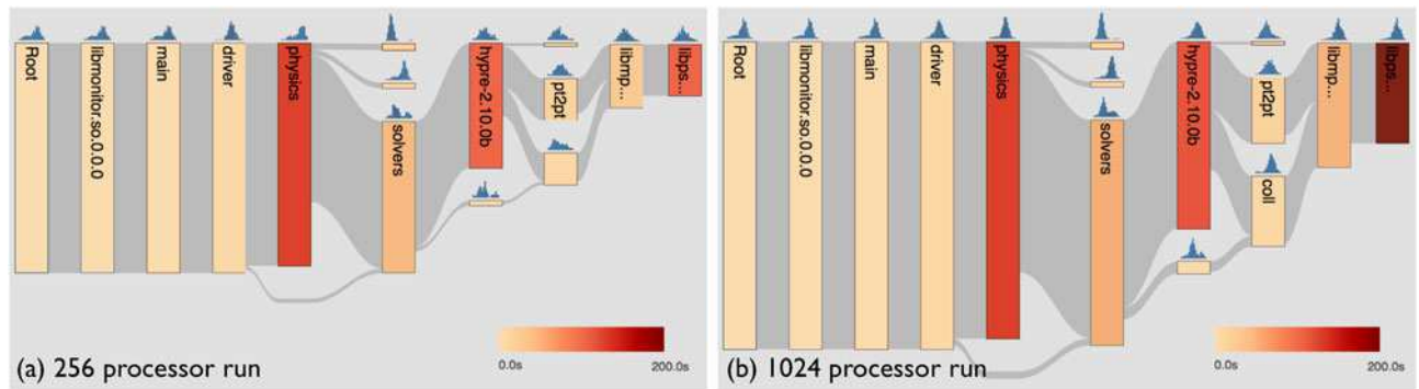
Fig. 10. Comparison of Miranda execution on 256 and 1024 processors; height and color of a bar represent the inclusive and exclusive time spent in the module, respectively. These visualizations help identify the modules in which significant time is spent in the execution, and reveal that the increase in the exclusive time spent in the libpsm module is the primary reason for lower performance on 1024 processors.
