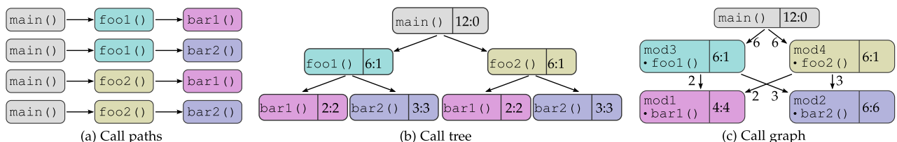
Fig. 2. The call paths (a) call tree (b) and call graph (c) of the example program in Table 1. In (a) each call path shows invocation instances of bar1() and bar2() , rooted at main() . Each node in the corresponding call tree contains three pieces of information: node name, inclusive metric, and exclusive metric (denoted as inclusive : exclusive). Since the call graph is constructed from the call tree, the original inclusive cost information can be retained through edge weights.
