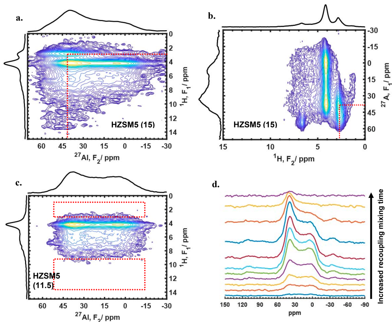
Figure 4. (a) ^{27}\text{Al}\{^1\text{H}\} and (b) ^1\text{H}\{^{27}\text{Al}\} two-dimensional D-HMQC data for dehydrated Si/Al = 15 H-ZSM-5 acquired at 19.6 T. (c) ^{27}\text{Al}\{^1\text{H}\} D-HMQC data for dehydrated Si/Al = 11.5. (d) Example ^{27}\text{Al} slices at the 4.2 ppm ^1\text{H} chemical shift as a function of dipolar mixing time for the Si/Al = 15 catalyst similar to that shown in part a. An example correlation for the ^{27}\text{Al} and ^1\text{H} shifts with maxima at 38 and 2.8 ppm, respectively, is highlighted by the dashed red lines in parts a and b. Note the absence of Al/H correlations in part c that were present in part a, as indicated by the boxed areas.
