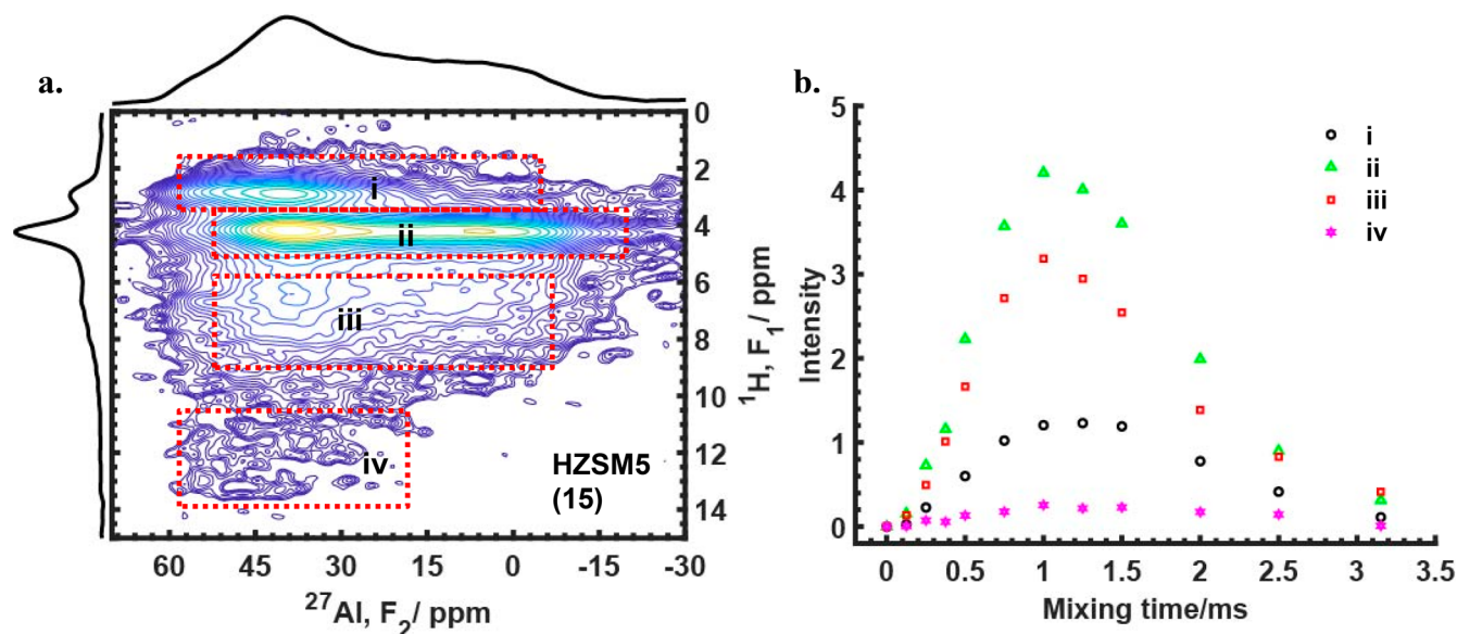
Figure 5. (a) Regions in the ^{27}\text{Al}\{^1\text{H}\} two-dimensional D-HMQC data used for quantitative analysis of Al–H internuclear distances by extracting ^{27}\text{Al} slices to get data of the type shown in (b) for four different ^1\text{H} chemical shifts denoted by the boxed regions. In part b, intensities are plotted in absolute units, while the companion Figure S6 shows the same data normalized to the maximum intensity for each curve to facilitate comparison between all species.
