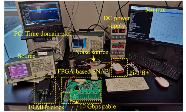
Fig. 2. Pulsar signal acquisition platform based on FPGA.
