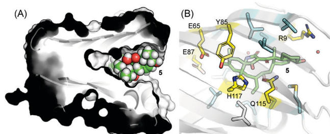
Figure 2. Cocrystal structure of PyrI4-product: (A) shown in surface-filling model and (B) enlarged view of the binding pocket shown in stick model with hydrophilic residues colored in yellow and hydrophobic residues colored in cyan.
