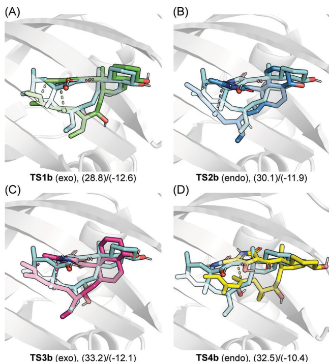
Figure 7. Docked pose of different stereoisomeric transition states overlaid with the XRD structure of the product (S, cyan colored) in complexation with PyrI4. First numbers in brackets are the DFT-calculated transition state energies at the M06-2X/6-311++G(d,p)/CPCM(ether)//M06-2X/6-31G(d,p)/CPCM(ether) level in the absence of enzyme. Second numbers in brackets are the binding energies predicted by AutoDock Vina. All numbers are in kcal/mol.
