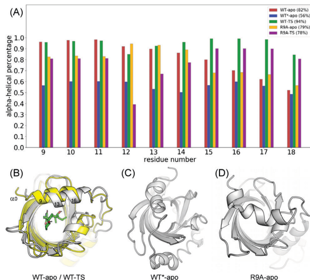
Figure 8. Study of the kinetic stability of \alpha 0-helix by helical content analysis. (A) \alpha -Helical content of key residues of \alpha 0 of different species. (B) Overlaid representative snapshots of WT-apo (gray) and WT-TS (yellow) in MD simulations. (C and D) Representative snapshots of the MD simulations of WT-apo performed at 100 °C and apo-R9A mutant. Percentage number in brackets after each species is the averaged \alpha -helical percentage over the 1 \mu s MD simulation.
