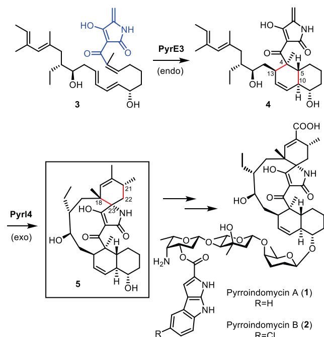
Scheme 1. Biosynthesis of Pyrroindomycin A (1) and B (2) Involves Two Key Diels–Alders
