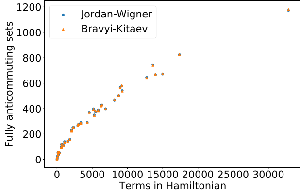
FIG. 1. Number of fully anticommuting sets for electronic structure Hamiltonians vs the number of terms in the full Pauli Hamiltonian using the greedy independent sets strategy. The number of fully anticommuting sets is at least an order of magnitude less than the number of terms. The Jordan-Wigner and Bravyi-Kitaev mappings perform almost equivalently.
