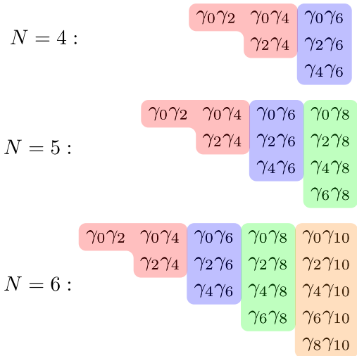
FIG. 4. Partitioning of electronic structure terms. Finding an anticommuting partition of the quartic terms can be reduced to finding an anticommuting partition of quadratic terms with exclusively even (equiv. odd) indices. Each highlighted bin is such an anticommuting set. Excluding the red bin, each set shares one common index 2q for 3 \leq q \leq N-1 . Although only three values of N are depicted, the induction of this diagram is straightforward for arbitrary N . One thus obtains N-3 bins of size q each and 1 “red bin” of size 3.
