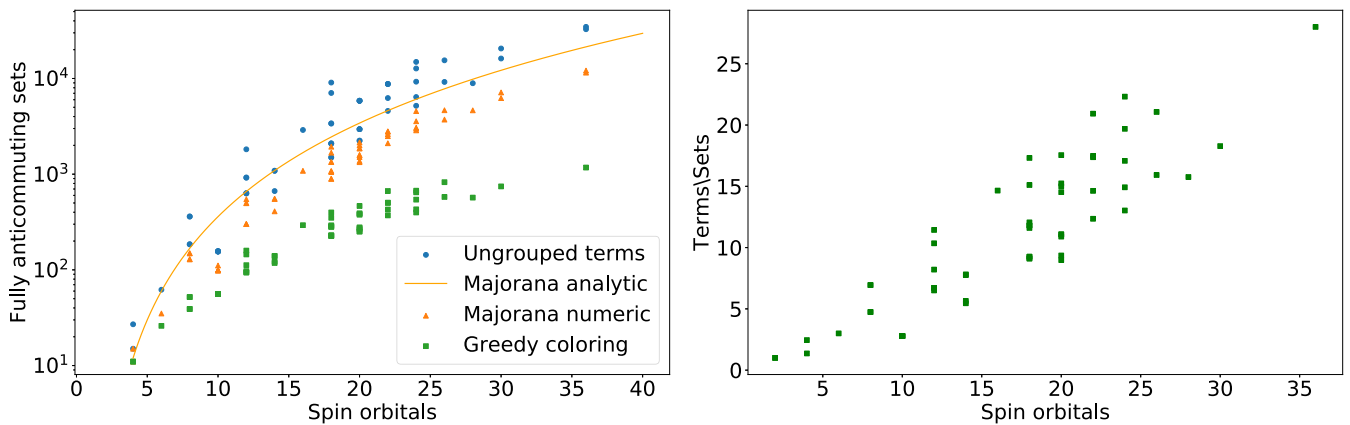
FIG. 2. Number of fully anticommuting sets for electronic structure Hamiltonians vs the number of spin orbitals using the Jordan-Wigner mapping. Left: Including all partitioning schemes. The “Majorana analytic” curve is the \binom{N}{2}(N-2) upper bound obtained from (1) for generic Hamiltonians of Eq. (67). The “Majorana numeric” data points correspond to the partitions described in Sec. IV B without further optimization. This upper bound is loose due to sparsity in the molecular Hamiltonians vs the set of all possible terms. Right: Ratio of the number of terms to the number of anticommuting sets for systems with more than five spin orbitals. A roughly linear trend is observed, in agreement with the analytic scaling discussed in Sec. IV B.
