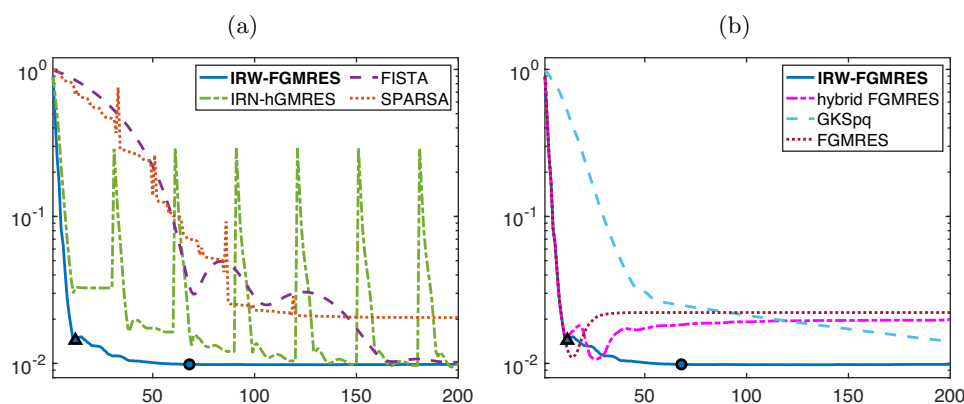
FIG. 2. Experiment 1. History of relative error norms (i.e., \|x_k(\lambda) - x_{true}\|_2 / \|x_{true}\|_2 against iteration number k ) for the new IRW-FGMRES, compared to (a) other standard solvers for the \ell_2 - \ell_1 problem, (b) other flexible and generalized Krylov-based solvers. The circle and triangle markers correspond to stopping criteria (4.4) based on the stabilization of \lambda and s(x_k) , respectively.
