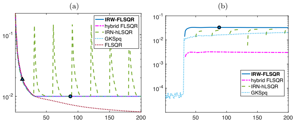
FIG. 8. Experiment 2. Methods based on Krylov subspaces. (a) History of the relative residuals. (b) History of the regularization parameters. The circle and triangle markers correspond to stopping criteria (4.4) based on the stabilization of \lambda and s(x_k) , respectively.
