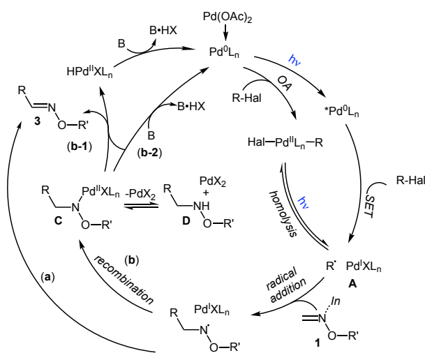
Scheme 5. Proposed Mechanism
