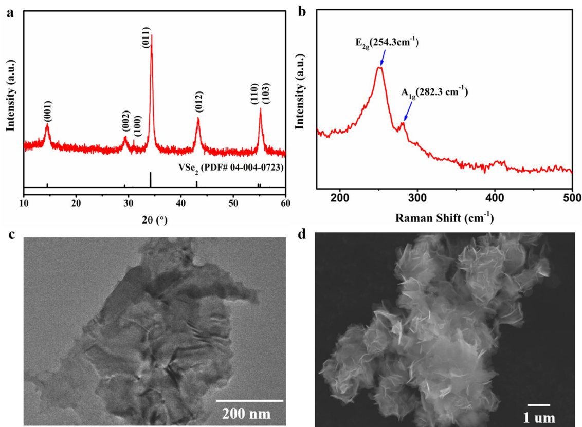
Figure 1. Characterization of the synthesized VSe 2 NSs. (a) X-ray diffraction. (b) Raman spectrum. (c) TEM image of a nanosheet. (d) SEM image of a nanosheet agglomerate.
