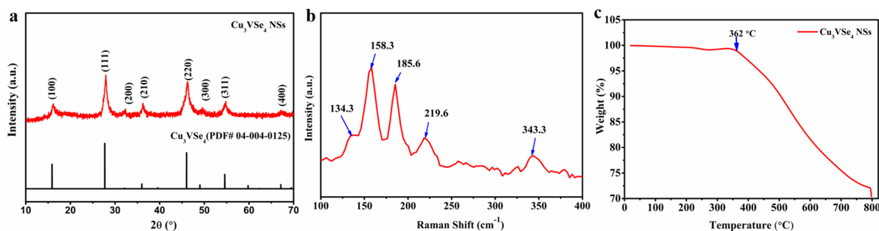
Figure 2. Characterization of Cu 3 VSe 4 NSs. (a) XRD pattern. (b) Raman spectrum. (c) TGA plot.
