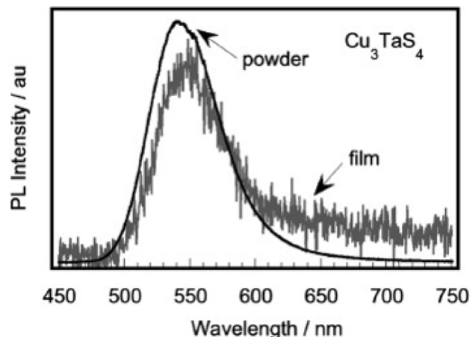
Figure 3. Photoluminescence spectra for \text{Cu}_3\text{TaS}_4 powder and thin film. Reprinted with permission from ref. [7], Copyright 2008 Elsevier B.V.
