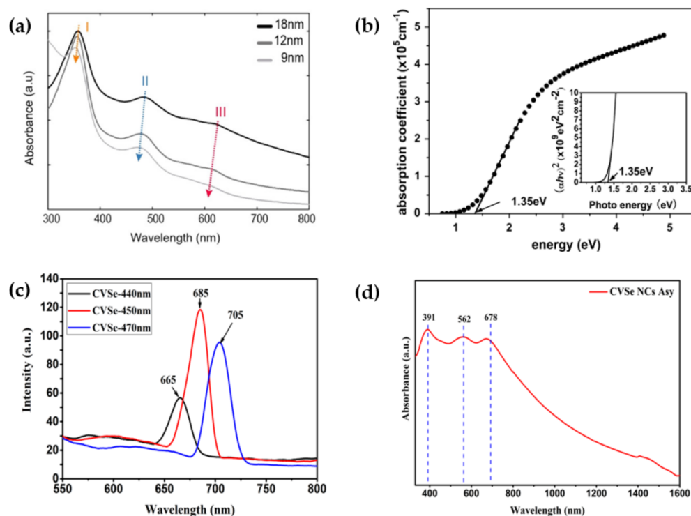
Figure 4. (a) UV-visible absorption spectra of \text{Cu}_3\text{VS}_4 nanocrystals of differing sizes. Reprinted with permission from ref. [12], Copyright 2019 American Chemical Society. (b) Absorption coefficient \alpha versus the photon energy of \text{Cu}_3\text{VS}_4 nano-thin films. Reprinted with permission from ref. [4], Copyright 2012 Elsevier B.V. (c) Photoluminescence of \text{Cu}_3\text{VSe}_4 nanocrystals at different excitation wavelengths (440, 450, and 470 nm). Reprinted with permission from ref. [9], Copyright 2020 Liu et al. (d) Uv-Vis-NIR spectra of \text{Cu}_3\text{VSe}_4 nanocrystals in ethanol. Reprinted with permission from ref. [9], Copyright 2020 Liu et al.
