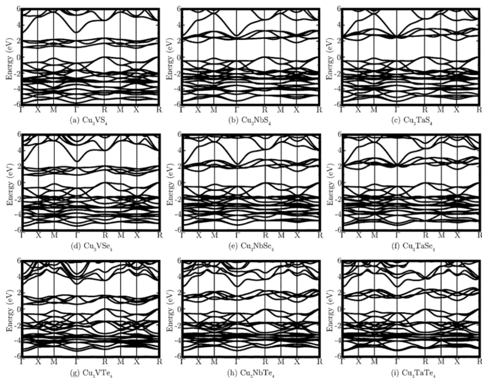
Figure 2. Electronic band structure of the sulvanite family of compounds calculated using \text{PbEsol} + \text{U} . The valence band maximum is taken to be zero. Reprinted with permission from [5], Copyright © 2015 Royal Society of Chemistry (RSC).
