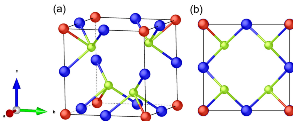
Figure 1. (a) The unit cell of \text{Cu}_3\text{MX}_4 . (b) The unit cell of \text{Cu}_3\text{MX}_4 , as seen from \langle 100 \rangle direction. (Red is attributed to M transition metal ion, blue represents Cu ions, light green is attributed to chalcogen ions.)
