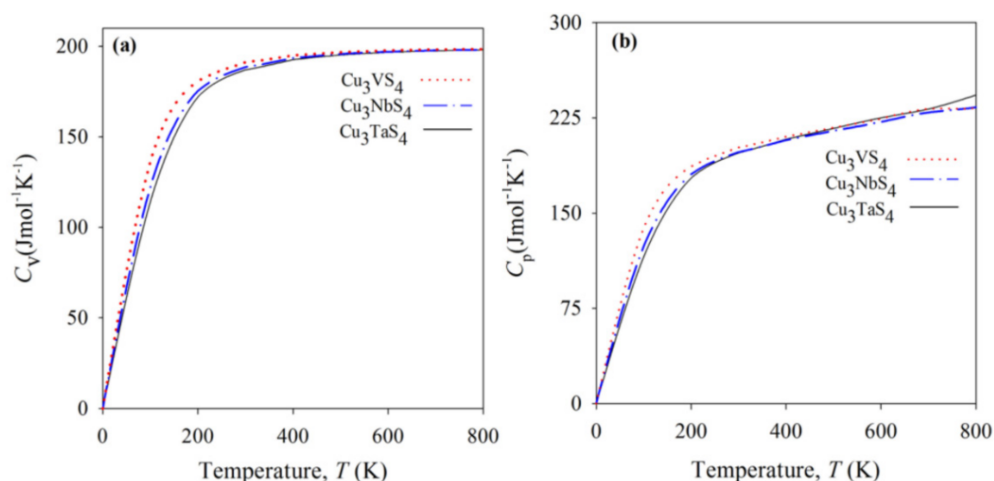
Figure 6. Heat capacities (a) at constant volume C_V and (b) at constant pressure C_P of the compounds \text{Cu}_3\text{MS}_4 ( M = \text{V}, \text{Nb}, \text{Ta} ). Reprinted with permission from ref. [27], Copyright 2014 JSR Publications, obtained 20 January 2021.
