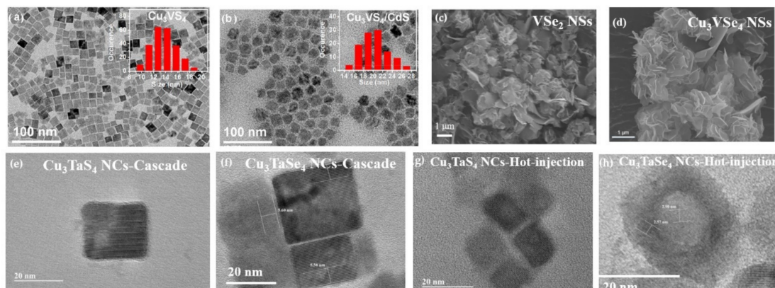
Figure 7. (a) TEM image of \text{Cu}_3\text{VS}_4 nanocrystals with size distribution inset. Reprinted with permission from ref. [12], Copyright 2019 American Chemical Society. (b) CVS/CdS nanocrystals with size distribution inset. Reprinted with permission from ref. [24], Copyright 2020 American Chemical Society. (c) \text{VSe}_2 nanosheet precursor as starting material. Reprinted with permission from ref. [8], Copyright 2020 Liu et al. (d) \text{Cu}_3\text{VSe}_4 nanosheets end product. Reprinted with permission from ref. [8], Copyright 2020 Liu et al. (e) TEM image of \text{Cu}_3\text{TaS}_4 prepared by Cascade method. Reprinted with permission from ref. [10], under Creative Commons CC BY license. (f) TEM image of \text{Cu}_3\text{TaSe}_4 prepared by Cascade method. Reprinted with permission from ref. [10], under Creative Commons CC BY license. (g) TEM image of \text{Cu}_3\text{TaS}_4 prepared by hot injection. Reprinted with permission from ref. [10], under Creative Commons CC BY license. (h) TEM image of \text{Cu}_3\text{TaSe}_4 prepared by hot injection. Reprinted with permission from ref. [10], under Creative Commons CC BY license.
