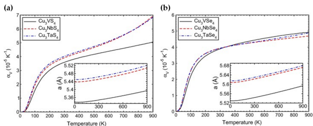
Figure 5. Calculated volume thermal expansion coefficient \alpha_V versus temperature T within the quasi-harmonic approximation for the compounds \text{Cu}_3\text{MX}_4 ( M = \text{V}, \text{Nb}, \text{Ta} ; X = \text{S}, \text{Se} ). (Inset) Cell parameter versus temperature. (a) Results for the sulfide compounds \text{Cu}_3\text{MS}_4 . (b) Results for the selenide compounds \text{Cu}_3\text{MSe}_4 . Reprinted with permission from ref. [65], Copyright 2015 Elsevier B.V.
