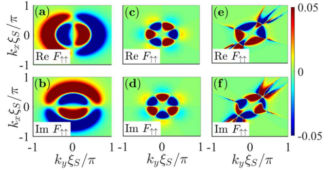
FIG. 5. Real and imaginary parts of equal-spin superconducting correlations in k space; \xi_S = \hbar/\sqrt{2m^*}\Delta is the characteristic length. (a), (b) Linear Rashba, \alpha = 1 . (c), (d) cSOC, \alpha_c = 1, \beta_c = 0 . (e), (f) cSOC, \alpha_c = \beta_c = 1 . The other parameters are the same for all panels.
