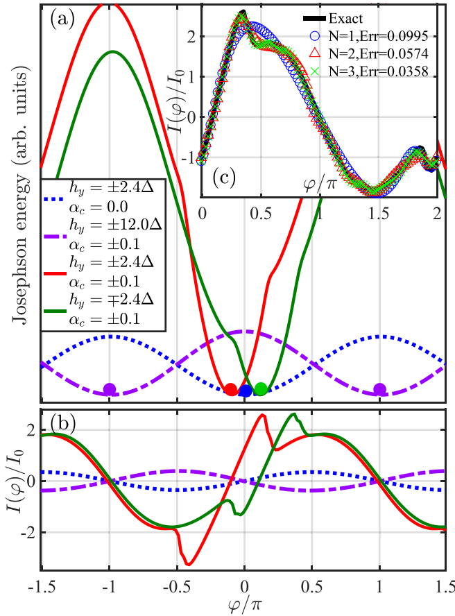
FIG. 3. (a) Josephson energy and (b) related supercurrent evolution with the superconducting phase difference \phi Zeeman field, h_y , at a fixed magnitude and varying Rashba cSOC strength \alpha_c are considered. The other parameters are \beta_c = 0 , \mu = \Delta , h_x = 0 . (c) Three fits to the green curve in (b) using the generalized CPR from Eq. (4) with N = 1, 2, 3 harmonics.
