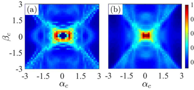
FIG. 4. Normalized critical supercurrent as a function of cSOC strength \alpha_c and \beta_c for (a) \mu = \Delta and (b) \mu = 10\Delta . The Zeeman field is set to zero.
