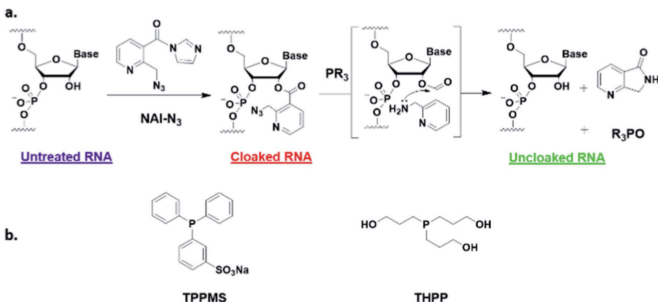
Fig. 1 (a) Mechanism of RNA cloaking using NAI- N_3 and Staudinger uncloaking by a soluble phosphine. (b) Structures of phosphines used in this study.
