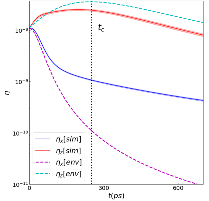
FIG. 8. Comparison of the evolution of the parameter \eta between the envelope equations (dashed lines) and the N -particle simulations (solid lines). The line and shaded area around the N -particle simulation lines represent the mean (solid line) \pm the standard deviation of 90 simulations. The vertical dotted line indicates the focal point. Notice that the emittance-conserving model overpredicts \eta_z and underpredicts \eta_x . This is partially due to the heat being transferred between the dimensional modes, a mechanism that is not captured by the emittance-conserving envelope equations.
