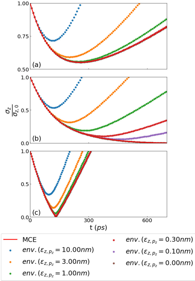
FIG. 3. Longitudinal width evolution, \sigma_z , divided by the initial longitudinal width, \sigma_{z,0} , of prolate ellipsoids with ( \alpha_0 = 10/75 ) focused by different initial chirps: (a) 0.7 v_{z,c}^* , (b) 1.0 v_{z,c}^* , (c) 1.5 v_{z,c}^* . In each figure, the red solid line represents the prediction from the MCE model, and the dotted lines represent the envelope equations with different emittance ranging from 0 to 10 nm. Notice that the envelope equations with zero emittance and the MCE model are in perfect agreement. Also notice that (1) increasing the emittance makes the waist larger and moves it earlier and (2) the evolution of the width statistic is more responsive to emittance when the chirp is in the vicinity of the critical chirp.
