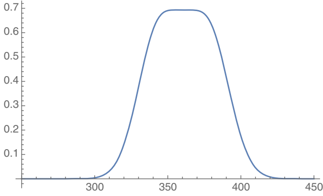
FIG. 8. Plot of H_s^{(q=1)} as a function of s for n = 1000 and R = 0.75 .
