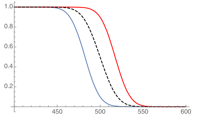
FIG. 9. Plots of \tilde{\lambda}^+ (red to the right), \tilde{\lambda}^- (blue to the left) as functions of s for n = 1000 and R = 1 , compared to \lambda^0 (dashed, center).
