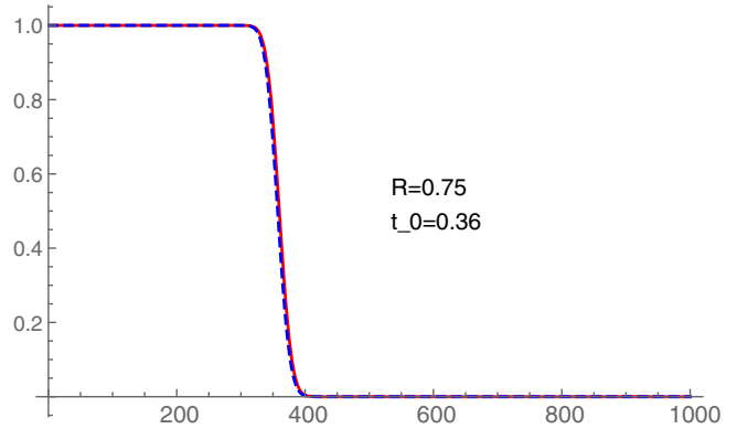
FIG. 2. Plots of \lambda_s as a function of s for k=1 (red), k=5 (blue dashed) and n=1000 and R=0.75 .
