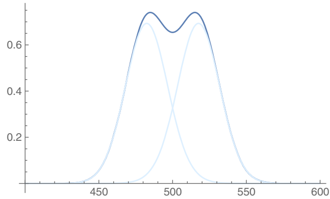
FIG. 12. Plot of \tilde{H}^+ + \tilde{H}^- as function of s for n = 1000 and R = 1 .
