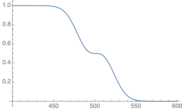
FIG. 5. Plot of \lambda_s^{(q=1)} as a function of s for k = 1, n = 1000 and R = 1 .
