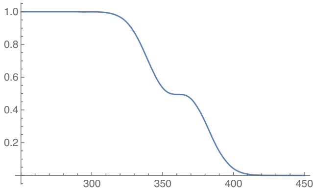
FIG. 6. Plot of \lambda_s^{(q=1)} as a function of s for k = 1, n = 1000 and R = 0.75 .
