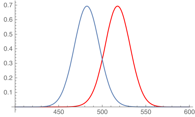
FIG. 11. Plots of \tilde{H}^+ (red to the right) and \tilde{H}^- (blue to the left) as functions of s for n = 1000 and R = 1 .
