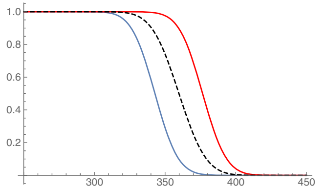
FIG. 10. Plots of \tilde{\lambda}^+ (red to the right), \tilde{\lambda}^- (blue to the left) as functions of s for n = 1000 and R = 0.75 , compared to \lambda^0 (dashed, center).
