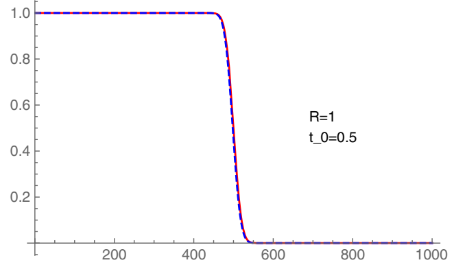
FIG. 1. Plots of \lambda_s as a function of s for k=1 (red), k=5 (blue dashed) and n=1000 and R=1 .
