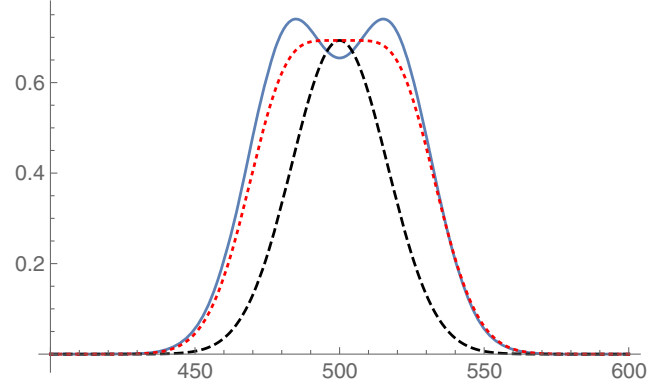
FIG. 13. Plots of H^{(\nu=1)} (black, dashed), H^{(q=1)} (red, dotted) and H^{(\nu=2)} (blue, solid) as functions of s for n = 1000 and R = 1 .
