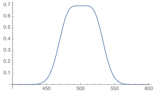
FIG. 7. Plot of H_s^{(q=1)} as a function of s for n = 1000 and R = 1 .
