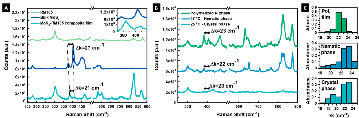
Figure 3. (A) Raman spectra of a solution cast film of MoS 2 -RM105, bulk MoS 2 , and RM105. (B) Raman spectra of different phases of the MoS 2 -RM105 composite: crystal, nematic, and polymerized film. (C) Distribution of frequency differences between the E 2g 1 and A 1g Raman modes of MoS 2 in the different phases.
