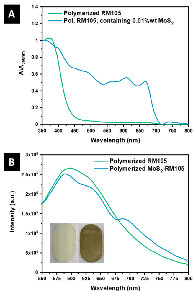
Figure 4. (A) Normalized absorption spectra of polymerized RM105 films, excluding and containing MoS 2 . (B) PL spectra of the same MoS 2 -RM105 films measured in part A. Inset: picture of the polymerized films.
