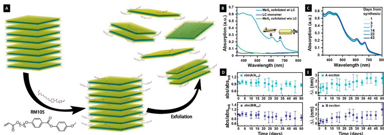
Figure 1. (A) Schematic illustration of MoS 2 exfoliation using thermotropic LCs. (B) Optical extinction spectra of MoS 2 suspensions produced with different exfoliation conditions. (C) Optical extinction spectra of the mesogen-containing-2D-MoS 2 suspension over time. (D) Relative intensity and (E) spectral shift at the A and B excitonic transition peaks over time.
