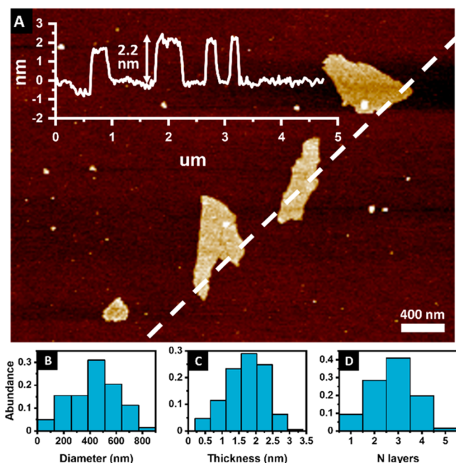
Figure 2. (A) AFM height image and profile of 2D-MoS 2 sheets drop-cast from solution. Distribution of exfoliated sheets' (B) size, (C) thickness, and (D) estimated number of layers.
