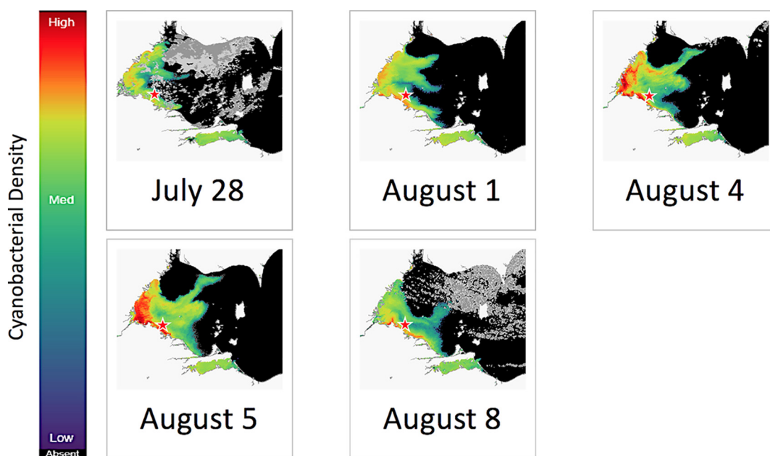
FIG 1 Satellite-derived cyanobacterial index images of the western Lake Erie cHAB 28 July to 8 August 2019. The star indicates the location of the Toledo water intake crib (41.7000436 N, –83.250217 W). Peak biomass of the bloom for the 2019 season occurred on 5 August 2019. The images were derived from Copernicus Sentinel-3 satellite data from the European Organization for the Exploitation of Meteorological Satellites (EUMETSAT) and processed to convert lake color to cHAB abundance by Richard Stumpf, NOAA, National Centers for Coastal Ocean Science.
