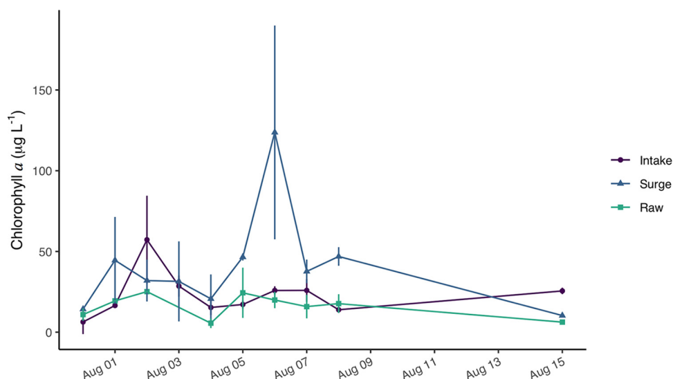
FIG 3 Chl a biomass in the intake, surge well, and WTP raw water. The concentrations measured at the intake valve represent the algal community that is pulled into the water treatment plant from Lake Erie. The surge well concentrations are most variable, likely owing to the retention of algal communities in the well. Concentrations are lowest in WTP raw water, as this water is posttreatment with low doses of the algaecide potassium permanganate and the addition of activated carbon.
