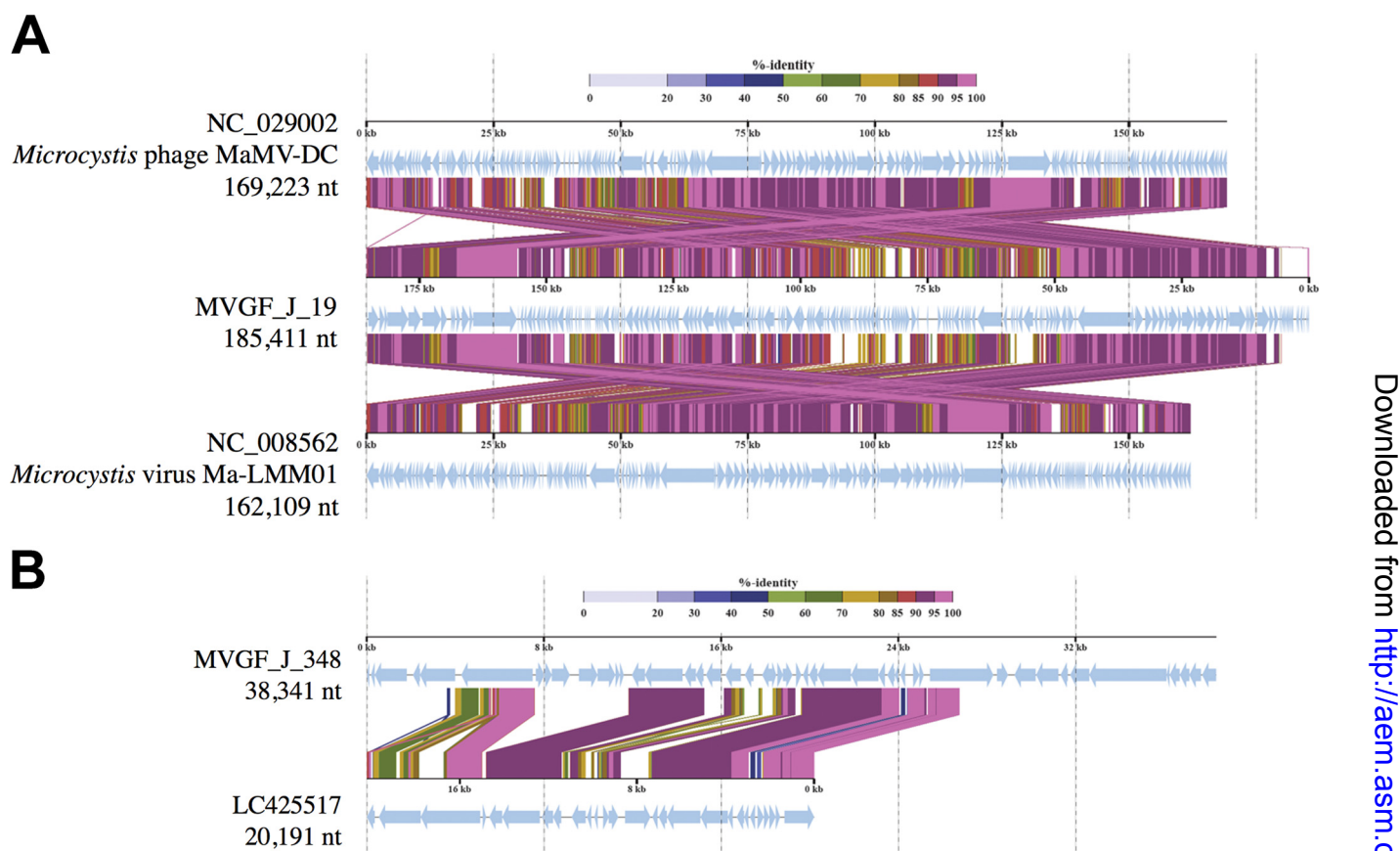
FIG 7 Proteomic similarity between closely related Microcystis viral genomic fragments (MVGFs). (A) The relationship between MVGF_J_19 and two isolated and characterized Microcystis cyanophages, Ma-LMM01 and MaMV-DC. The genetic rearrangement but high protein percent identity suggest MVGF_J_19 to be a Lake Erie variant of these two isolates. (B) Sequence similarity between MVGF_J_348 and Morimoto et al. (23) siphovirus MVGF LC425517 (NODE382).
